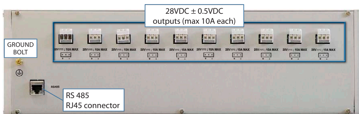
Active Subrack - rear view
