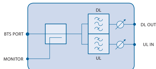
Duplex TAPOI - Block diagram
