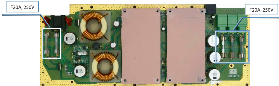
Very High Power and Pole mounting Remote Units: DC/DC Power Supply Module protection fuses position and electrical rating
