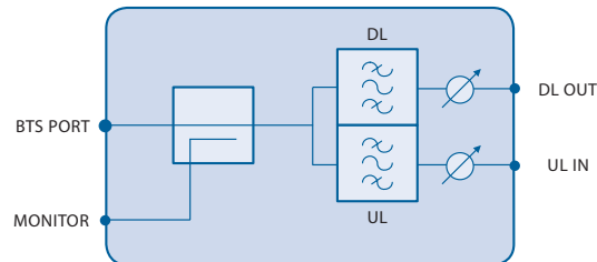
Point Of Interface module block diagram
