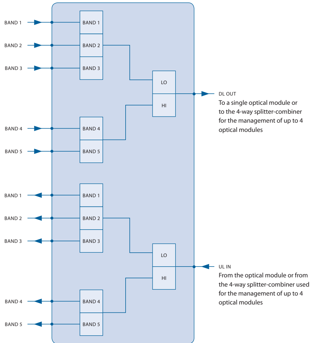
Example: 3-Low-band- + 2-High-Band Pentaplexer block diagram
