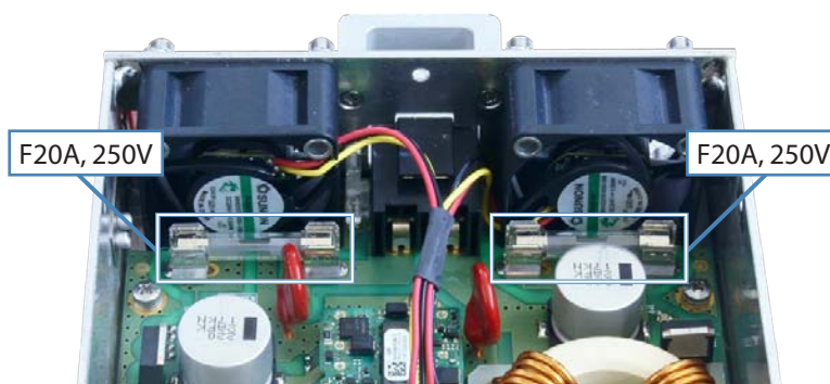
DC/DC Power Supply module (TPSU/48-30-1K) input protection fuses - position and electrical rating
