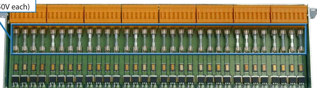
Output port protection fuses - position and electrical rating
