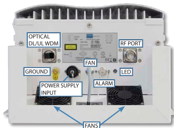
Dual band/Triband high power Remote Units Bottom view
