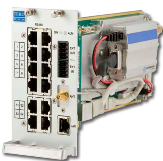
Supervision Module equipped with optional built-in wireless modem
