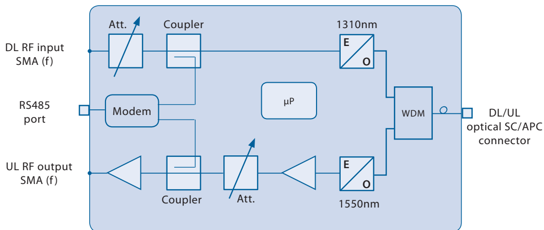
Master Point to Point Module block diagram
