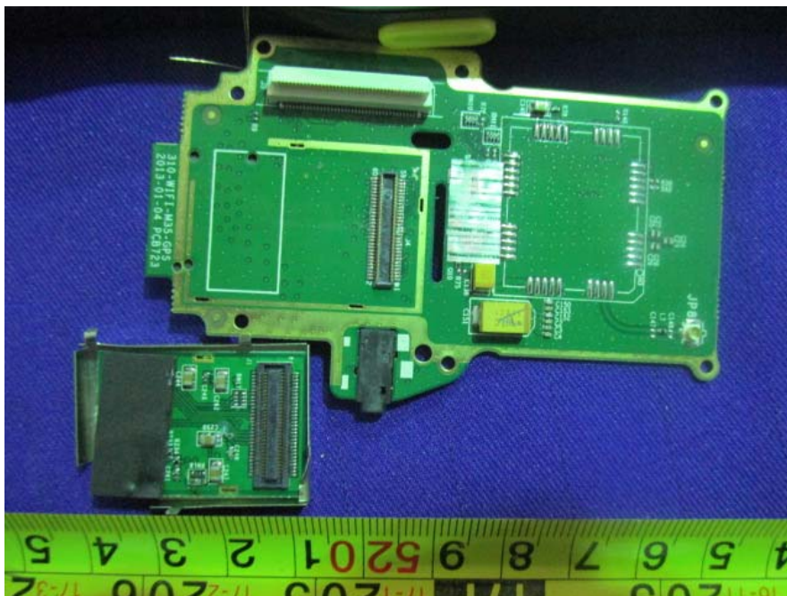
EUT – Sub Board 1 Bottom without Shielding View
