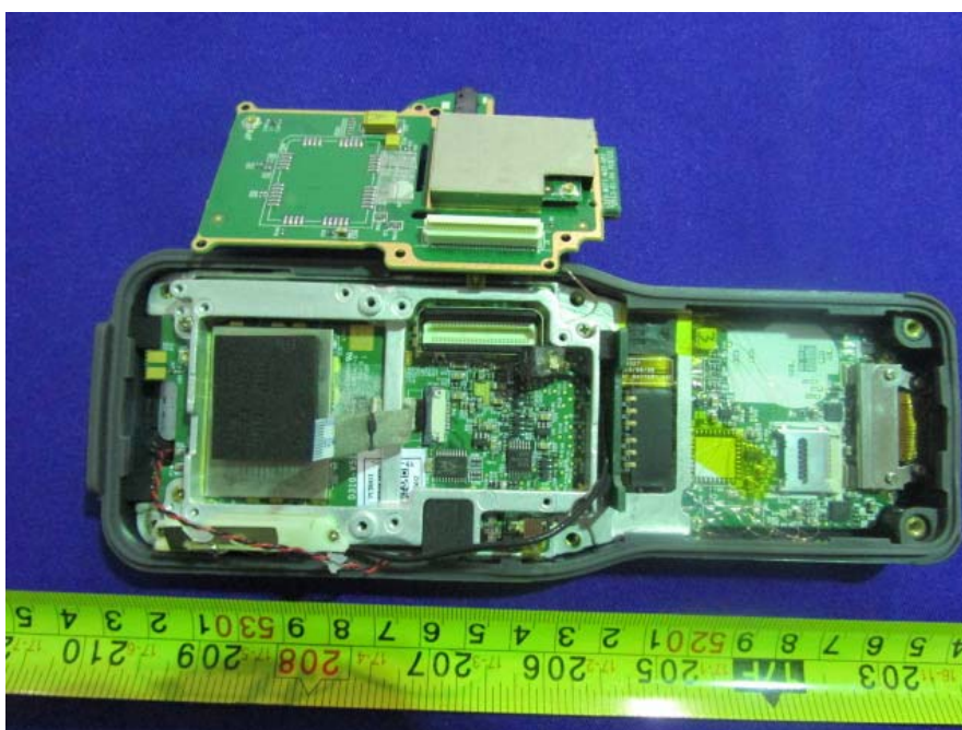
EUT – PCB Uncover View
