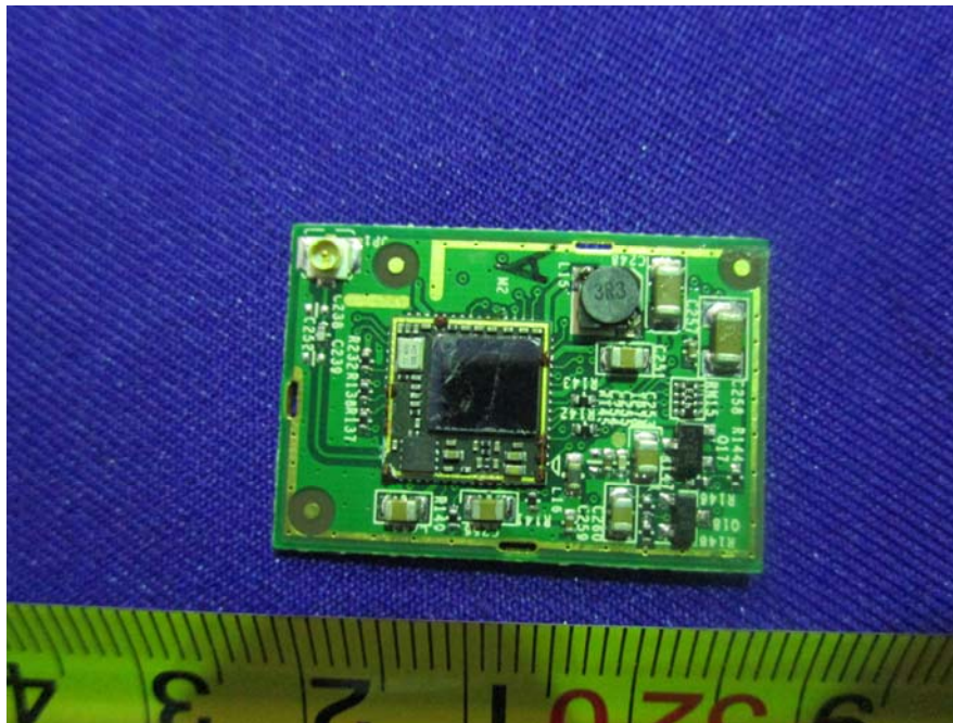
EUT – RF Module Top without Shielding View
