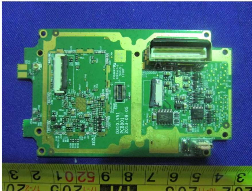
EUT – Sub Board 2 Top without Shielding View
