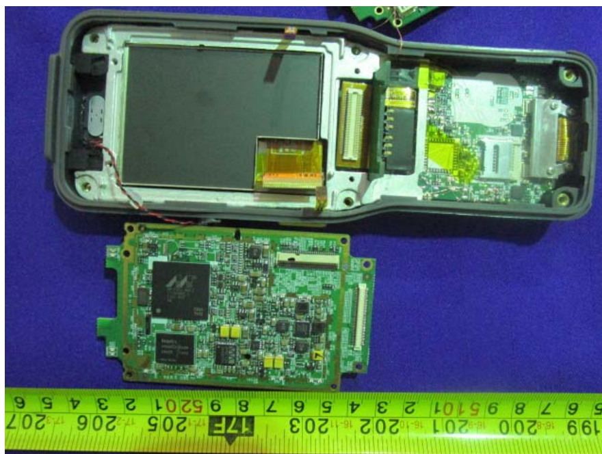
EUT – Sub Board 2 Off View
