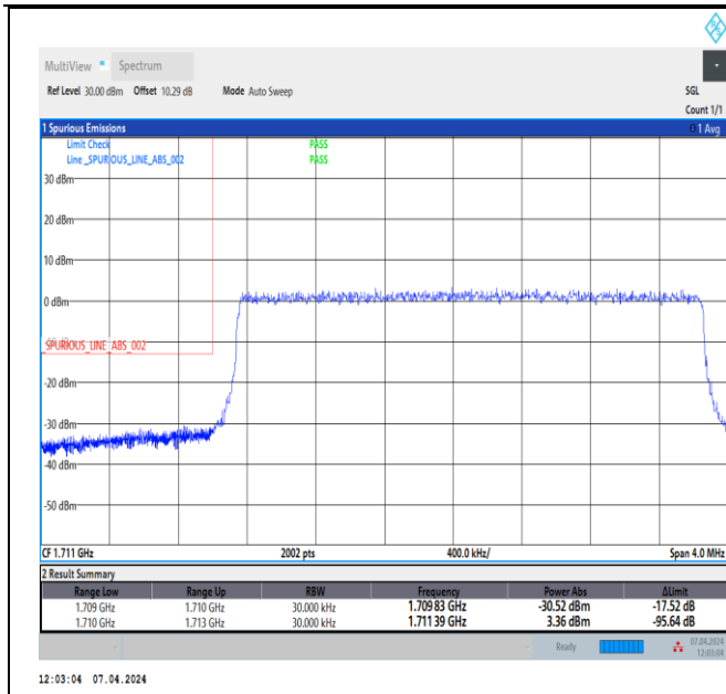
Band4_3MHz_64QAM_19965_15RB#0
