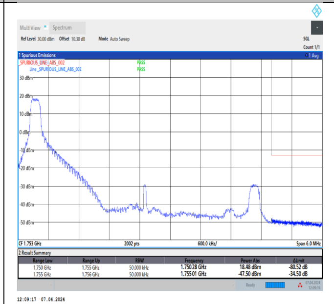
Band4_5MHz_QPSK_20375_1RB#0
