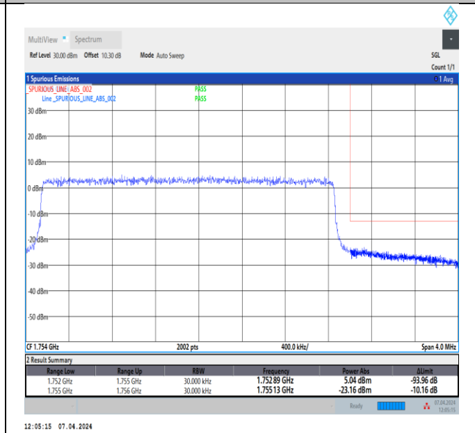
Band4_3MHz_QPSK_20385_15RB#0
