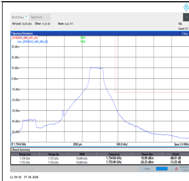
Band4_1.4MHz_64QAM_20393_1RB#5
