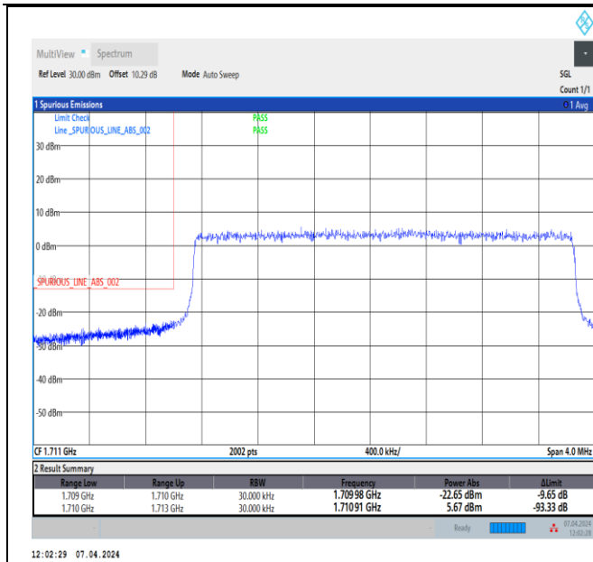
Band4_3MHz_QPSK_19965_15RB#0
