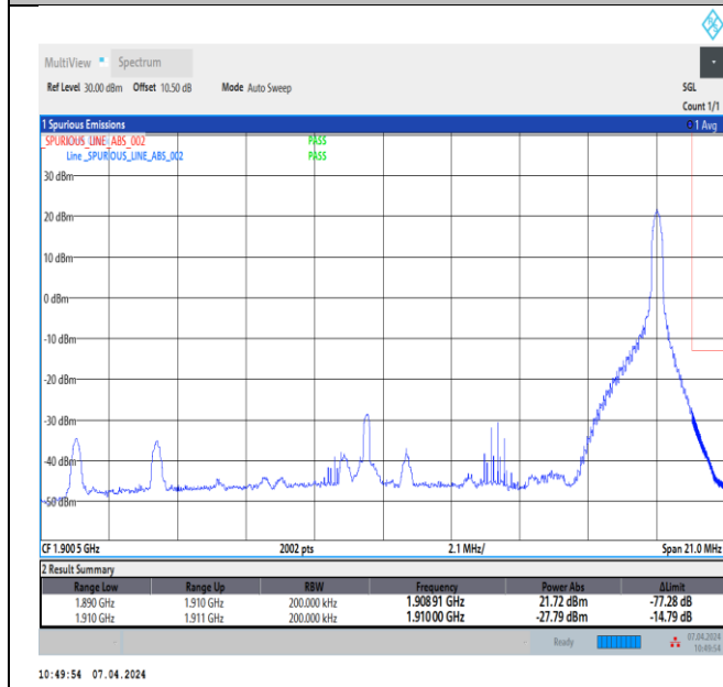
Band2_20MHz_64QAM_19100_1RB#99
