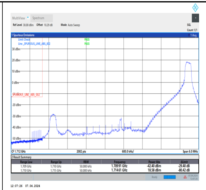
Band4_5MHz_QPSK_19975_1RB#24
