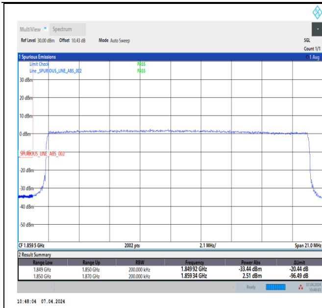
Band2_20MHz_64QAM_18700_100RB#0
