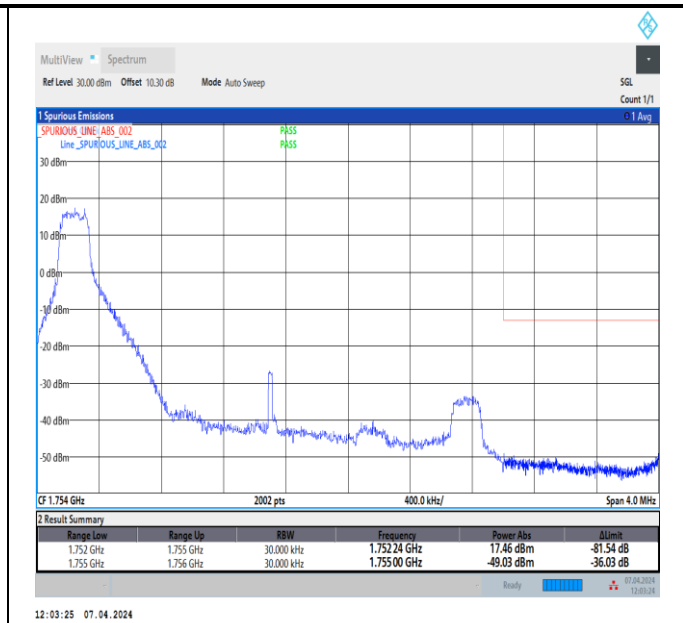
Band4_3MHz_QPSK_20385_1RB#0
