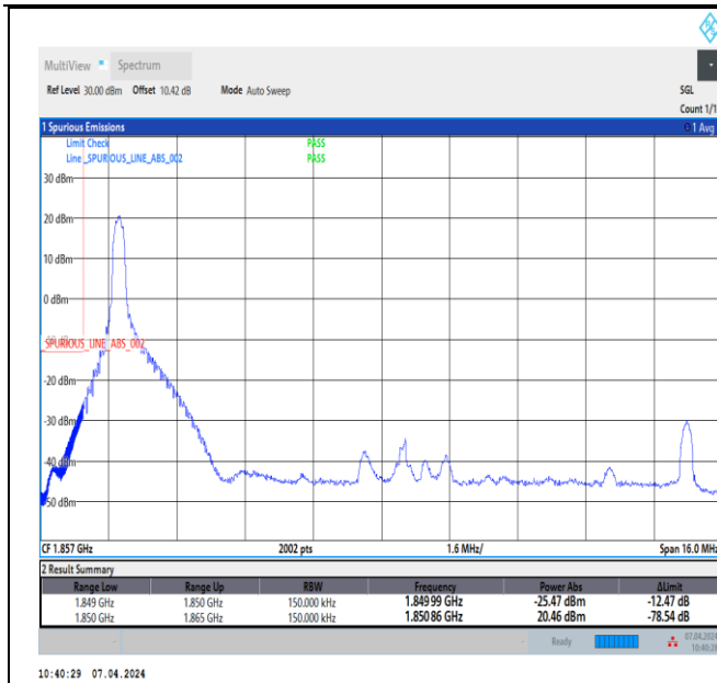
Band2_15MHz_64QAM_18675_1RB#0
