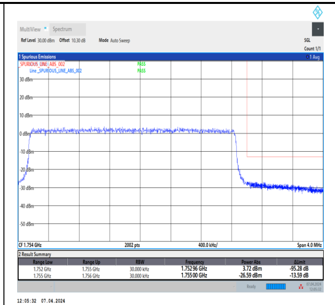
Band4_3MHz_16QAM_20385_15RB#0
