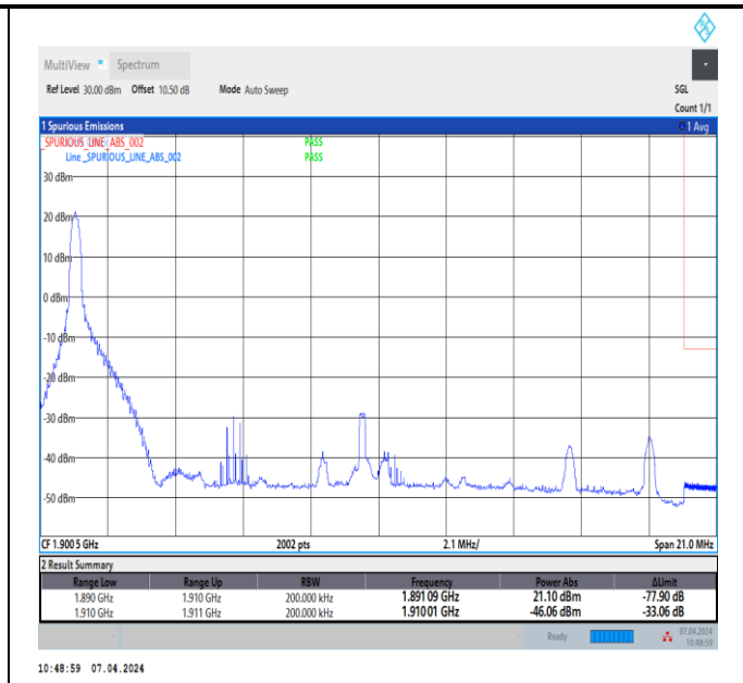
Band2_20MHz_64QAM_19100_1RB#0
