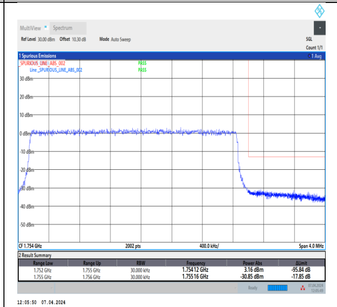
Band4_3MHz_64QAM_20385_15RB#0
