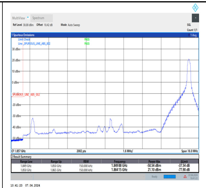
Band2_15MHz_64QAM_18675_1RB#74
