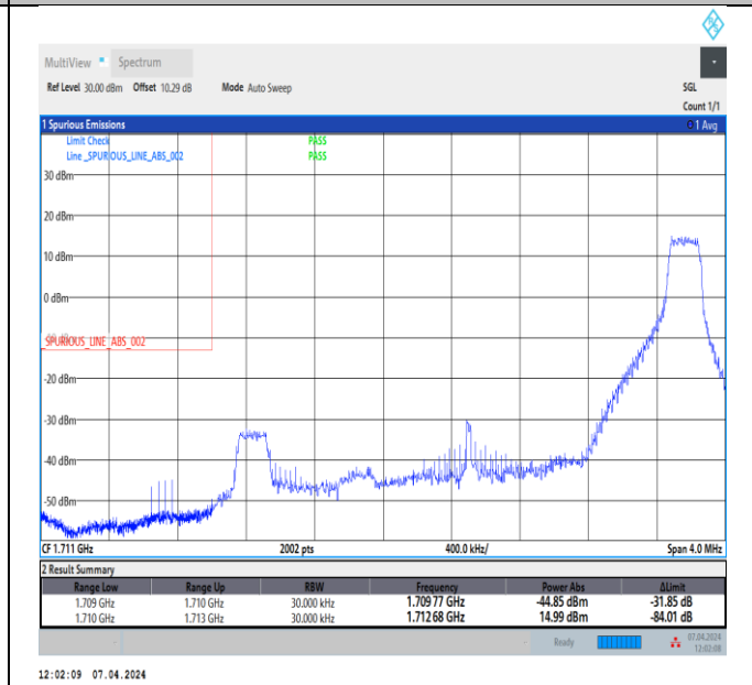
Band4_3MHz_64QAM_19965_1RB#14
