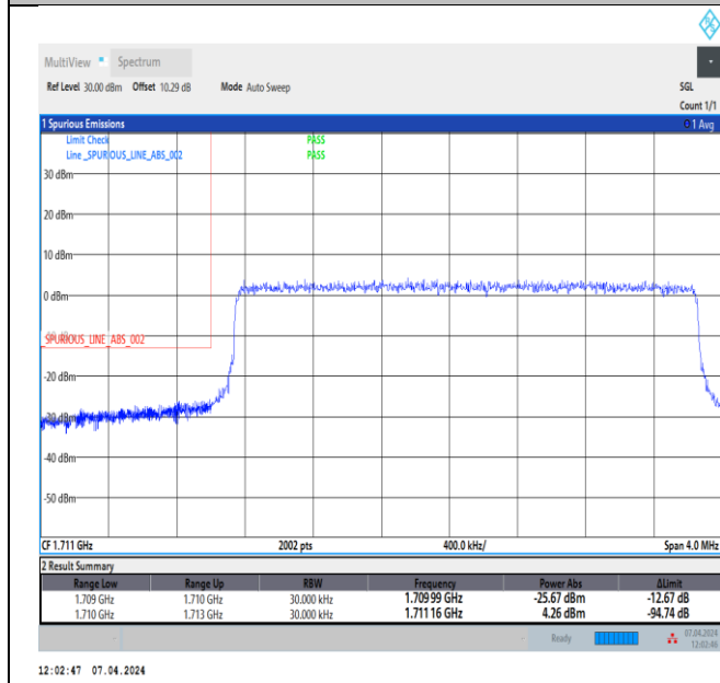
Band4_3MHz_16QAM_19965_15RB#0
