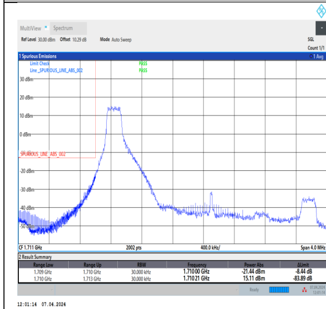
Band4_3MHz_64QAM_19965_1RB#0
