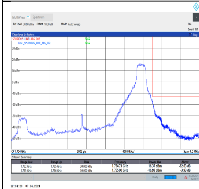
Band4_3MHz_QPSK_20385_1RB#14
