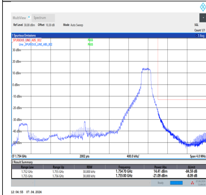
Band4_3MHz_64QAM_20385_1RB#14
