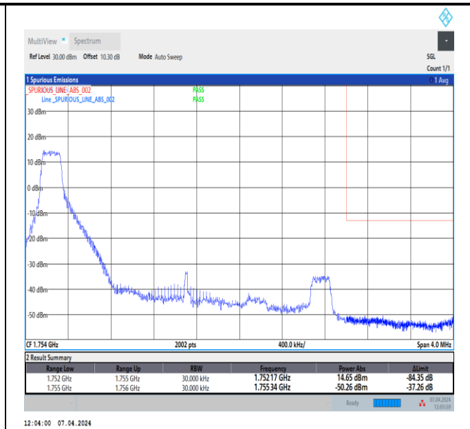
Band4_3MHz_64QAM_20385_1RB#0
