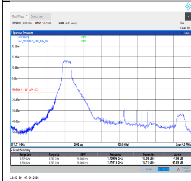
Band4_3MHz_QPSK_19965_1RB#0
