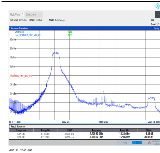
Band4_3MHz_16QAM_19965_1RB#0
