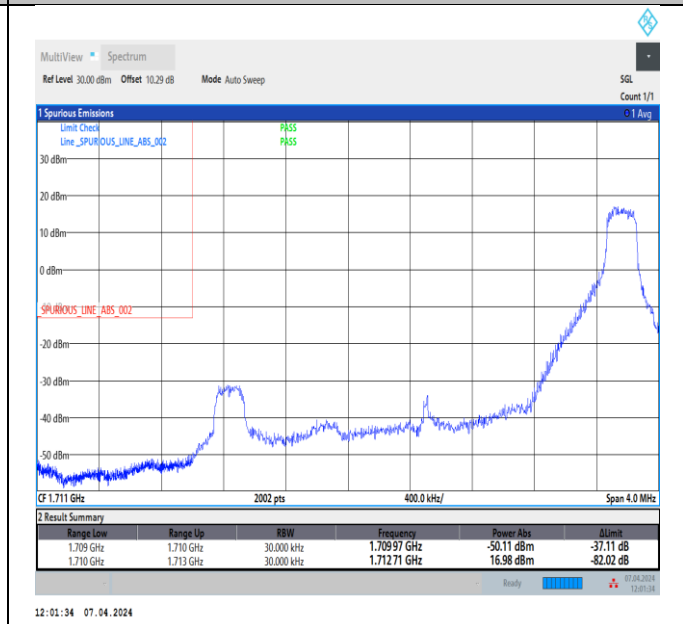
Band4_3MHz_QPSK_19965_1RB#14
