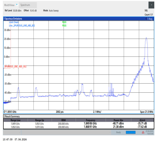
Band2_20MHz_64QAM_18700_1RB#99
