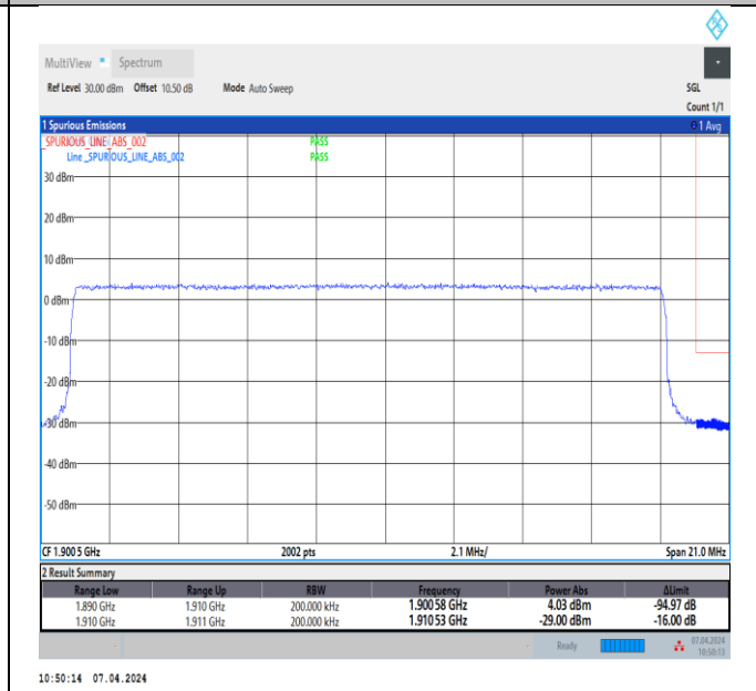
Band2_20MHz_QPSK_19100_100RB#0
