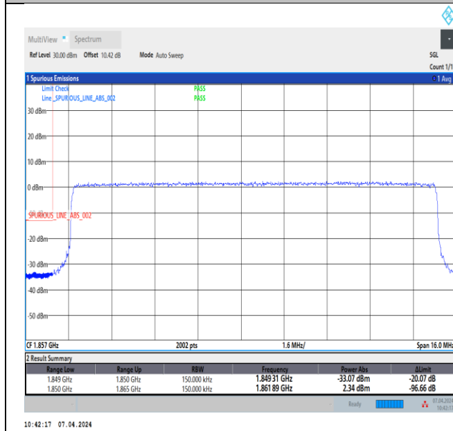
Band2_15MHz_64QAM_18675_75RB#0
