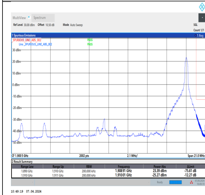
Band2_20MHz_QPSK_19100_1RB#99
