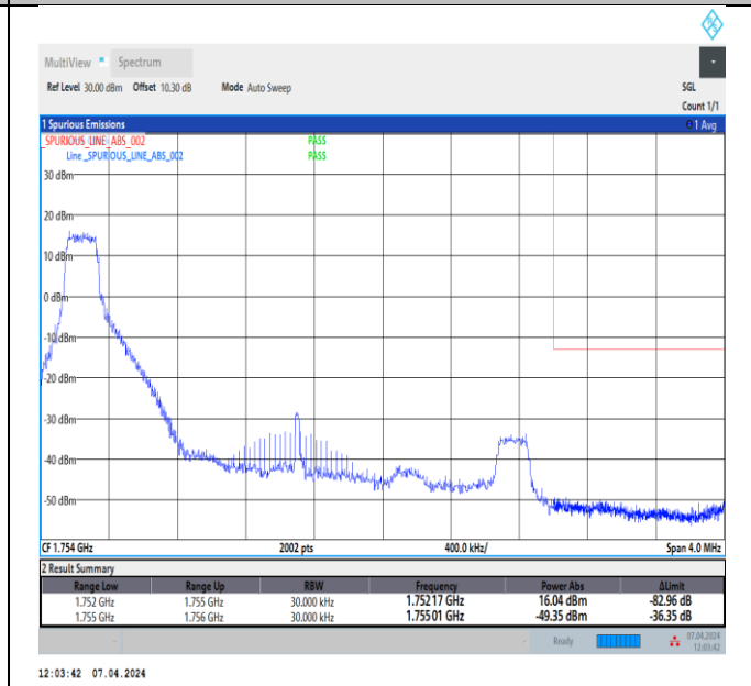
Band4_3MHz_16QAM_20385_1RB#0
