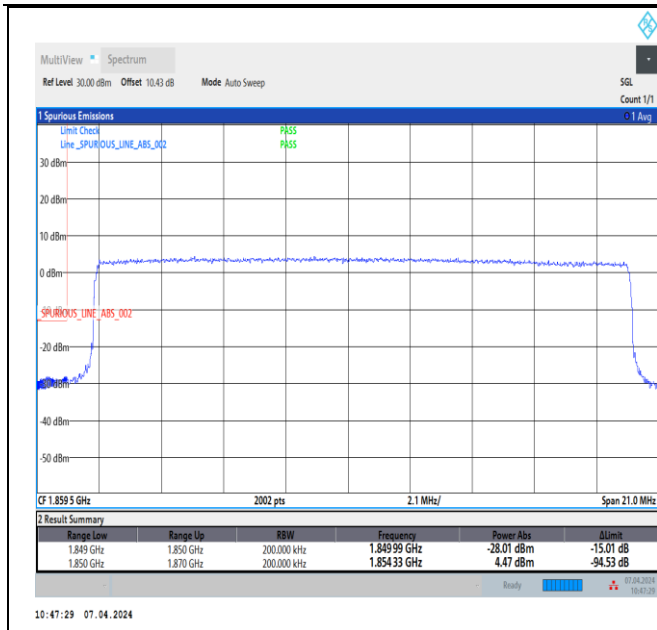
Band2_20MHz_QPSK_18700_100RB#0
