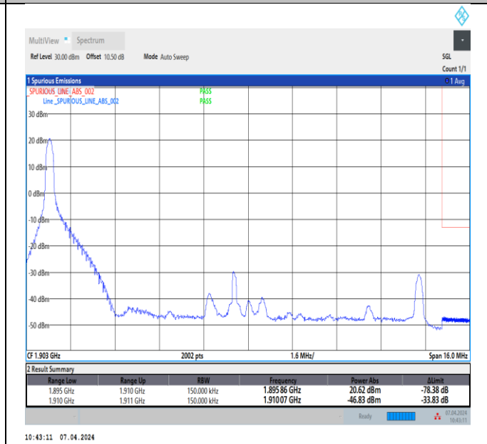
Band2_15MHz_64QAM_19125_1RB#0
