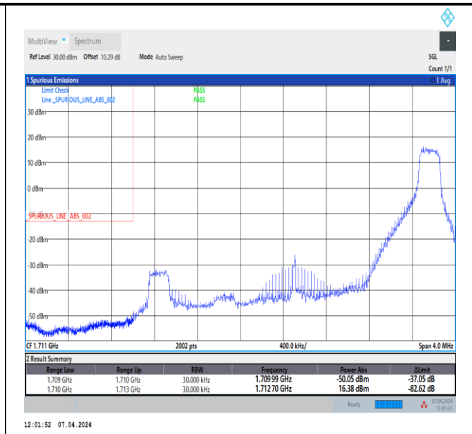
Band4_3MHz_16QAM_19965_1RB#14
