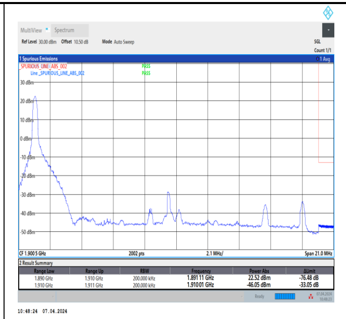
Band2_20MHz_QPSK_19100_1RB#0
