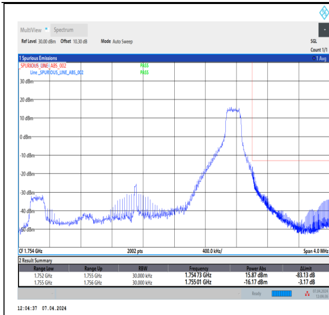
Band4_3MHz_16QAM_20385_1RB#14
