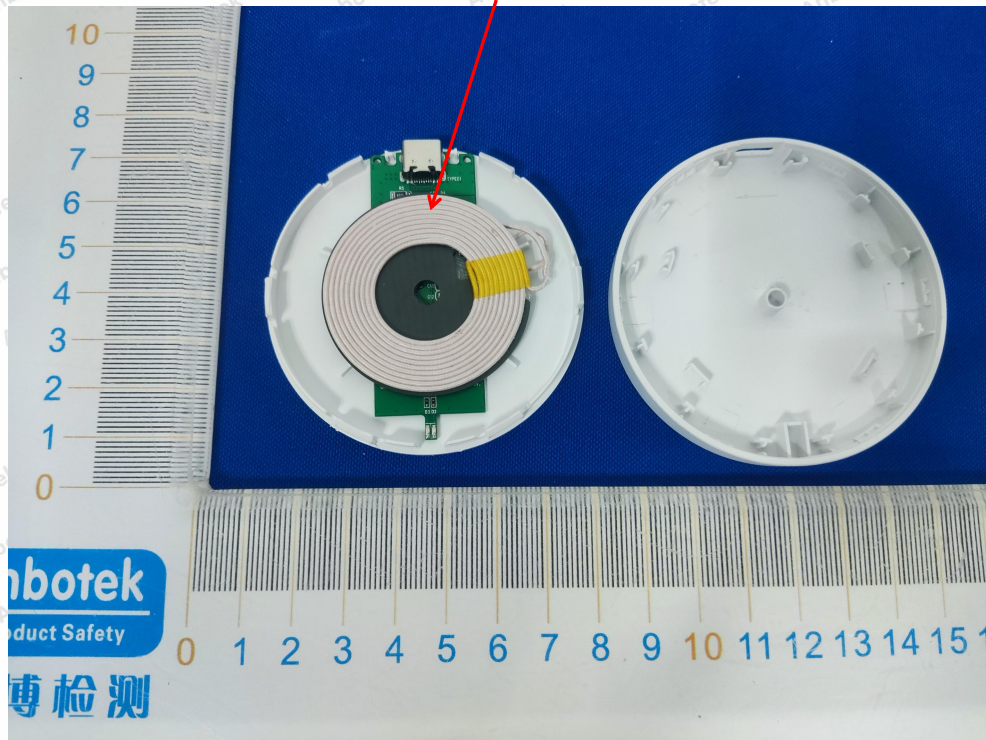
Internal Photograph
