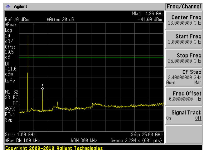
High Channels 1 GHz – 25 GHz
