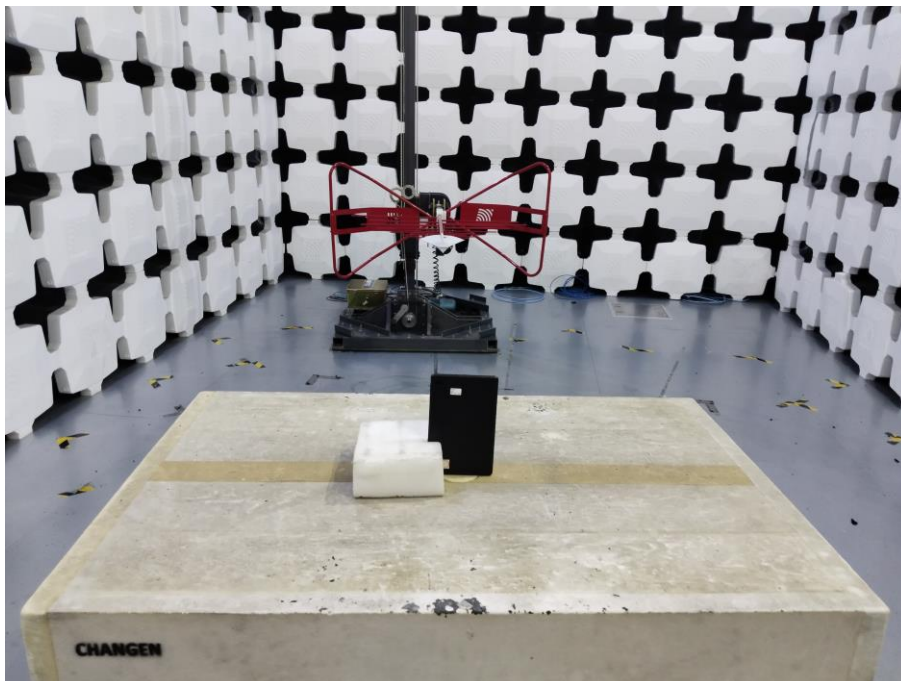
2. Radiated Emissions (Part 15C Wi-Fi/Bluetooth, 30MHz-1GHz)
