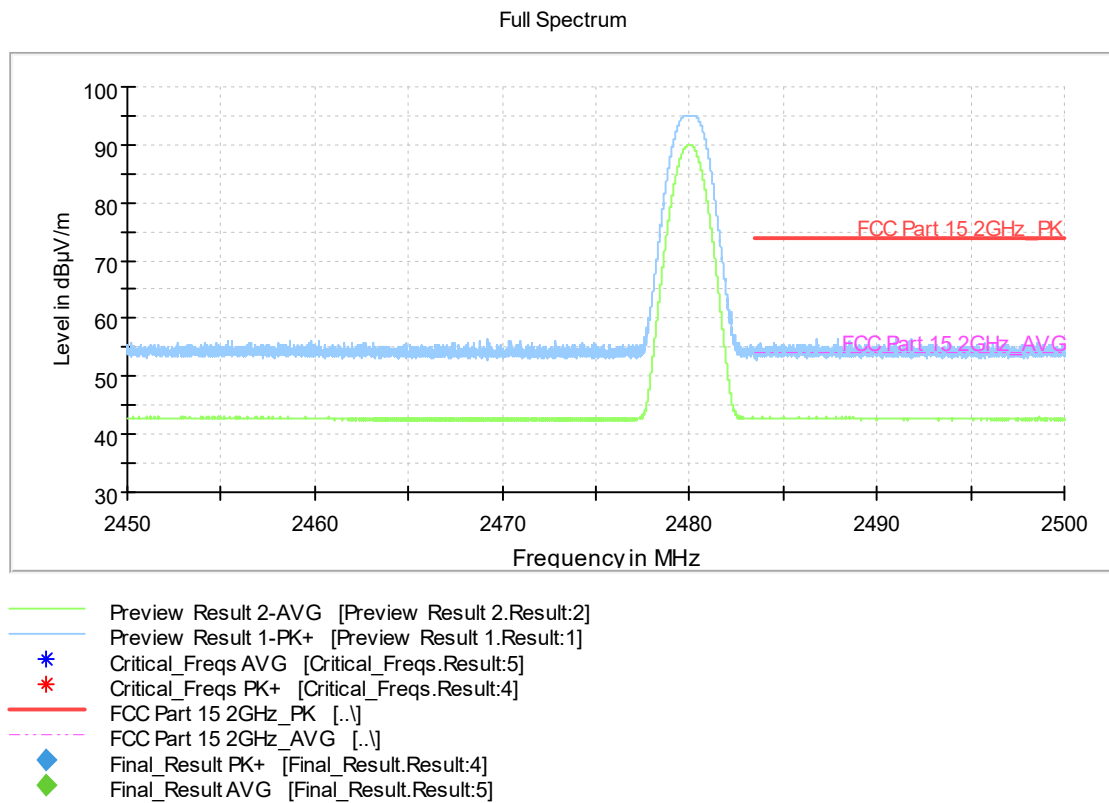
Fig.4. Frequency Band Edges: BLE GFSK, 2480 MHz, Hopping Off , 2.45 GHz - 2.50GHz
