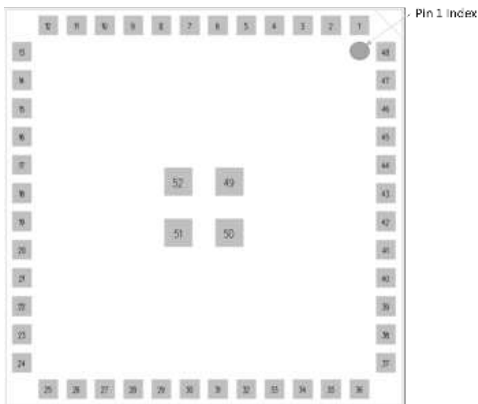
Figure 6.1. BGM241S Module Pinout (Top view)
