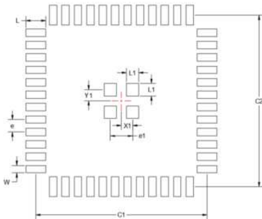
Figure 8.4. Recommended Land Pattern for Modules with a Built-in Antenna
