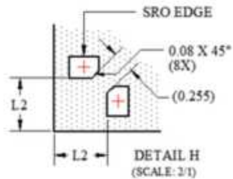
Figure 8.3. Bottom View about Package Corner
