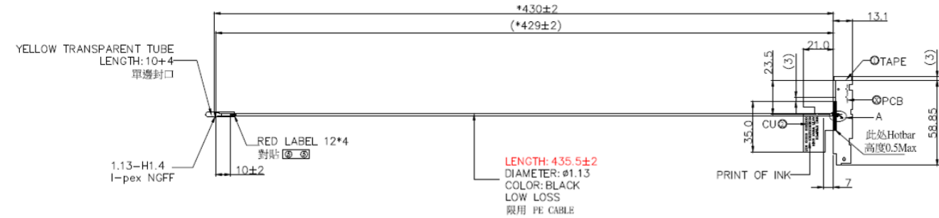
Ant5 Dimensioned Drawing:
