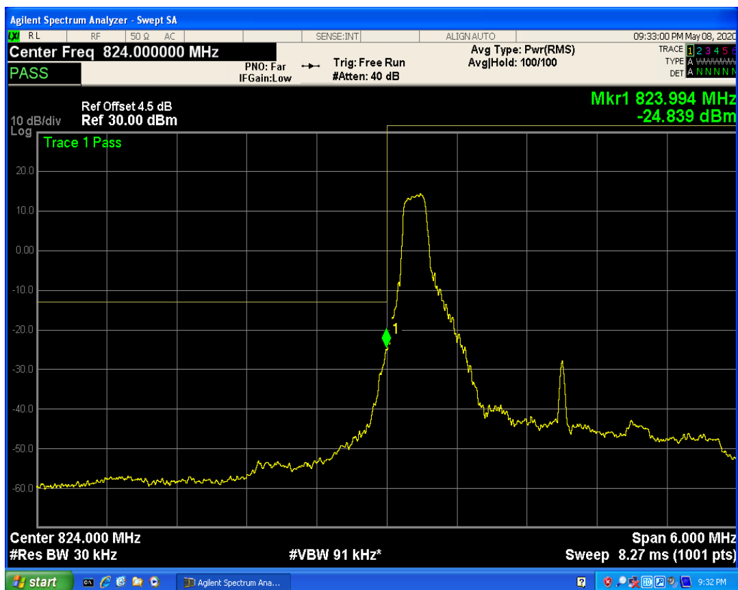
LTE Band5 QAM16 BW=3MHz Channel=20415 RB Size=15 Position=#0
