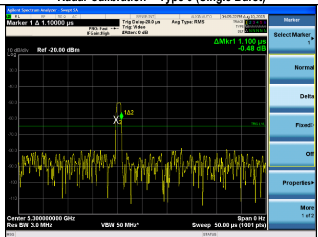
Radars Calibration - Type 1 (Single Burst)
