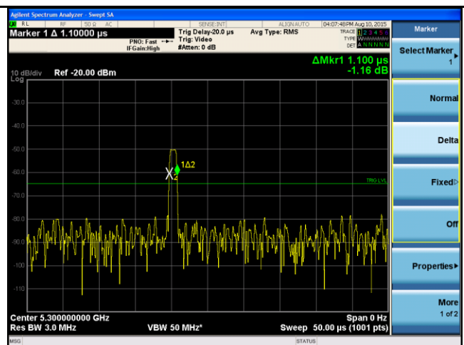
Radars Calibration - Type 0 (Single Burst)
