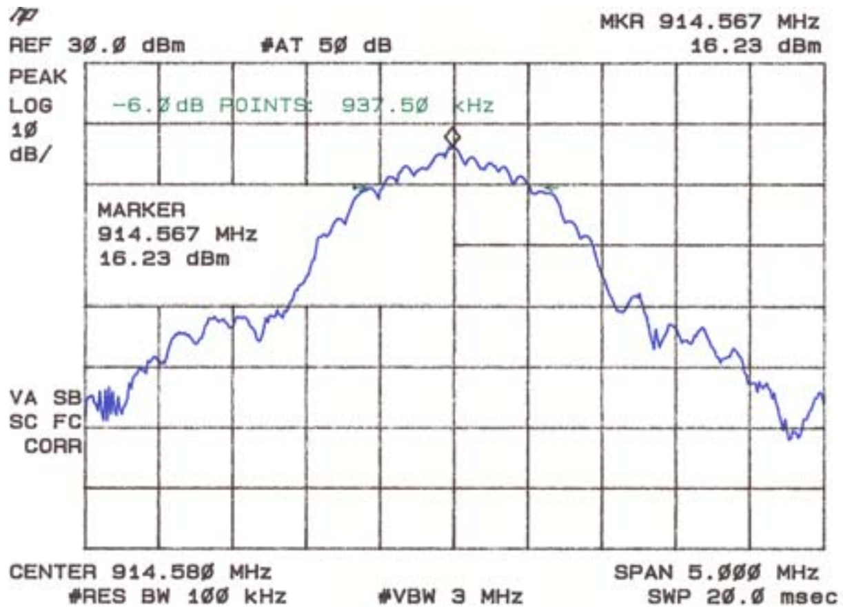
Figure 7b 6 dB Bandwidth per FCC Section 15.247(a)(2) – mid
