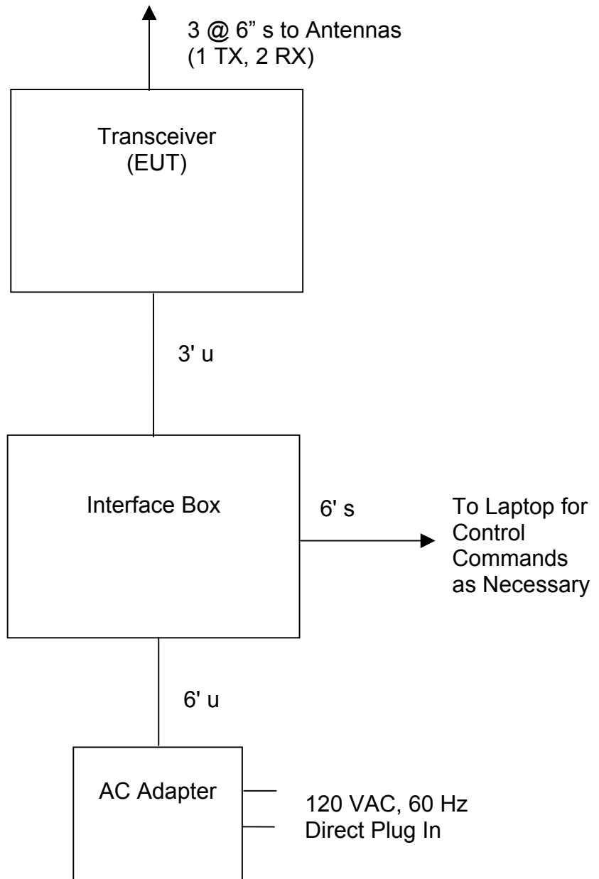
FIGURE 1 TEST CONFIGURATION
