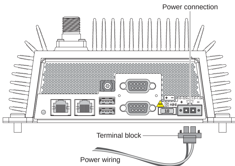
Figure 7 Power Plug Connection
