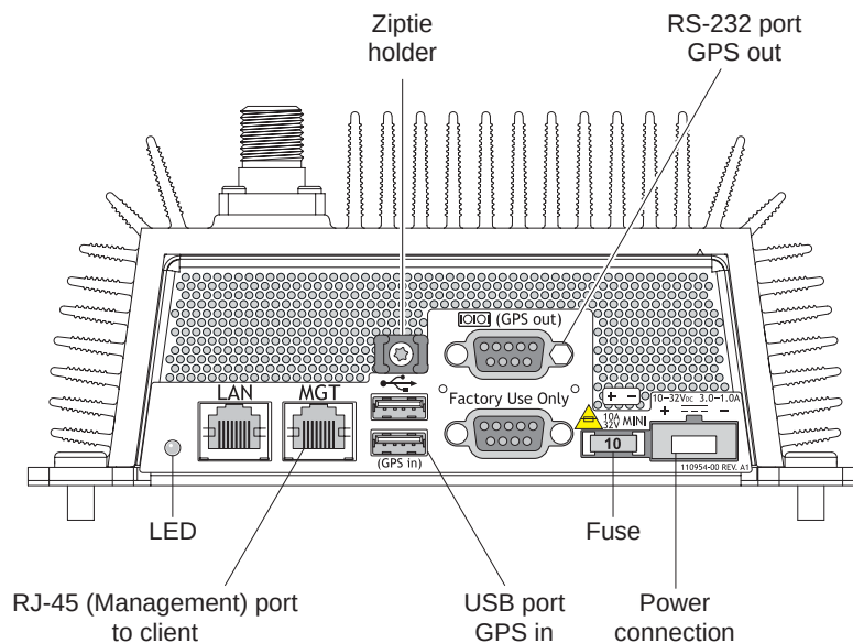
Figure 3 Connector Panel
