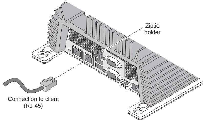
Figure 6 Ethernet Cable Connection
