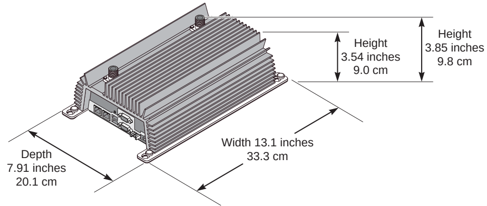
Figure 1 Tropos 4210 MetroMesh Router
