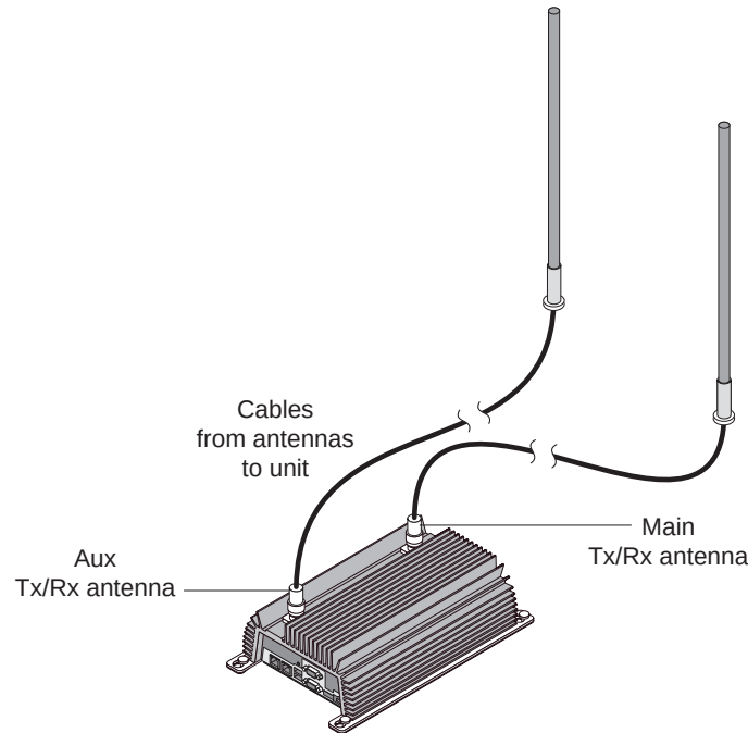
Figure 2 Tropos 4210 MetroMesh Routerwith Cable-Attached Antennas
