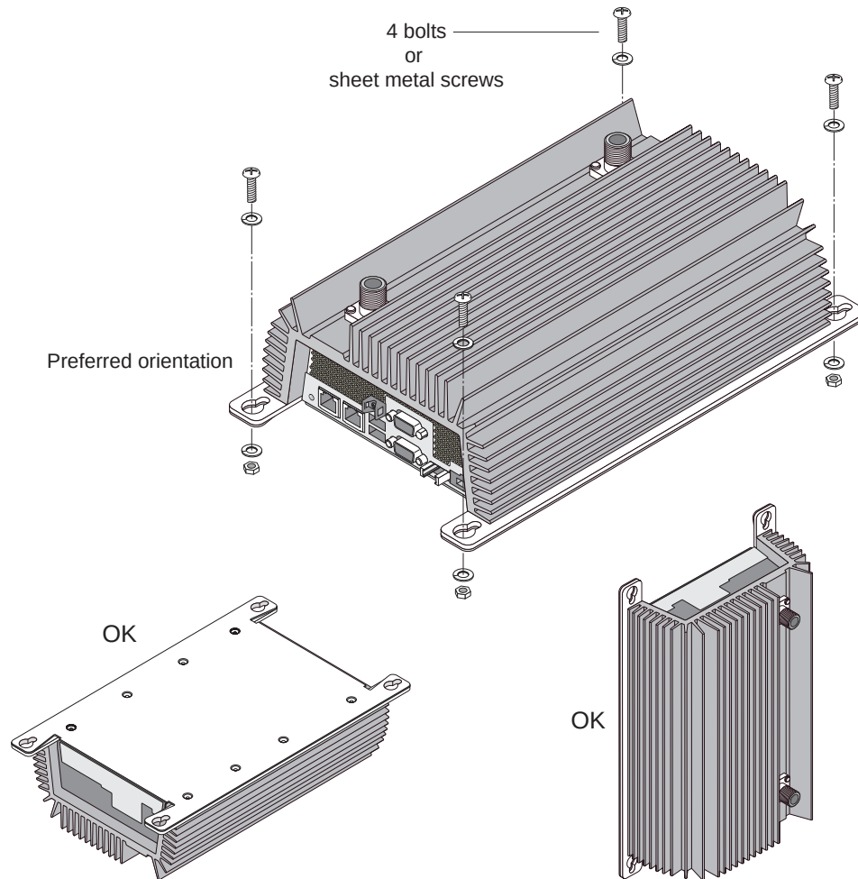
Figure 5 Attaching the Router to a Mounting Surface
