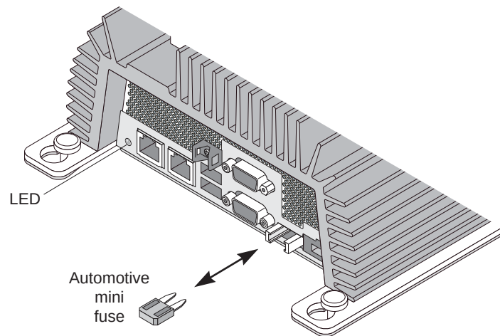
Figure 9 Fuse Replacement
