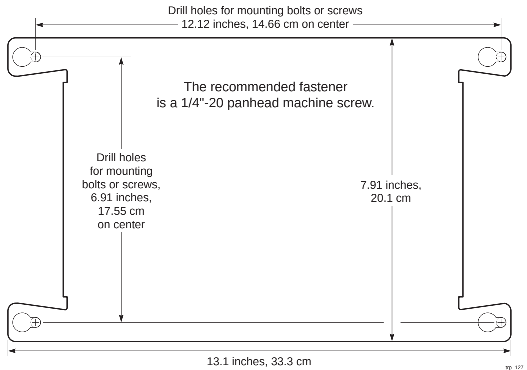
Figure 4 Preparing the Mounting Surface
