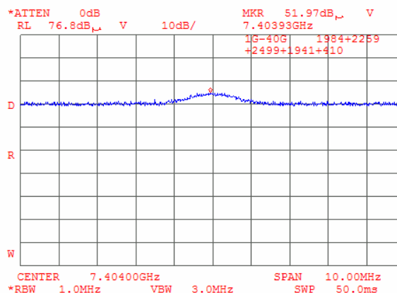
Plot 7.4.38 Radiated emission measurements at the forth harmonic of mid carrier frequency
