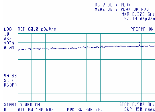
Plot 7.4.18 Radiated emission measurements from 5000 to 6500 MHz at the high carrier frequency
