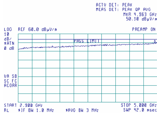
Plot 7.4.14 Radiated emission measurements from 2900 to 5000 MHz at the mid carrier frequency
