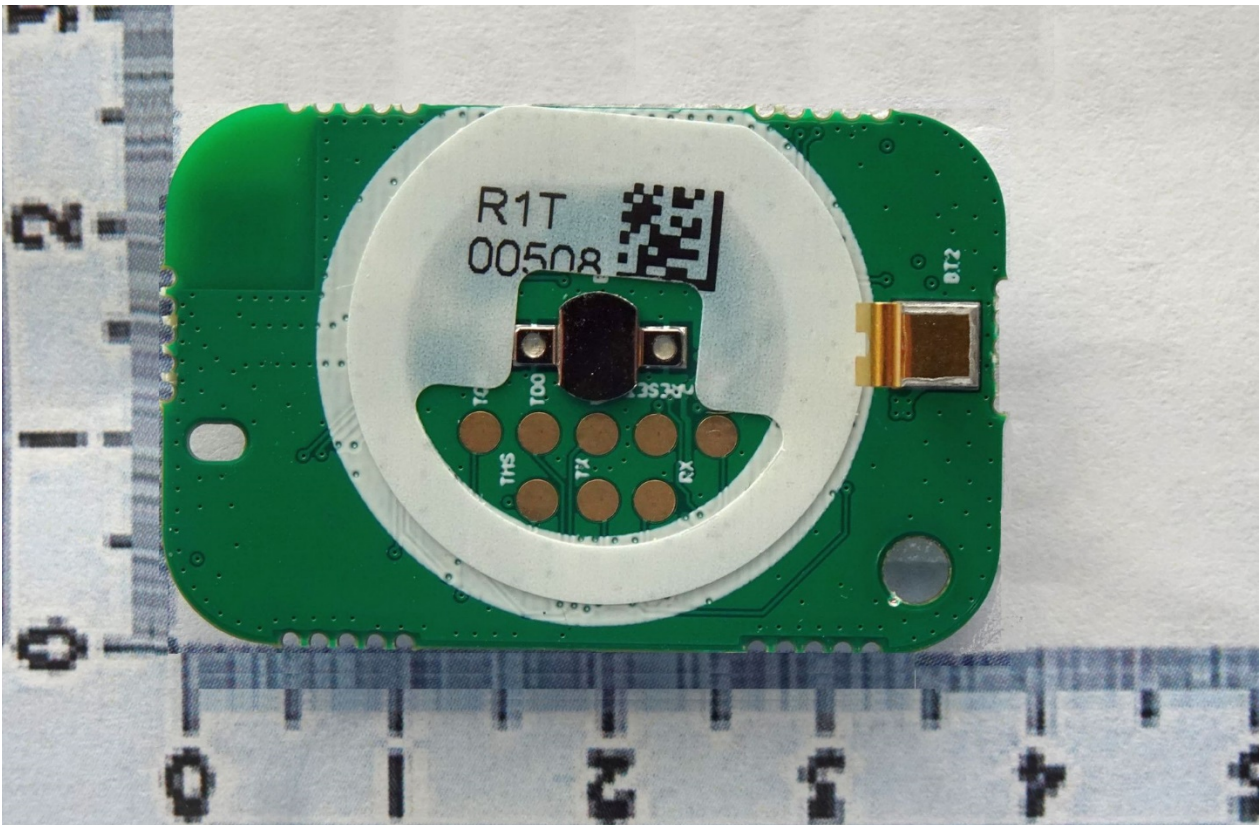
R1T KFB PCBA, Battery side View
