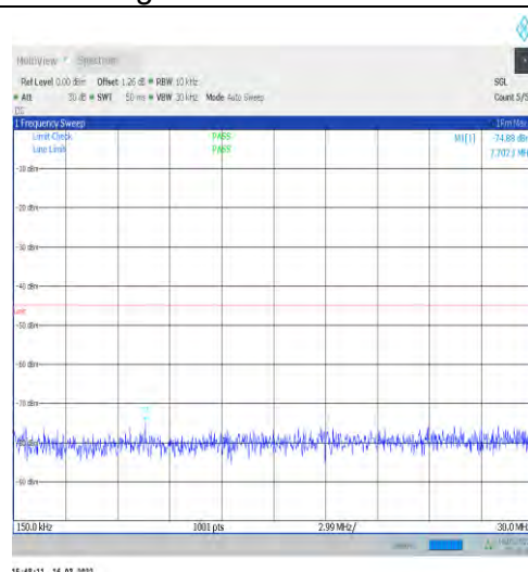
1-N41-30-100-H-1-DFT-PI2BPSK-Inner_1RB_Left-1 @1-0.15-30-Ant1--74.88--45-PASS
