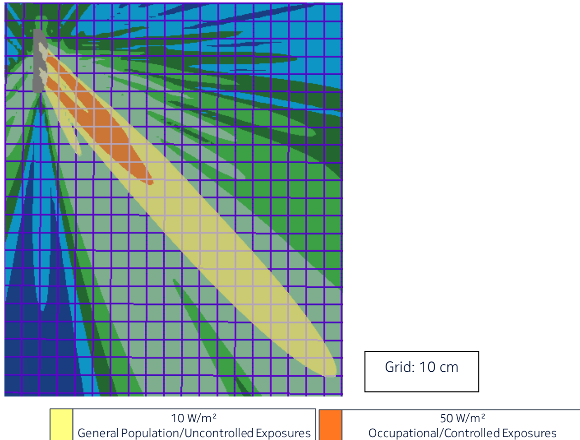
Figure 4 – Top view of AEWB power density for the time-averaged maximum transmitted power of 1.33 W and the beam oriented in azimuth = 45° & elevation = 0°
