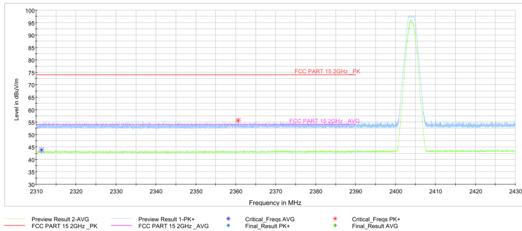
Fig.18. Frequency Band Edges: GFSK, 2402 MHz, Hopping Off, 2.31 GHz – 2.43GHz
