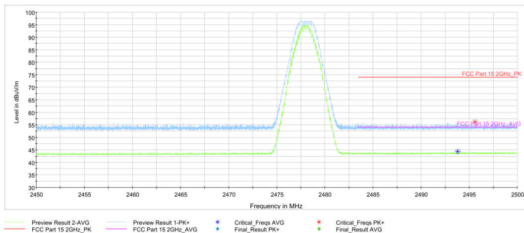
Fig.19. Frequency Band Edges: GFSK, 2480 MHz, Hopping Off, 2.45 GHz - 2.50GHz
