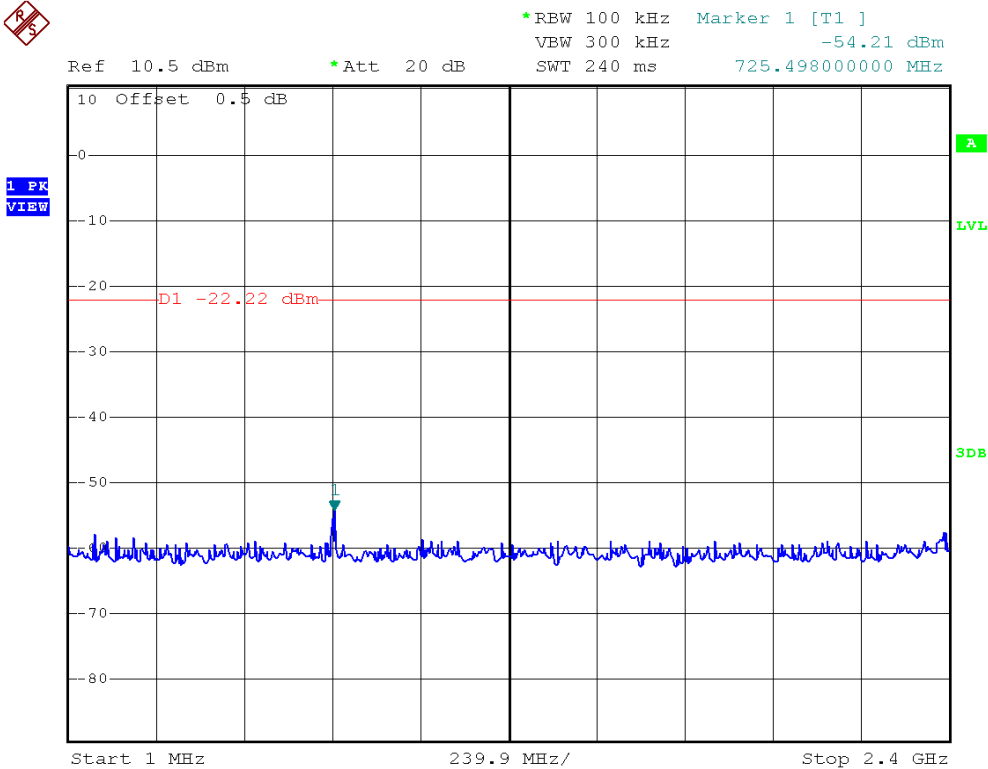
802.11g, Highest Channel, Plot A
