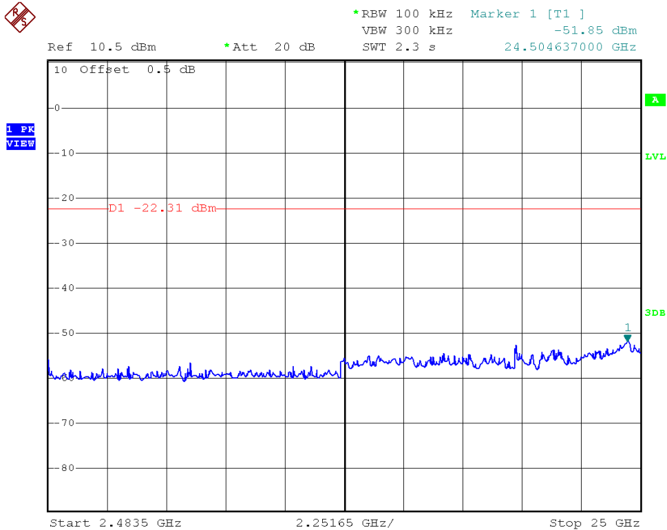
802.11g, Middle Channel, Plot B
