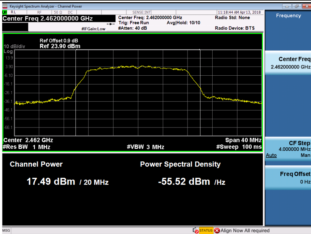
Maximum peak conducted output power_11G_2462_Ant1
