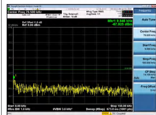
Band38-5MHz-16QAM-37775-1RB#24-0.009~0. 15-PASS
