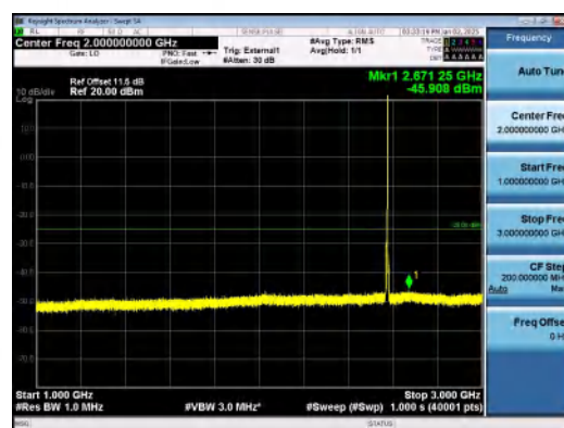
Band38-5MHz-16QAM-37775-1RB#24-1000~30 00-PASS
