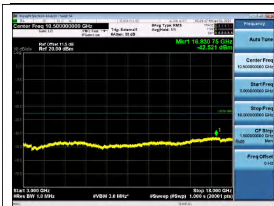
Band38-5MHz-16QAM-37775-1RB#0-3000~180 00-PASS
