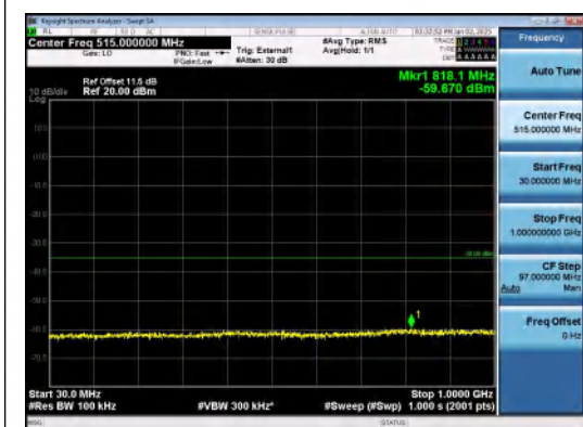
Band38-5MHz-16QAM-37775-1RB#24-30~1000- PASS
