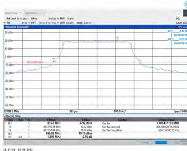
Band26-1.4MHz-QPSK-26915-6RB#0
