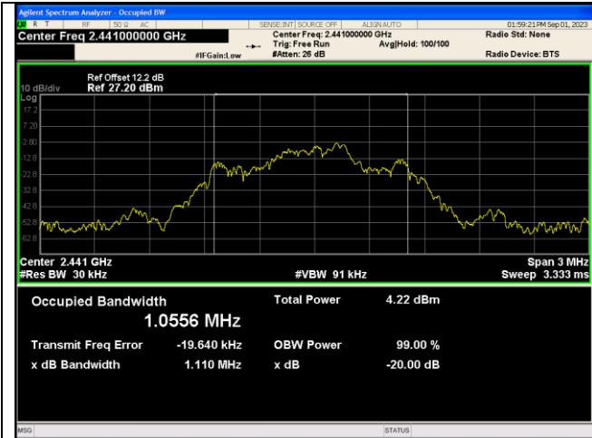
\pi/4 DQPSK_2-DH5_Channel 39
