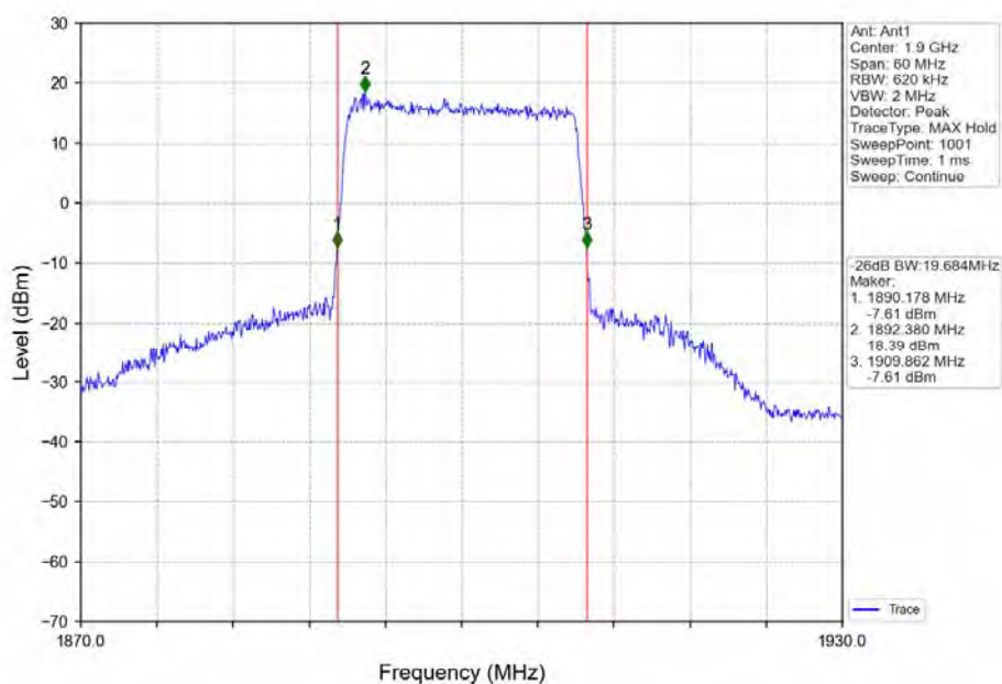
Band2_20MHz_64QAM_HCH_1900MHz_RB_100_0_NTNV
