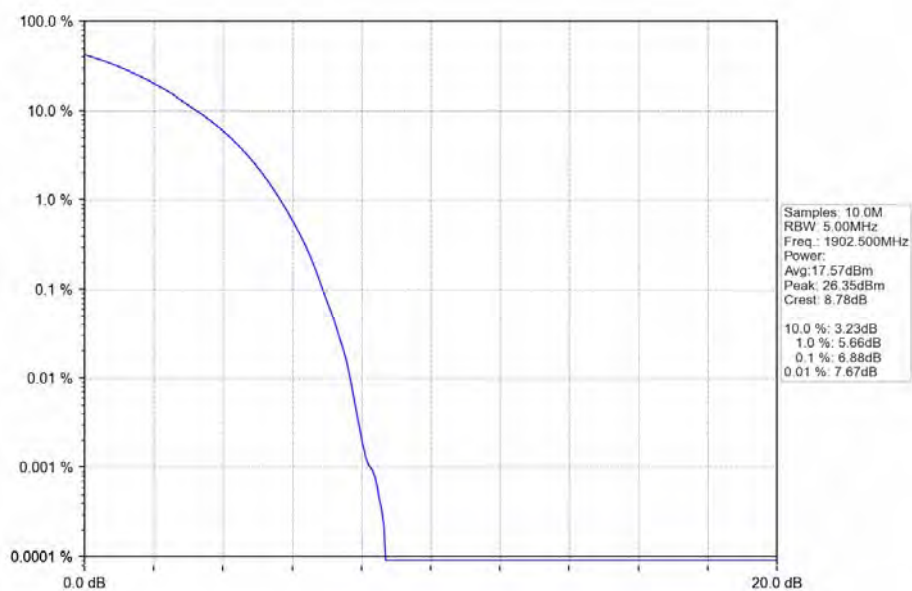
Band2_15MHz_64QAM_HCH_1902.5MHz_RB_75_0_NTNV
