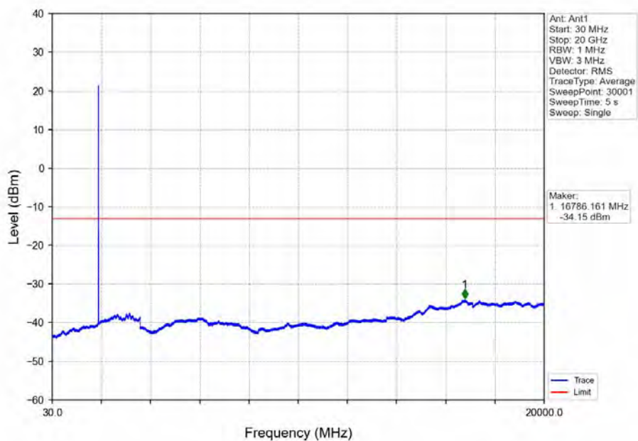
Band2_5MHz_64QAM_HCH_1907.5MHz_RB_1_24_NTNV
