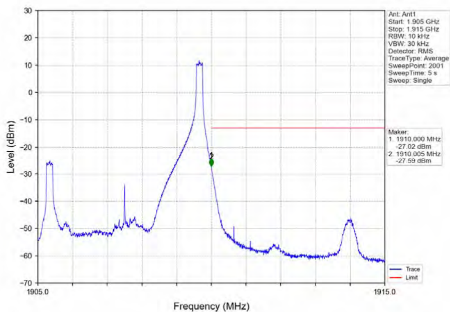
Band2_5MHz_16QAM_HCH_1907.5MHz_RB_25_0_NTNV
