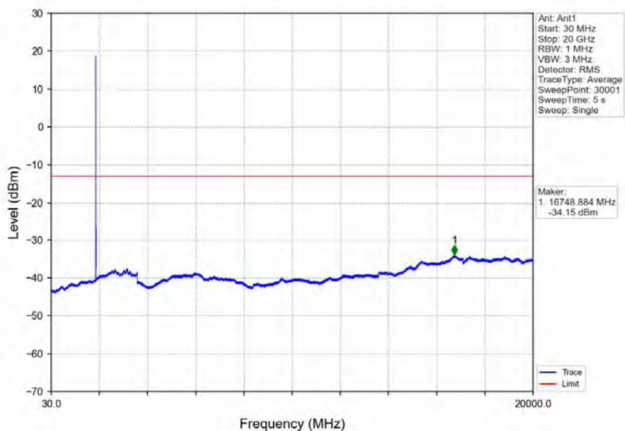
Band2_3MHz_64QAM_MCH_1880MHz_RB_1_0_NTNV
