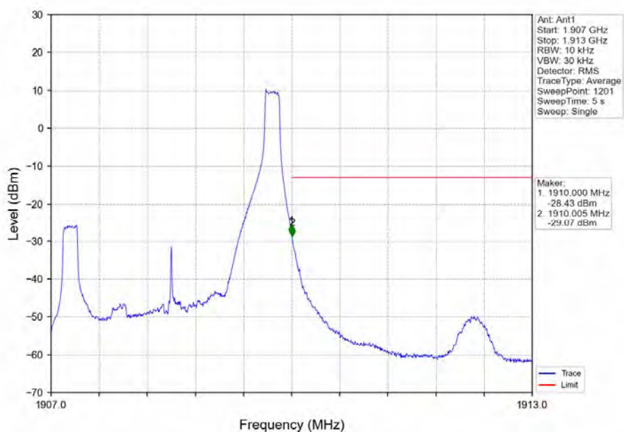
Band2_3MHz_64QAM_HCH_1908.5MHz_RB_1_14_NTNV
