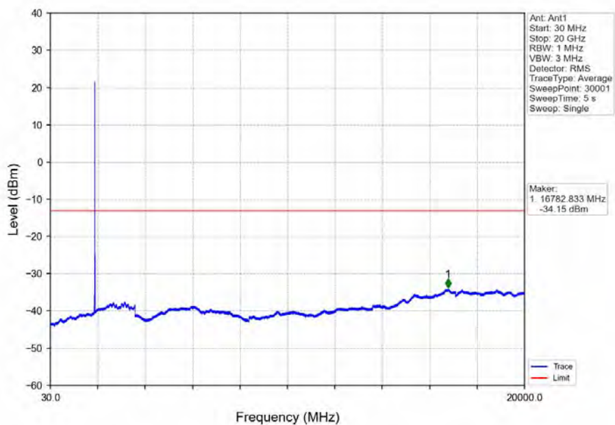
Band2_10MHz_64QAM_HCH_1905MHz_RB_1_49_NTNV
