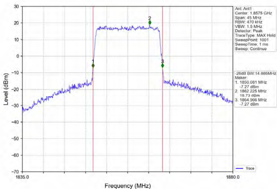
Band2_15MHz_16QAM_LCH_1857.5MHz_RB_75_0_NTNV
