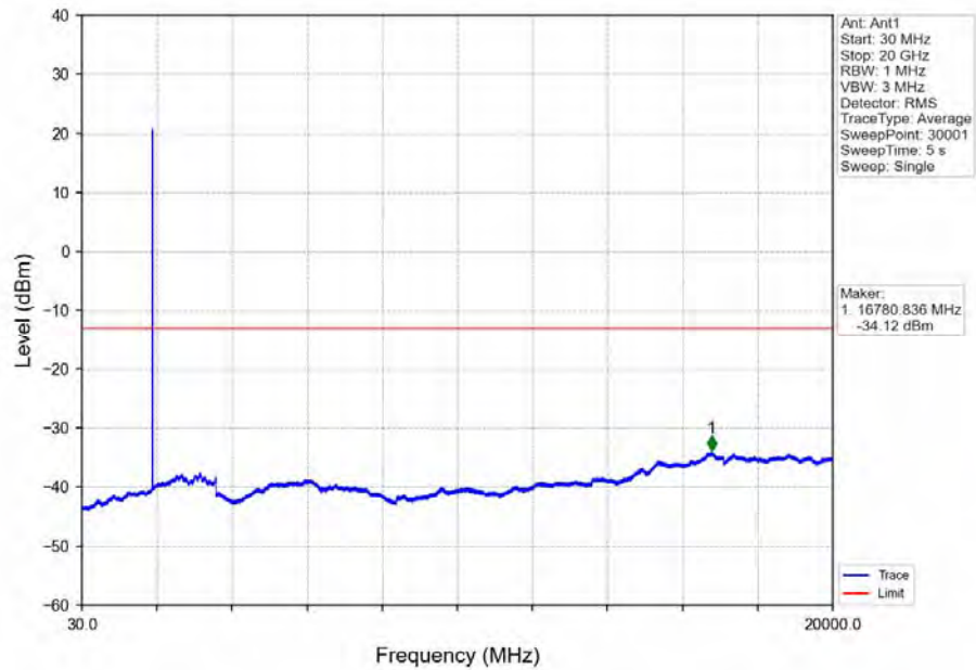
Band2_1.4MHz_64QAM_HCH_1909.3MHz_RB_1_5_NTNV
