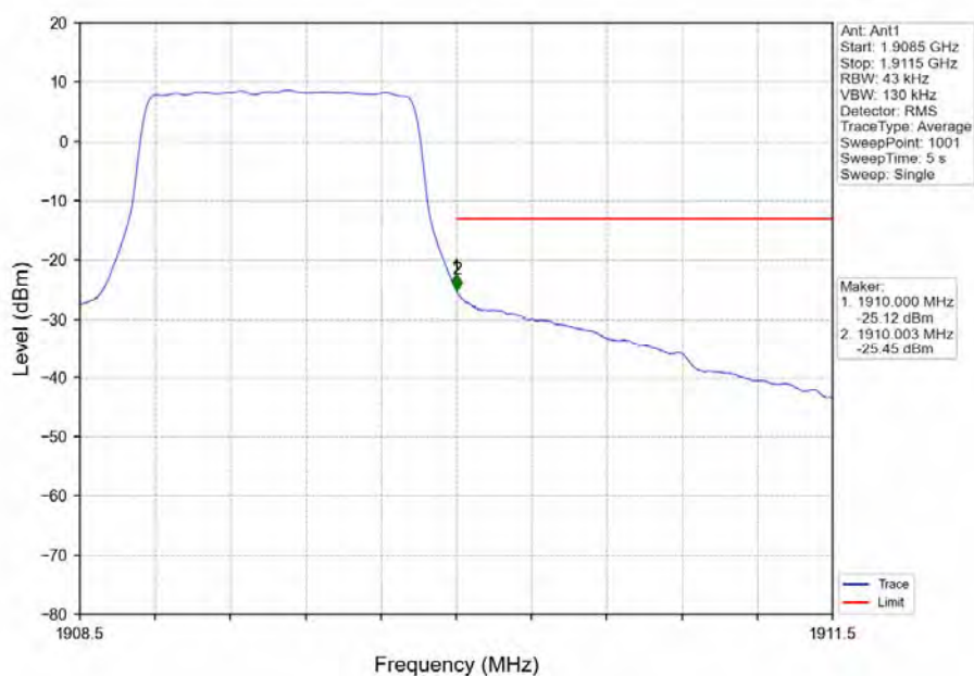
Band2_1.4MHz_16QAM_HCH_1909.3MHz_RB_6_0_NTNV
