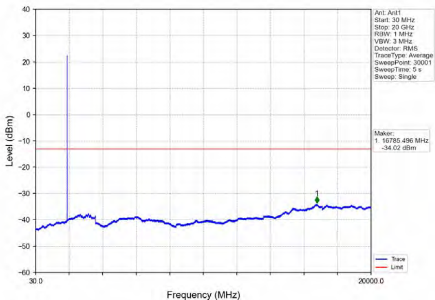
Band2_5MHz_16QAM_HCH_1907.5MHz_RB_1_0_NTNV
