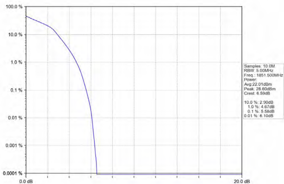
Band2_3MHz_16QAM_LCH_1851.5MHz_RB_15_0_NTNV
