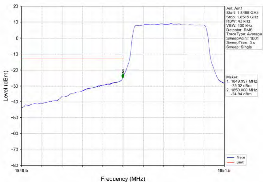
Band2_1.4MHz_16QAM_LCH_1850.7MHz_RB_6_0_NTNV
