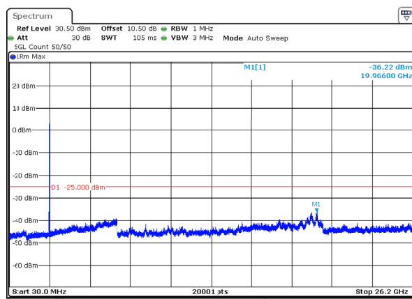
n38_30MHz_30kHz_2595MHz_DFT-s-OFDM QPSK_RB1@77 -36.22dBm
