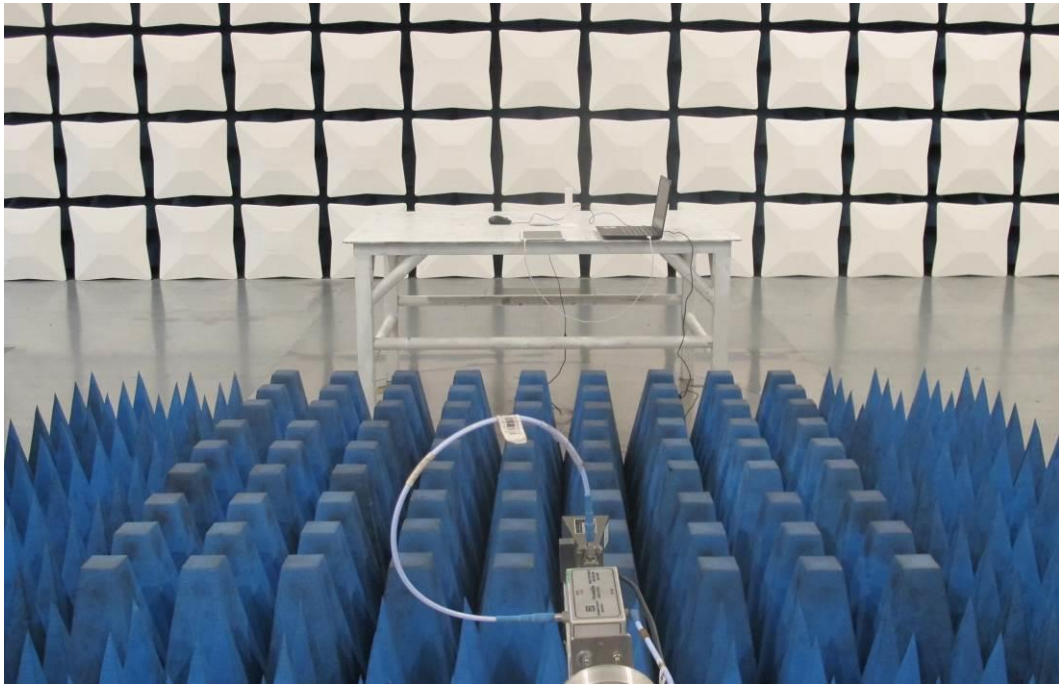
Radiated Disturbance Emissions (18GHz to 26.5GHz)
