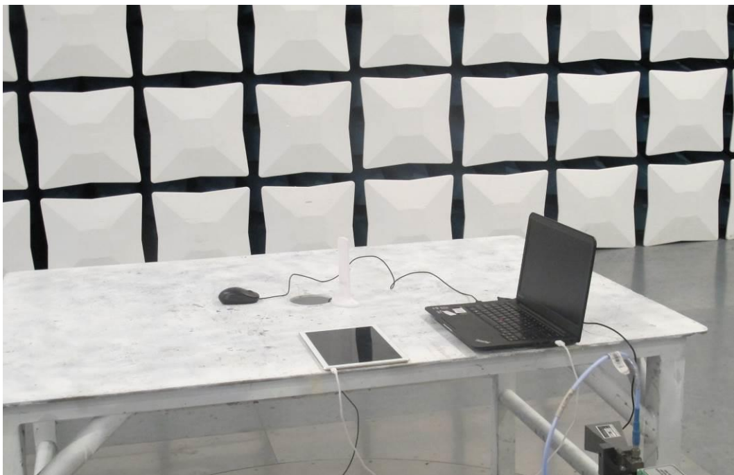
Radiated Disturbance Emissions (26.5GHz to 40GHz)
