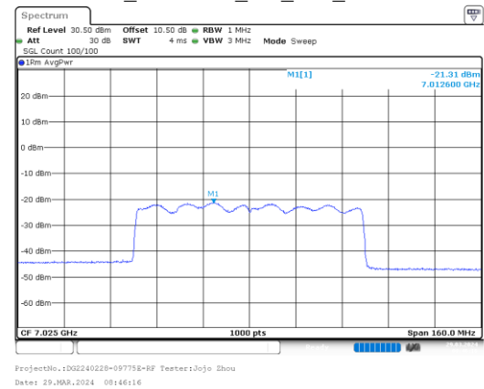
ax80_7025MHz_RU_Full_Chain 1
