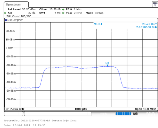
ax20_7095MHz_RU_Full_Chain 1
