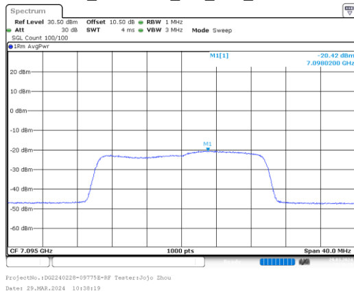
ax20_7095MHz_RU_Full_Chain 2
