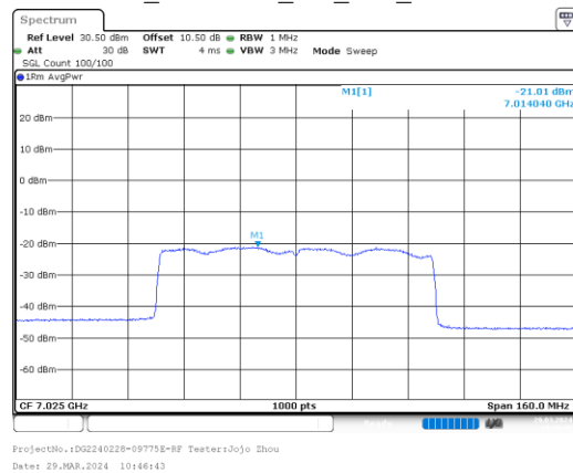
ax80_7025MHz_RU_Full_Chain 2
