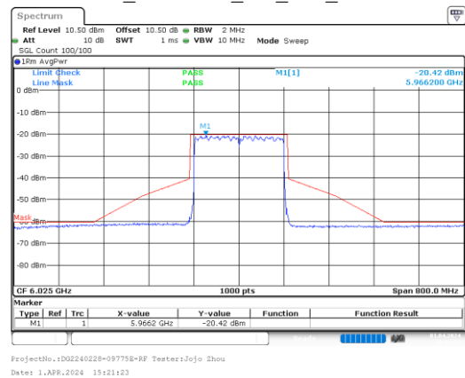
ax160_6025MHz_RU_Full_Chain 3
