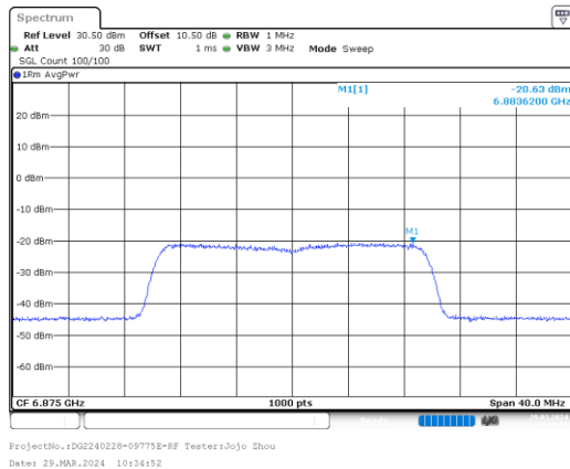
ax20_6875MHz_RU_Full_Chain 2
