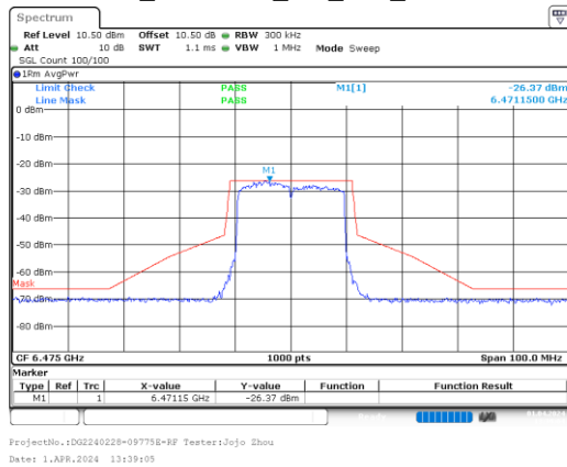
ax20_6475MHz_RU_Full_Chain 2
