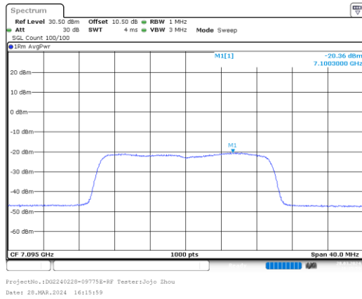
ax20_7095MHz_RU_Full_Chain 0
