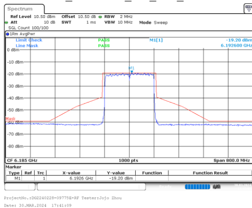
ax160_6185MHz_RU_Full_Chain 0
