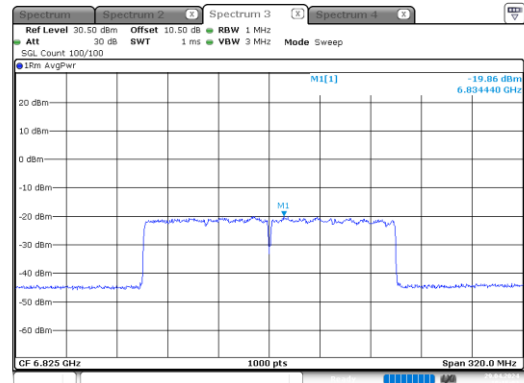
ax160_6825MHz_RU_Full_Chain 1
