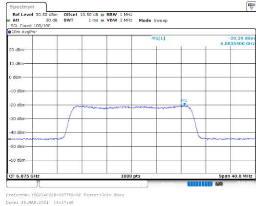
ax20_6875MHz_RU_Full_Chain 1
