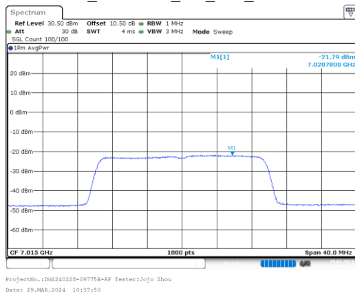
ax20_7015MHz_RU_Full_Chain 2
