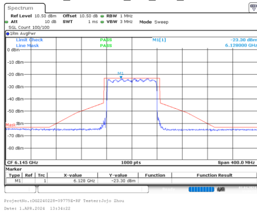
ax80_6145MHz_RU_Full_Chain 2
