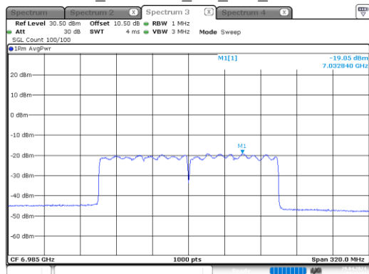
ax160_6985MHz_RU_Full_Chain 2
