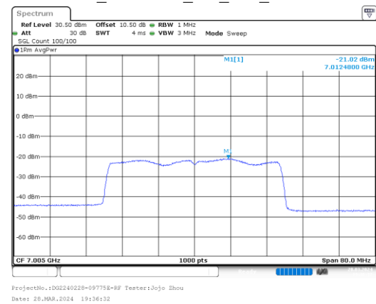
ax40_7005MHz_RU_Full_Chain 1
