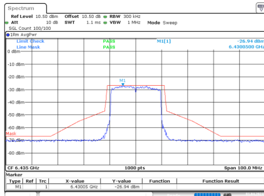
ax20_6435MHz_RU_Full_Chain 2
