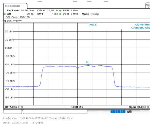
ax40_7085MHz_RU_Full_Chain 0
