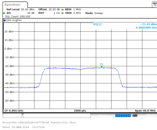
ax20_6895MHz_RU_Full_Chain 2
