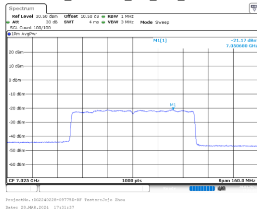
ax80_7025MHz_RU_Full_Chain 0
