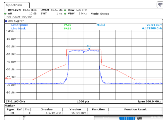
ax40_6165MHz_RU_Full_Chain 3
