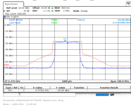
ax20_6475MHz_RU_Full_Chain 3
