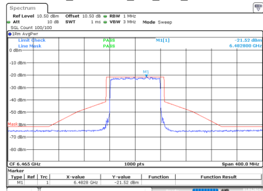
ax80_6465MHz_RU_Full_Chain 3
