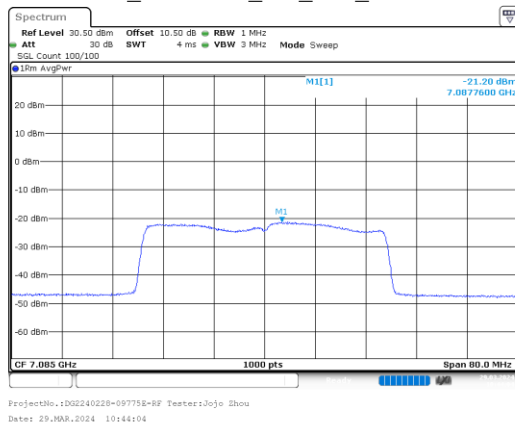
ax40_7085MHz_RU_Full_Chain 2
