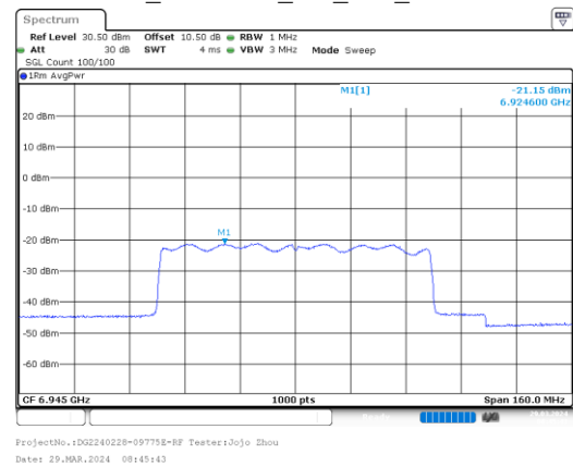
ax80_6945MHz_RU_Full_Chain 1
