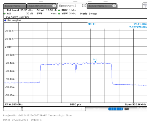
ax160_6985MHz_RU_Full_Chain 0
