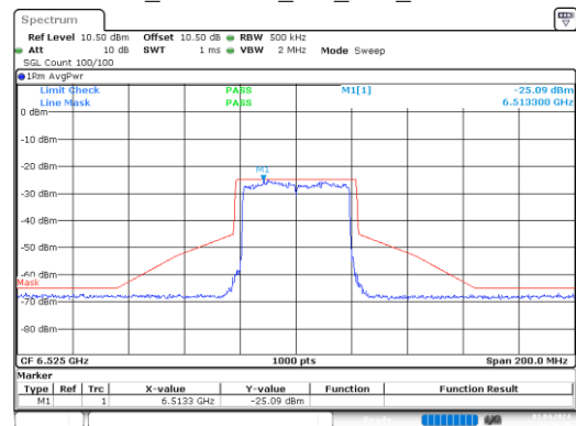
ax40_6525MHz_RU_Full_Chain 1
