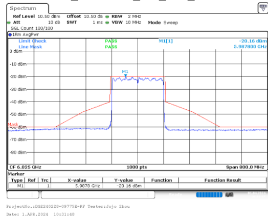
ax160_6025MHz_RU_Full_Chain 1
