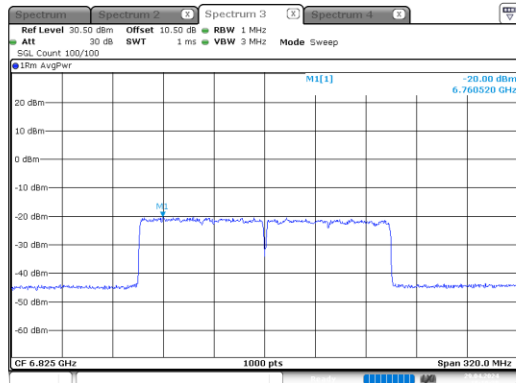
ax160_6825MHz_RU_Full_Chain 0
