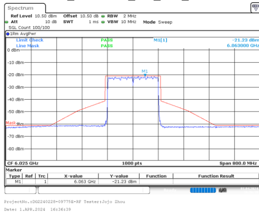
ax160_6025MHz_RU_Full_Chain 0
