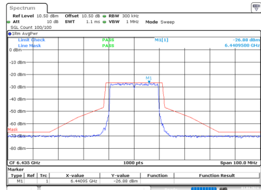
ax20_6435MHz_RU_Full_Chain 3
