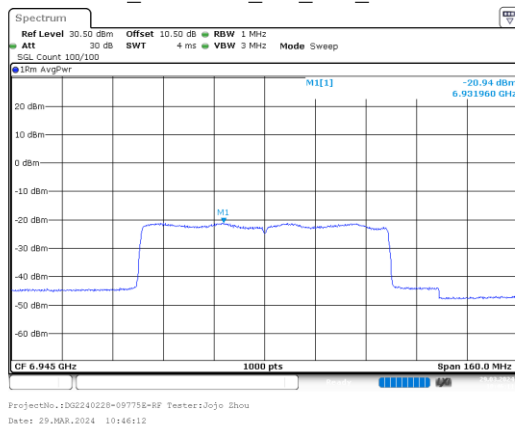
ax80_6945MHz_RU_Full_Chain 2
