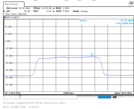
ax20_7015MHz_RU_Full_Chain 1
