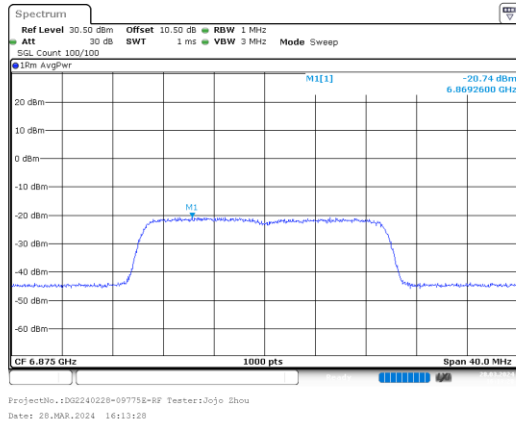
ax20_6875MHz_RU_Full_Chain 0
