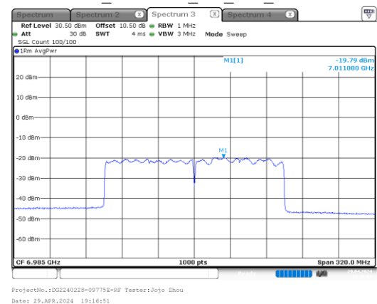
ax160_6985MHz_RU_Full_Chain 1
