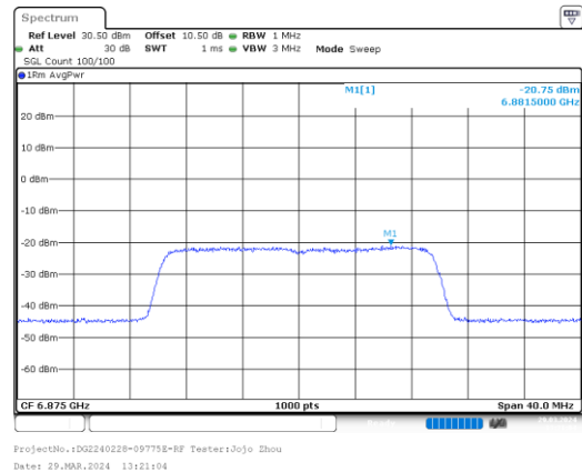
ax20_6875MHz_RU_Full_Chain 3
