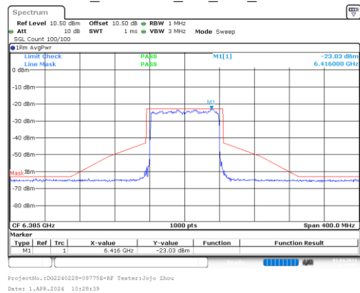
ax80_6385MHz_RU_Full_Chain 1
