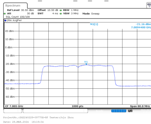
ax40_7005MHz_RU_Full_Chain 0
