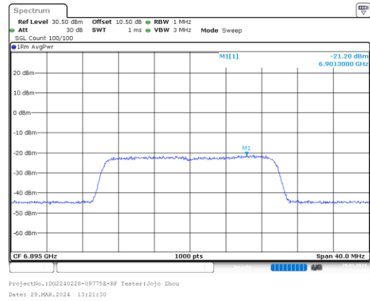
ax20_6895MHz_RU_Full_Chain 3
