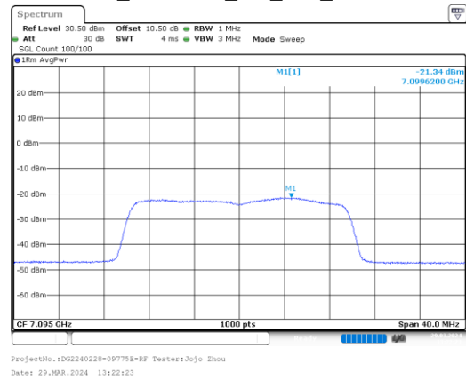
ax20_7095MHz_RU_Full_Chain 3
