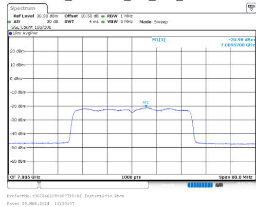
ax40_7085MHz_RU_Full_Chain 3
