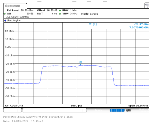
ax40_7005MHz_RU_Full_Chain 2
