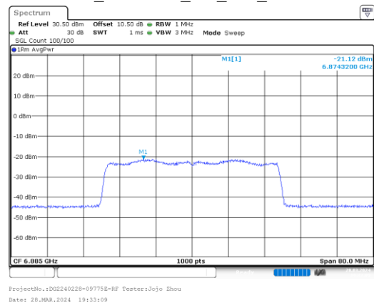
ax40_6885MHz_RU_Full_Chain 1
