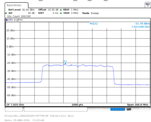
ax80_7025MHz_RU_Full_Chain 3
