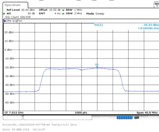
ax20_7015MHz_RU_Full_Chain 0
