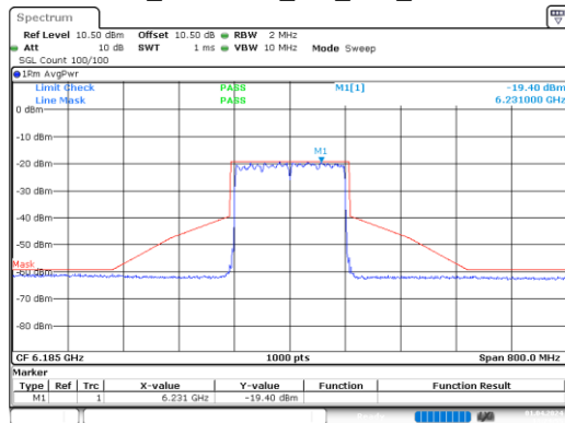
ax160_6185MHz_RU_Full_Chain 2
