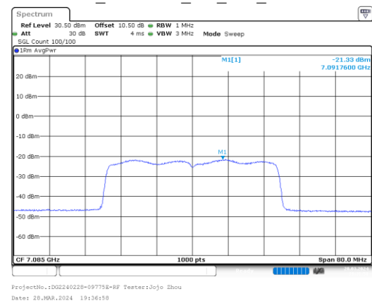
ax40_7085MHz_RU_Full_Chain 1
