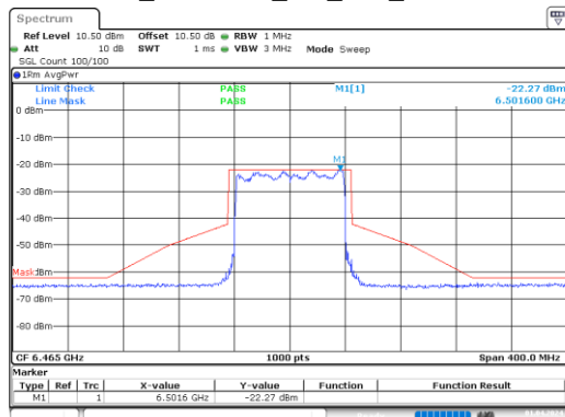
ax80_6465MHz_RU_Full_Chain 2
