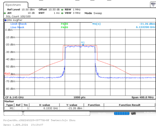
ax80_6145MHz_RU_Full_Chain 3
