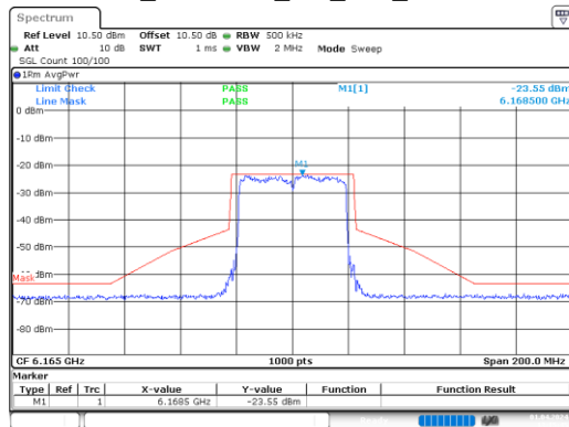
ax40_6165MHz_RU_Full_Chain 2
