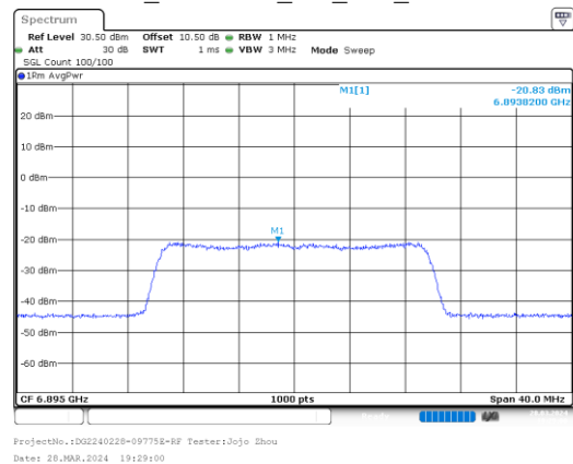
ax20_6895MHz_RU_Full_Chain 1
