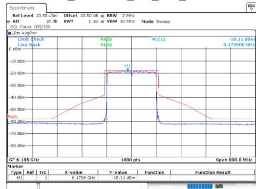
ax160_6185MHz_RU_Full_Chain 3
