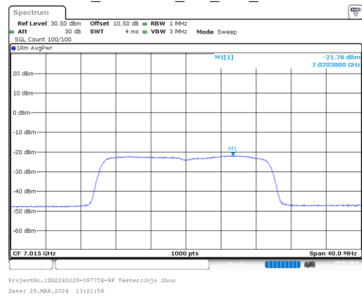
ax20_7015MHz_RU_Full_Chain 3
