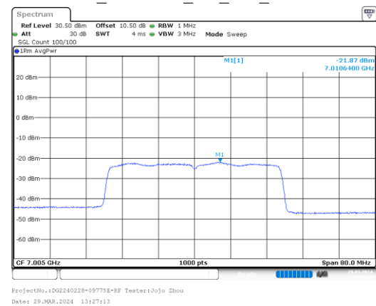
ax40_7005MHz_RU_Full_Chain 3
