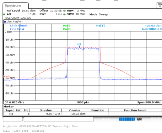
ax160_6025MHz_RU_Full_Chain 2
