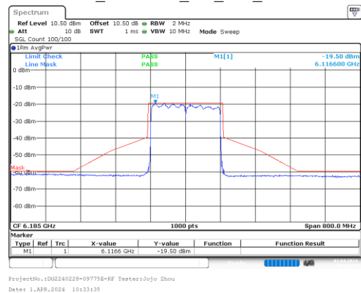
ax160_6185MHz_RU_Full_Chain 1
