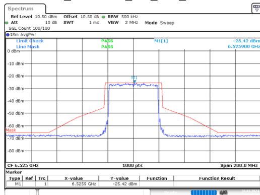
ax40_6525MHz_RU_Full_Chain 0
