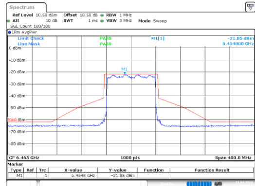
ax80_6465MHz_RU_Full_Chain 1
