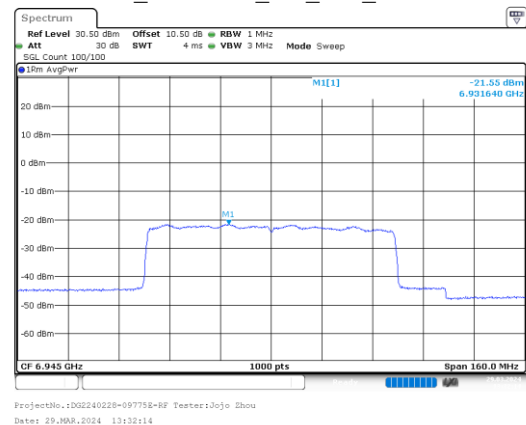
ax80_6945MHz_RU_Full_Chain 3
