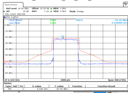
ax80_6545MHz_RU_Full_Chain 1
