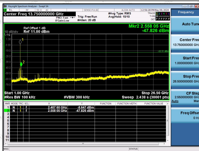
2.4G-Ant1-2408-1000~26500-PASS
