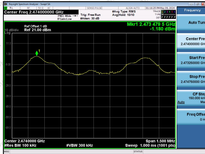
2.4G-Ant1-2474-0~Reference-PASS
