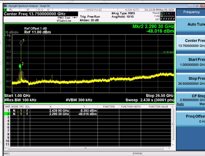
2.4G-Ant1-2440-1000~26500-PASS
