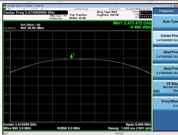
2.4G-Ant1-2474-PASS
