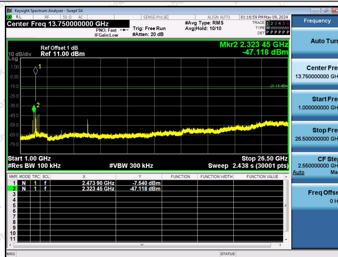
2.4G-Ant1-2474-1000~26500-PASS
