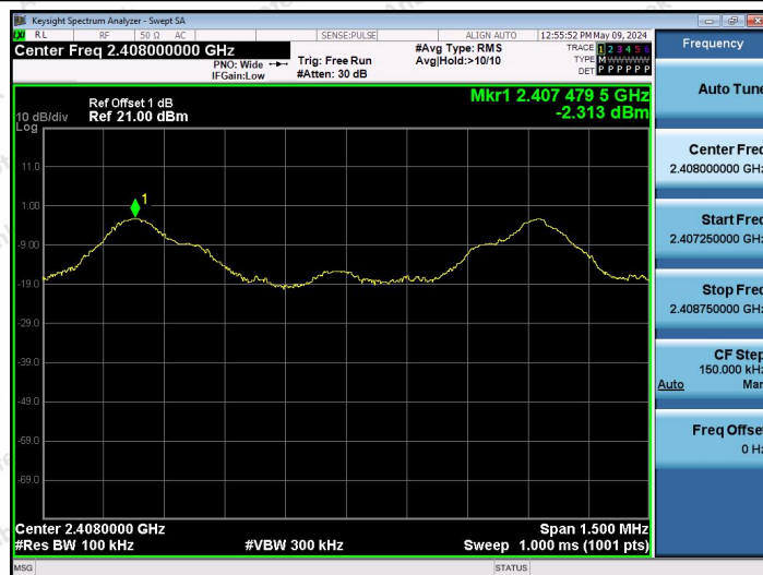
2.4G-Ant1-2408-0~Reference-PASS
