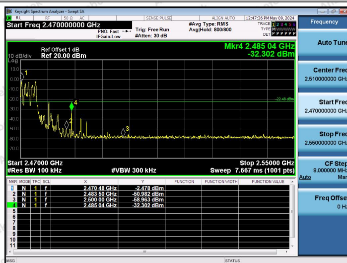
2.4G-Ant1-Hop_2474-PASS
