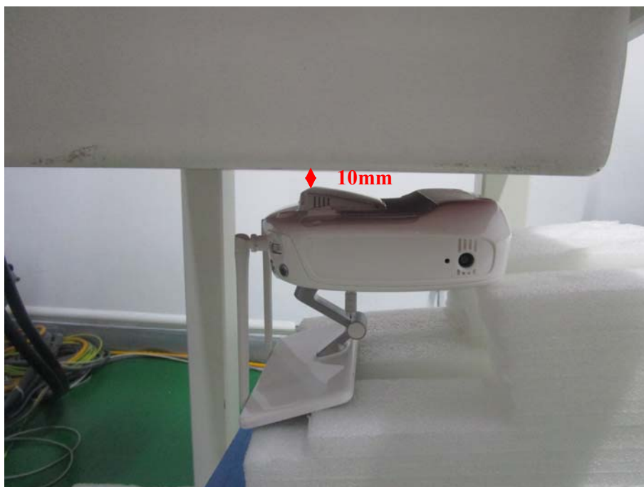
Test Position_Back Antenna Fold (10mm)
