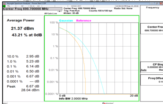
LTE_Band12_1_4MHz_16QAM_6_0_LowCH23017-699.7
