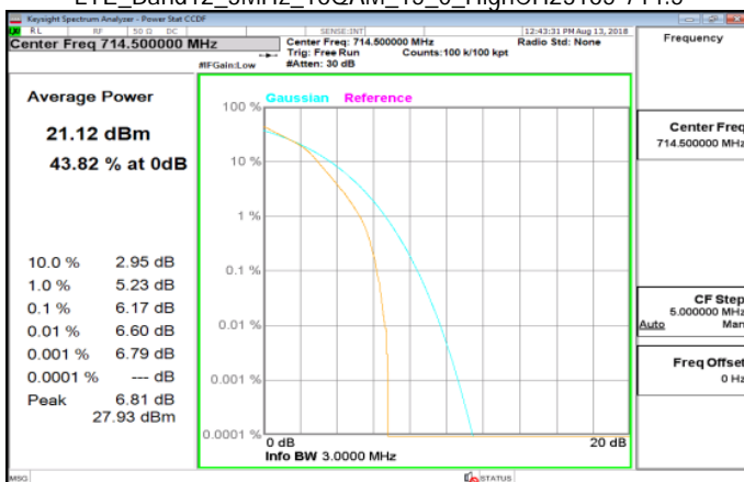
LTE_Band12_3MHz_16QAM_15_0_HighCH23165-714.5
