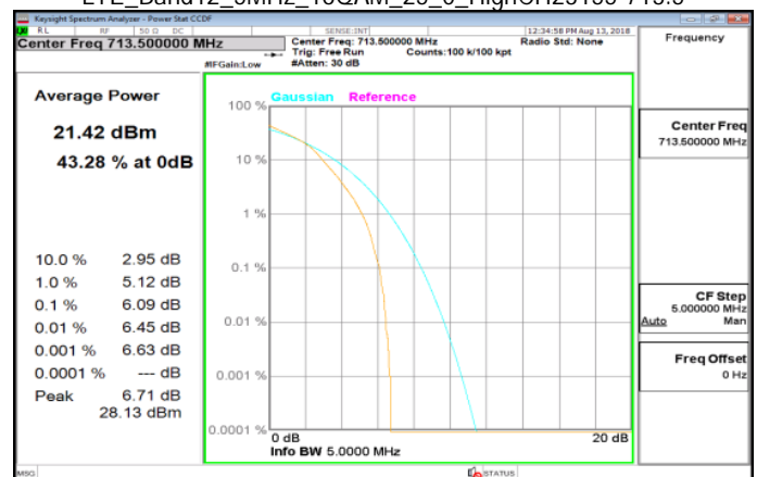
LTE_Band12_5MHz_16QAM_25_0_HighCH23155-713.5
