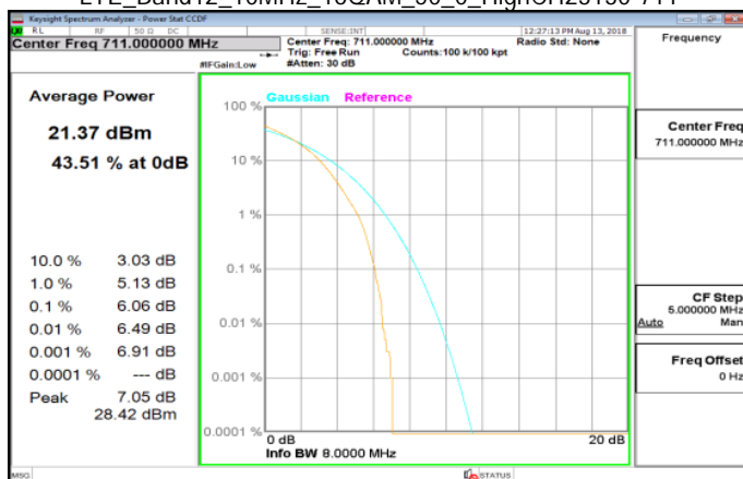
LTE_Band12_10MHz_16QAM_50_0_HighCH23130-711
