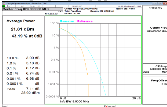
LTE_Band5_10MHz_16QAM_50_0_LowCH20450-829
