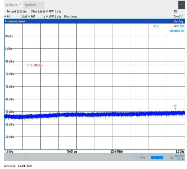
Band26(814-824)-10MHz-QPSK-26740-1RB#0-1000~3000-PASS
