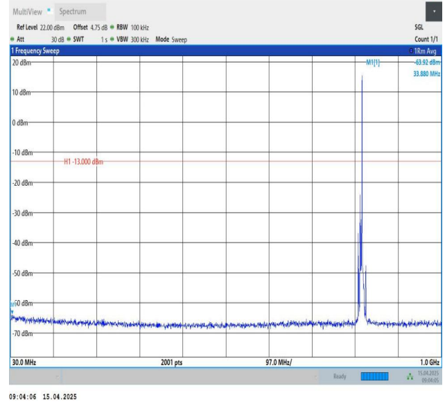
Band26(814-824)-5MHz-QPSK-26740-1RB#24-30~1000-PASS
