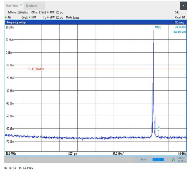
Band26(814-824)-5MHz-QPSK-26765-1RB#24-30~1000-PASS
