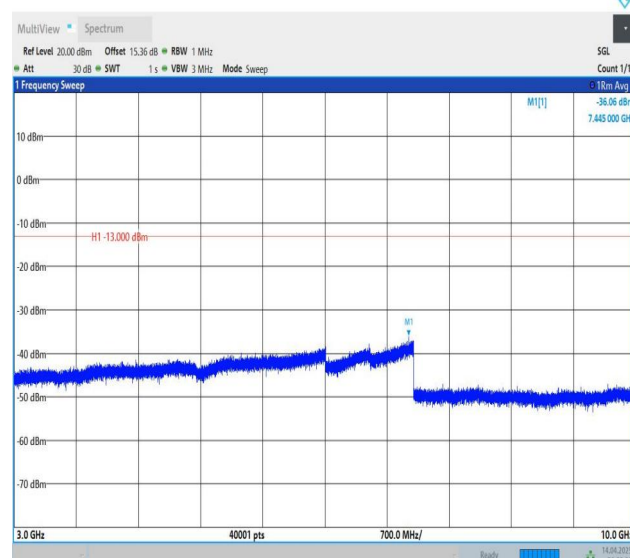
Band26(814-824)-10MHz-QPSK-26740-1RB#49-3000~10000-PAS
