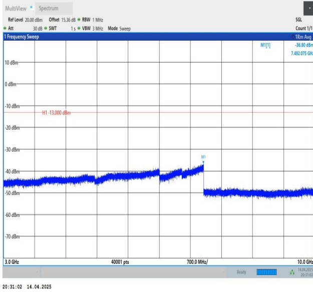
Band26(814-824)-5MHz-QPSK-26765-1RB#0-3000~10000-PASS
