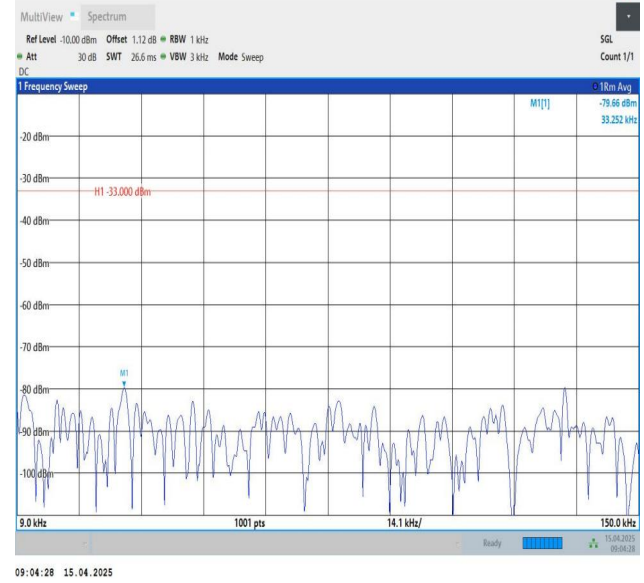
Band26(814-824)-5MHz-QPSK-26765-1RB#24-0.009~0.15-PASS
