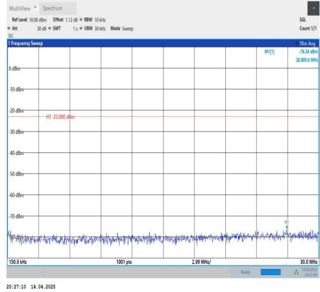
Band26(814-824)-3MHz-QPSK-26740-1RB#0-0.15~30-PASS
