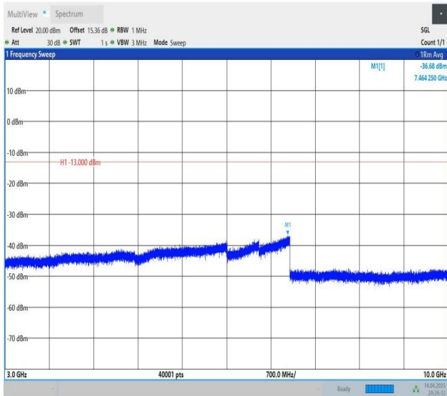
Band26(814-824)-3MHz-QPSK-26705-1RB#0-3000~10000-PASS
