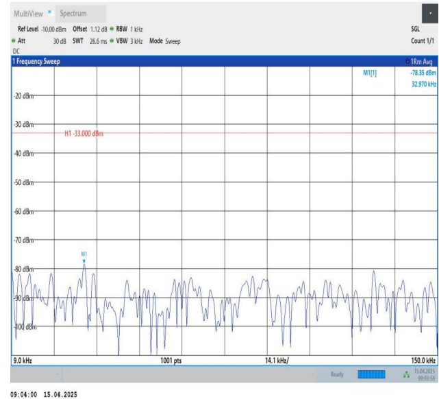
Band26(814-824)-5MHz-QPSK-26740-1RB#24-0.009~0.15-PASS
