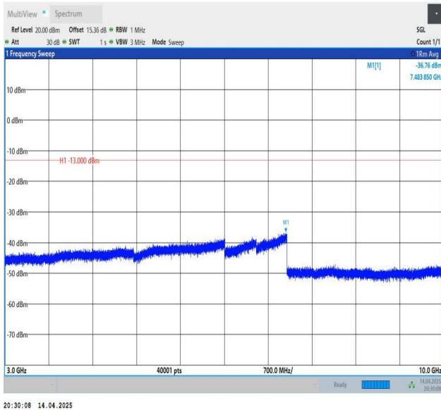
Band26(814-824)-5MHz-QPSK-26740-1RB#0-3000~10000-PASS
