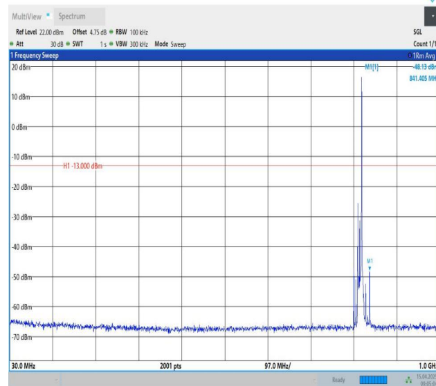
Band26(814-824)-10MHz-QPSK-26740-1RB#49-30~1000-PASS
