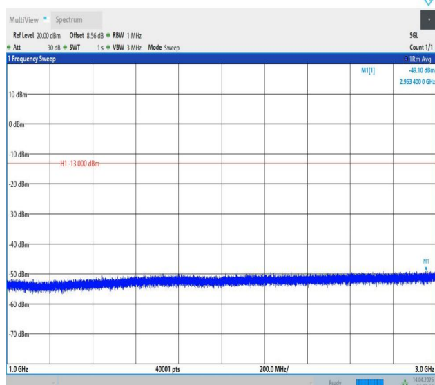
Band26(814-824)-10MHz-QPSK-26740-1RB#49-1000~3000-PAS
