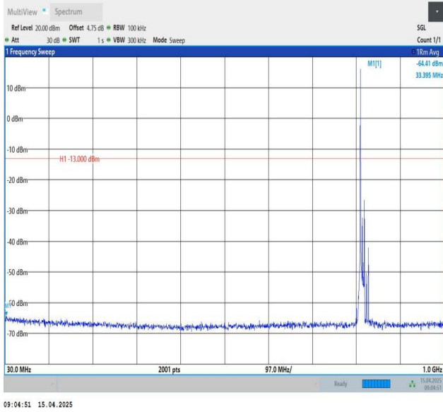
Band26(814-824)-10MHz-QPSK-26740-1RB#0-30~1000-PASS
