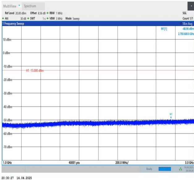
Band26(814-824)-5MHz-QPSK-26740-1RB#24-1000~3000-PASS
