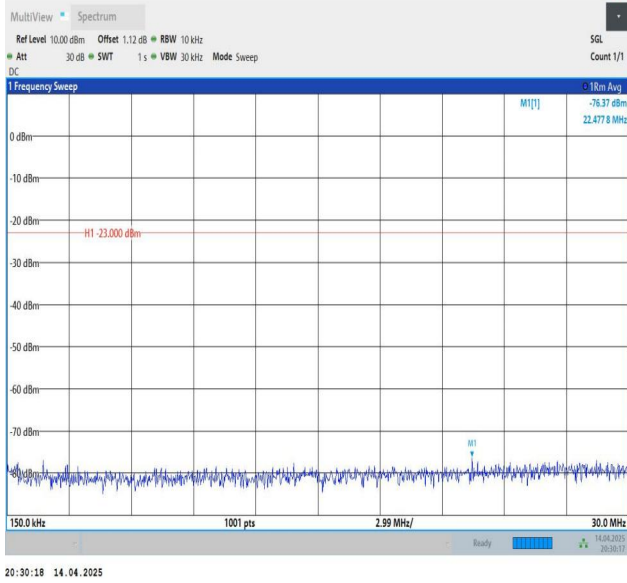
Band26(814-824)-5MHz-QPSK-26740-1RB#24-0.15~30-PASS
