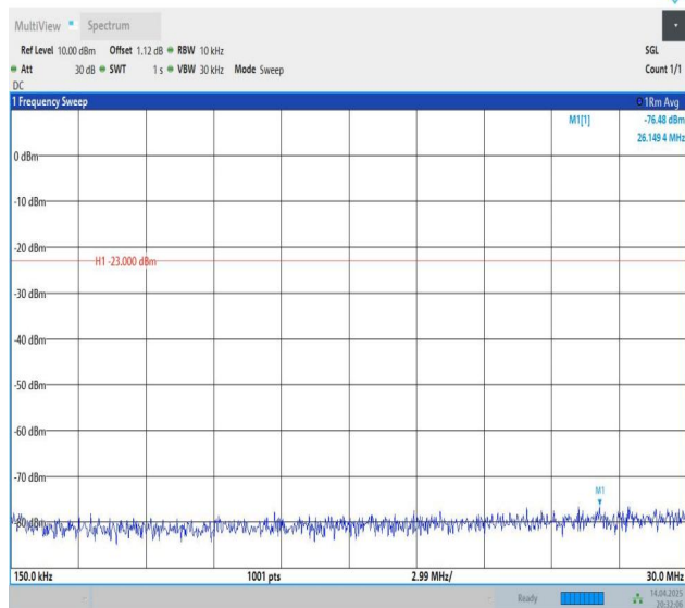
Band26(814-824)-10MHz-QPSK-26740-1RB#49-0.15~30-PASS
