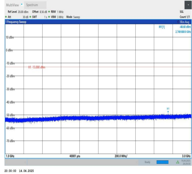
Band26(814-824)-5MHz-QPSK-26740-1RB#0-1000~3000-PASS
