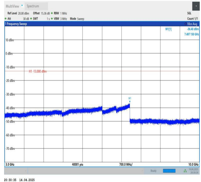
Band26(814-824)-5MHz-QPSK-26740-1RB#24-3000~10000-PASS
