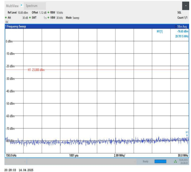
Band26(814-824)-3MHz-QPSK-26775-1RB#0-0.15~30-PASS
