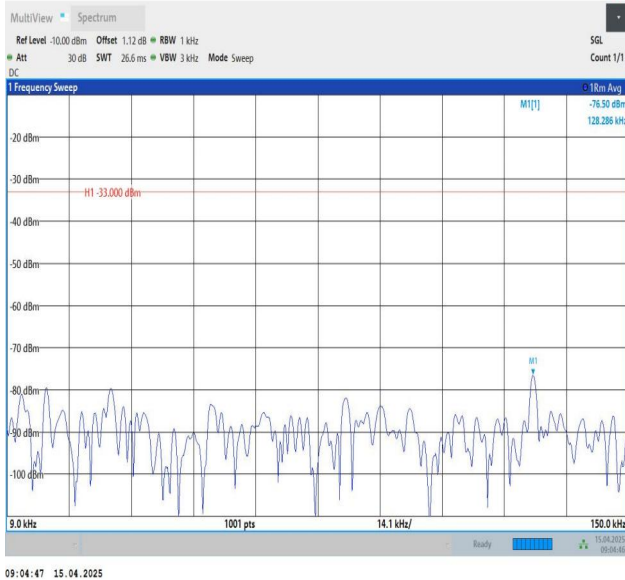
Band26(814-824)-10MHz-QPSK-26740-1RB#0-0.009~0.15-PASS
