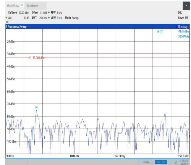
Band26(814-824)-3MHz-QPSK-26705-1RB#14-0.009~0.15-PASS
