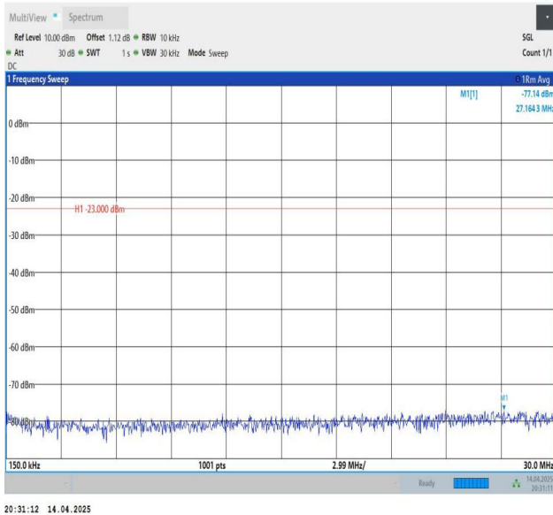
Band26(814-824)-5MHz-QPSK-26765-1RB#24-0.15~30-PASS
