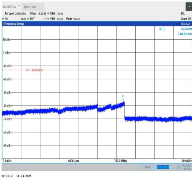
Band26(814-824)-10MHz-QPSK-26740-1RB#0-3000~10000-PAS
