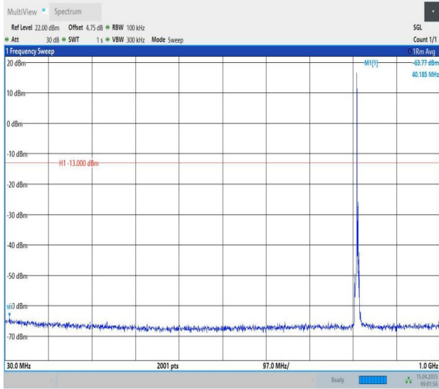
Band26(814-824)-3MHz-QPSK-26705-1RB#0-30~1000-PASS
