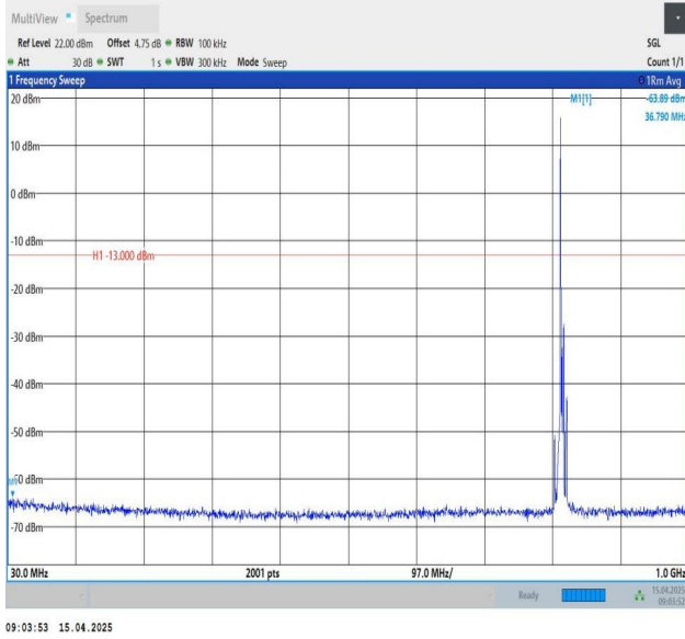
Band26(814-824)-5MHz-QPSK-26740-1RB#0-30~1000-PASS
