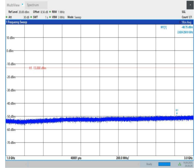
Band26(814-824)-3MHz-QPSK-26705-1RB#0-1000~3000-PASS
