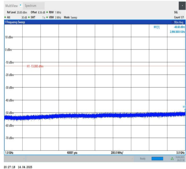
Band26(814-824)-3MHz-QPSK-26740-1RB#0-1000~3000-PASS
