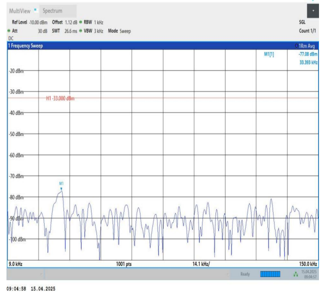
Band26(814-824)-10MHz-QPSK-26740-1RB#49-0.009~0.15-PASS
