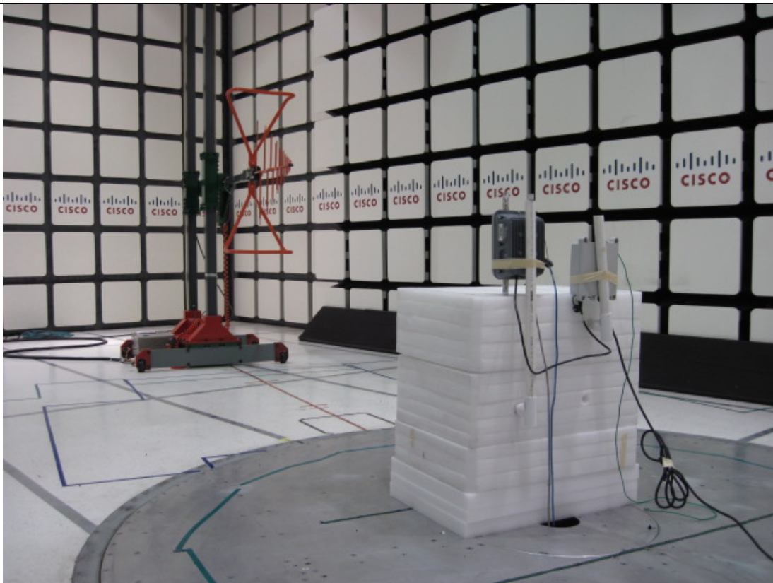
Title: Radiated Emissions 30-1000MHz Configuration Photograph
