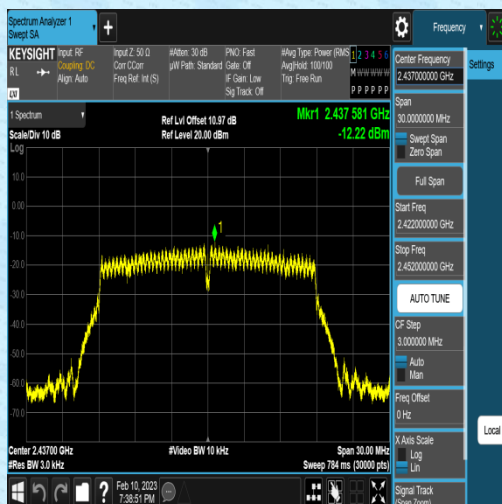
11N20MIMO-Ant1-2437--12.22-0.00-0.00-0.00
