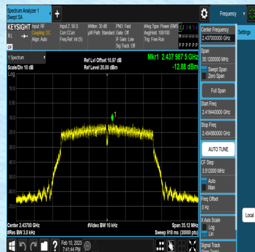
11N20MIMO-Ant2-2437--12.88-0.00-0.00-0.00
