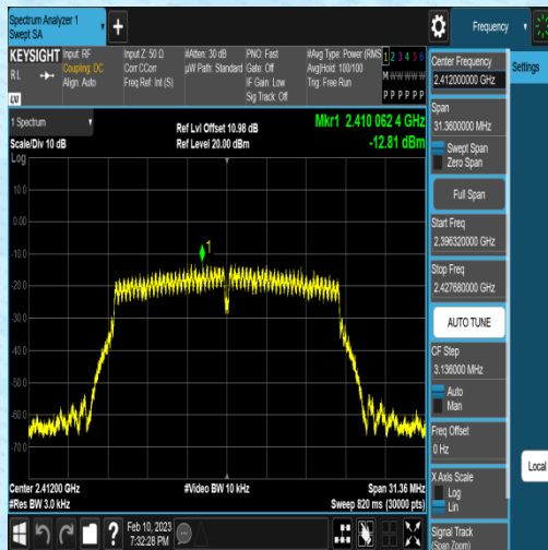
11N20MIMO-Ant1-2412--12.81-0.00-0.00-0.00
