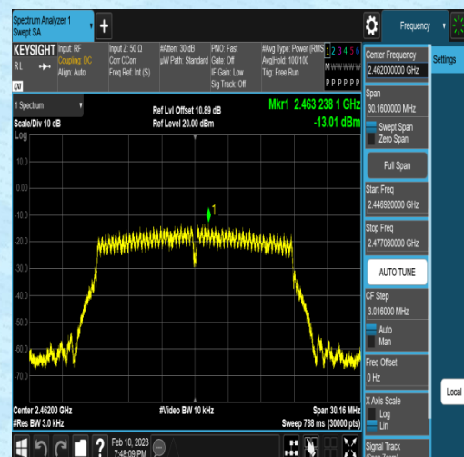
11N20MIMO-Ant2-2462--13.01-0.00-0.00-0.00
