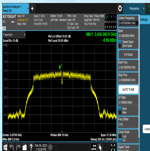
11G-Ant1-2437--8.86-0.00-0.00-0.00
