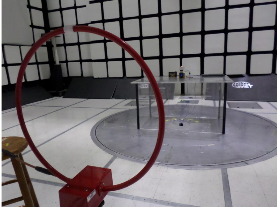
Photograph 5. Spurious Emissions, Outside the Bands, Loop Antenna View
