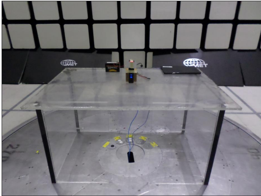
Photograph 1. Emissions Within the Band 13.553 – 14.01 MHz, Front View
