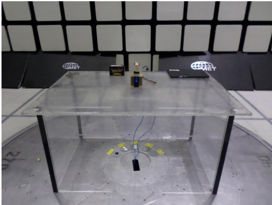
Photograph 4. Spurious Emissions, Outside the Bands, Front View
