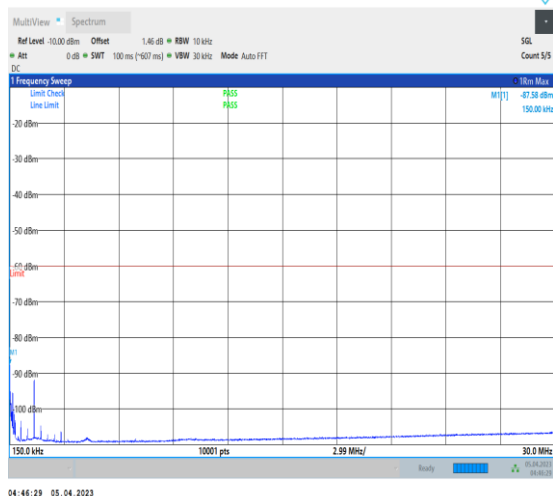
1-N48-PC3-30-40-M-1-DFT-PI2BPSK-Inner_1RB_Le ft-1@1-0.15-30-Ant0-0.15--87.58--60-PASS
