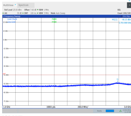
1-N48-30-40-H-1-DFT-QPSK-Edge_1RB_Left-1@0-100 0-3000-Ant0-2630.80--48.15--40-PASS
