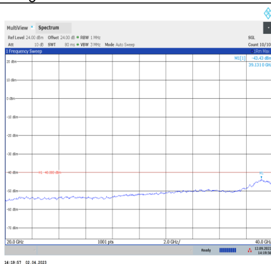
1-N48-PC3-30-40-H-1-DFT-PI2BPSK-Inner_1RB_Le ft-1@1-20000-40000-Ant0-61.62--54.53--50-PASS
