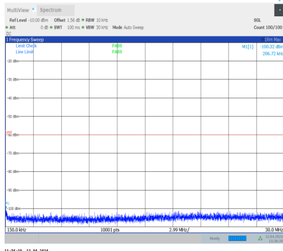
1-N48-30-40-H-1-DFT-QPSK-Edge_1RB_Left-1@0-0.1 5-30-Ant0-29.97--100.32--60-PASS
