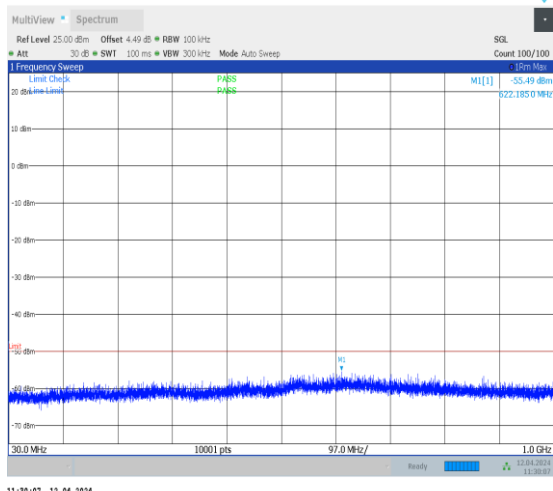
1-N48-30-40-M-1-DFT-QPSK-Edge_1RB_Left-1@ 0-30-1000-Ant0-33.88--55.49--50-PASS
