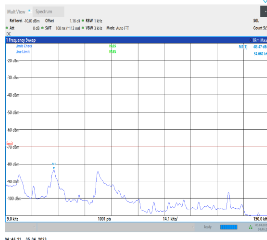
1-N48-PC3-30-40-M-1-DFT-PI2BPSK-Inner_1RB_Lef t-1@1-0.009-0.15-Ant0-0.02--83.47--70-PASS
