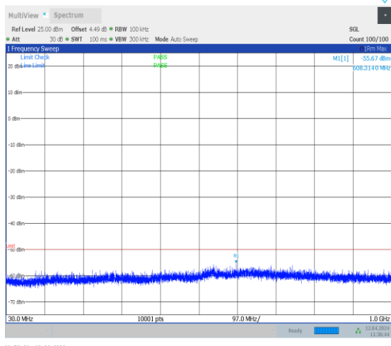
1-N48-30-40-H-1-DFT-QPSK-Edge_1RB_Left-1@ 0-30-1000-Ant0-35.72--55.67--50-PASS
