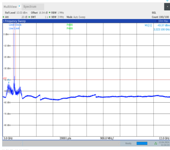
1-N48-30-40-M-1-DFT-QPSK-Edge_1RB_Left-1@ 0-3000-12000-Ant0-3317.25--43.37--40-PASS
