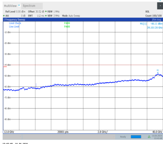
1-N48-PC3-30-40-L-1-DFT-PI2BPSK-Inner_1RB_Left-1 @1-12000-40000-Ant0-12000.00--48.12--40-PASS
