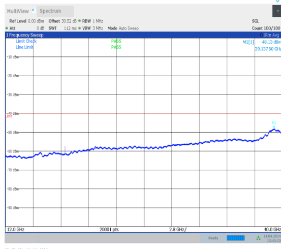
1-N48-PC3-30-40-M-1-DFT-PI2BPSK-Inner_1RB_Left- 1@1-12000-40000-Ant0-12000.00--48.12--40-PASS
