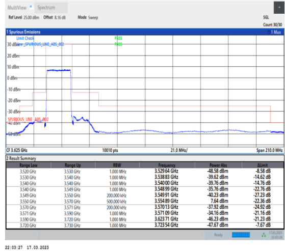
1-N48-PC3-30-20-L-3-DFT-PI2BPSK-Outer_Full-50@0-Ant0-1--PASS-see graph
