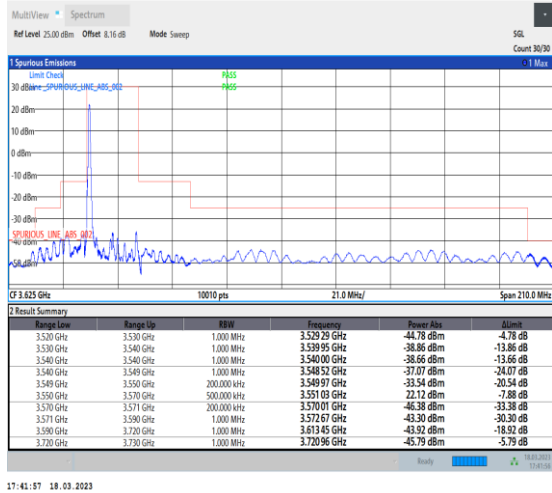
1-N48-PC3-30-20-L-1-DFT-PI2BPSK-Edge_1RB_Left-1@0-Ant0-1--PASS-see graph
