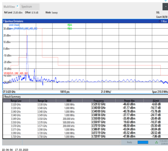
1-N48-PC3-30-20-L-4-CP-QPSK-Edge_1RB_Left-1@0-Ant0-1--PASS-see graph
