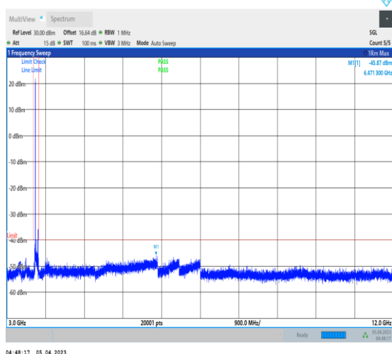
1-N48-PC3-30-40-H-1-DFT-PI2BPSK-Inner_1RB_Le ft-1@1-3000-12000-Ant0-3368.55--45.87--40-PASS
