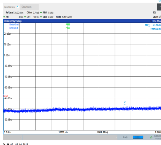
1-N48-PC3-30-40-L-1-DFT-PI2BPSK-Inner_1RB_Lef t-1@1-1000-3000-Ant0-2998.40--47.20--40-PASS
