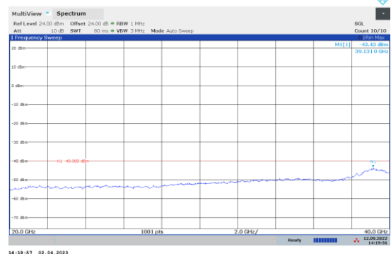
1-N48-PC3-30-40-L-1-DFT-PI2BPSK-Inner_1RB_Lef t-1@1-20000-40000-Ant0-3197.55--44.44--40-PASS
