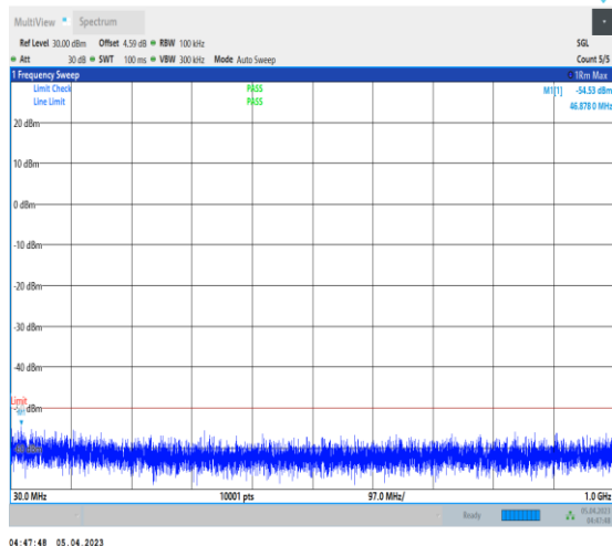
1-N48-PC3-30-40-H-1-DFT-PI2BPSK-Inner_1RB_Le ft-1@1-30-1000-Ant0-61.62--54.53--50-PASS
