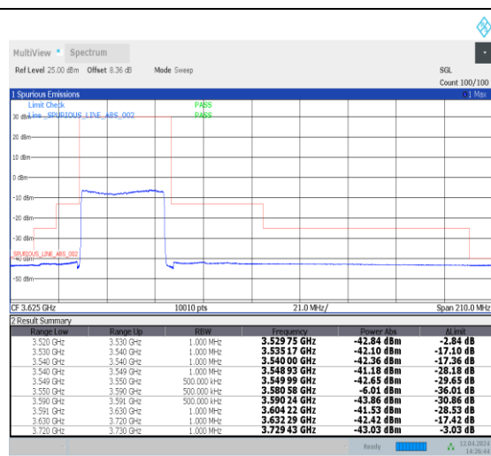
1-N48-30-40-L-3-DFT-PI2BPSK-Outer_Full-100@0-Ant0-1--PASS-see graph
