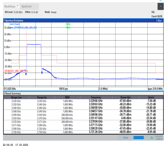
1-N48-PC3-30-20-L-6-CP-QPSK-Outer_Full-51@0-Ant0-1--PASS-see graph
