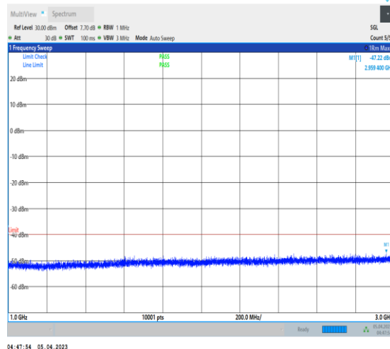
1-N48-PC3-30-40-H-1-DFT-PI2BPSK-Inner_1RB_Le ft-1@1-1000-3000-Ant0-2996.80--47.22--40-PASS
