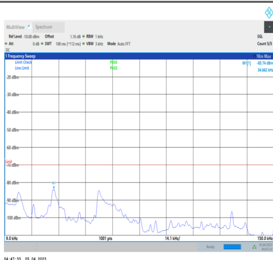
1-N48-PC3-30-40-H-1-DFT-PI2BPSK-Inner_1RB_Le ft-1@1-0.009-0.15-Ant0-0.06--83.74--70-PASS
