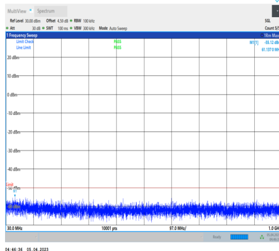
1-N48-PC3-30-40-M-1-DFT-PI2BPSK-Inner_1RB_Le ft-1@1-30-1000-Ant0-45.13--55.12--50-PASS
