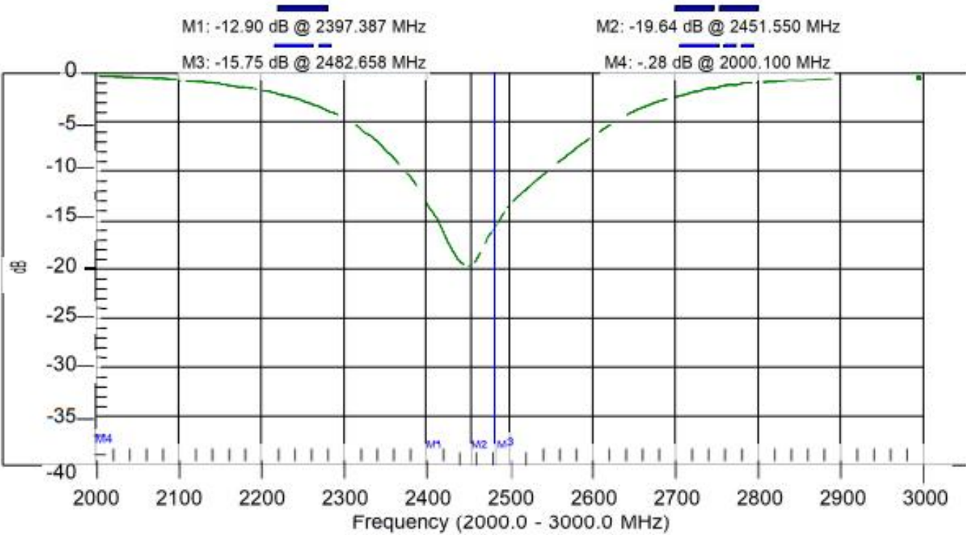
Return Loss
