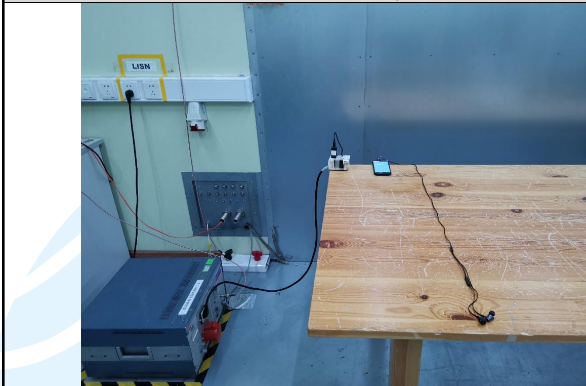
Conducted Emission Test Setup-3 - Mode 1
