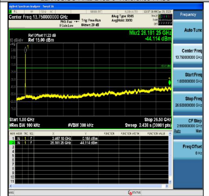
11N40SISO-Ant1-2452-1000-26500-PASS
