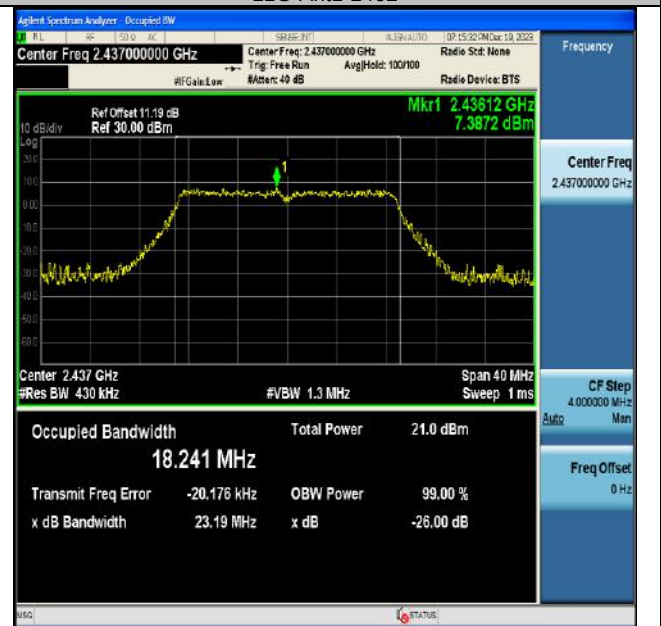
11N20SISO-Ant1-2437
