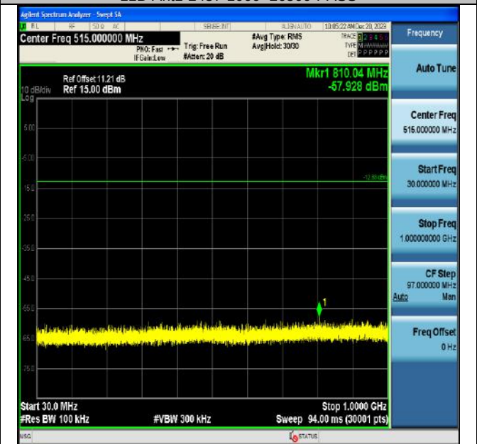
11B-Ant1-2462-30-1000-PASS
