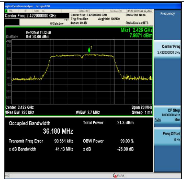
11N40SISO-Ant1-2422
