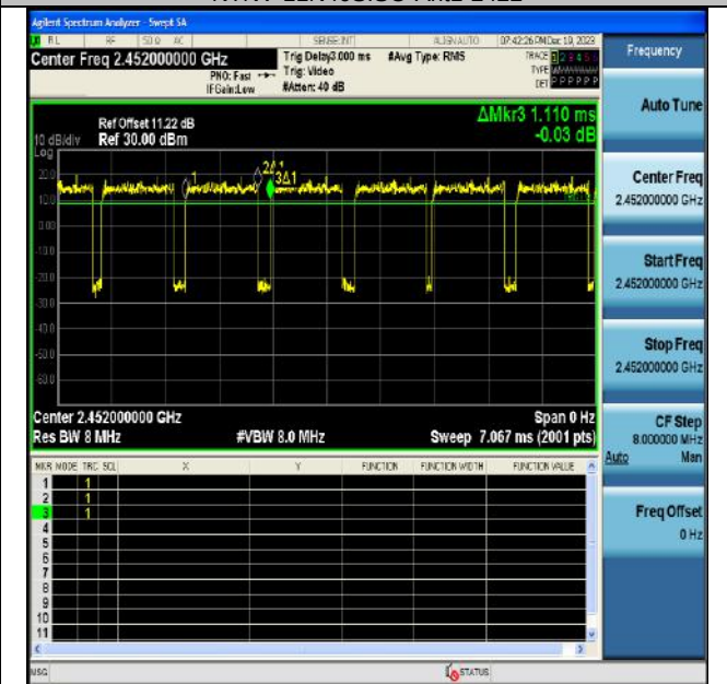
NTVN-11N40SISO-Ant1-2452
