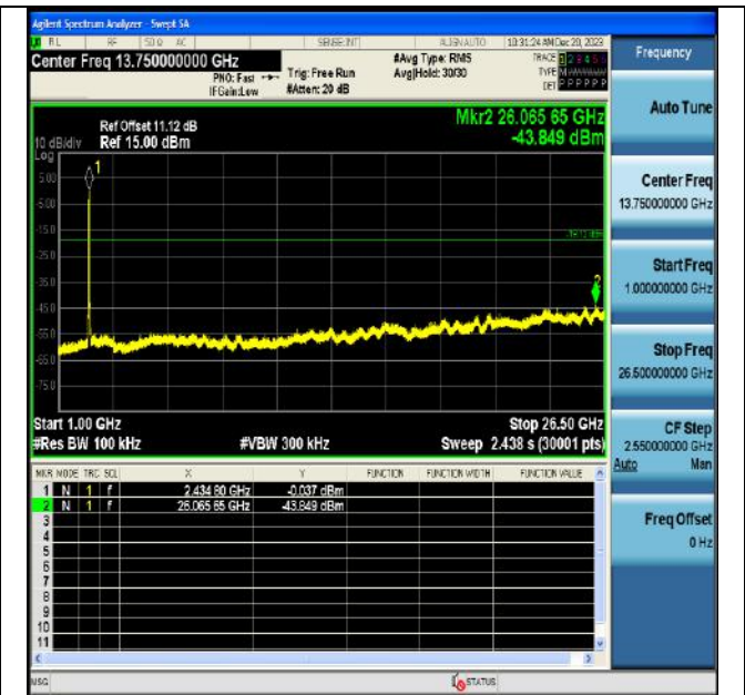
11N40SISO-Ant1-2422-1000~26500-PASS
