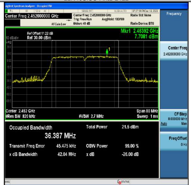
11N40SISO-Ant1-2452
