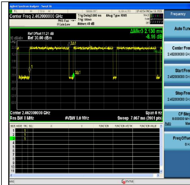
NTVN-11N20SISO-Ant1-2462
