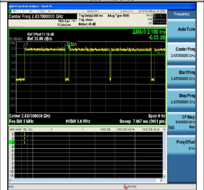
NTNV-11N20SISO-Ant1-2437
