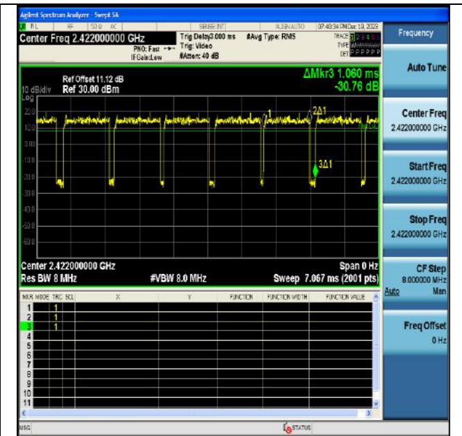
NTVN-11N40SISO-Ant1-2422
