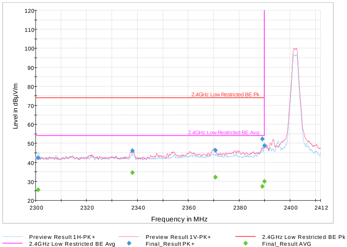
Plot 20. 2402 MHz, 2Mbps Lower Band Edge, Restricted
