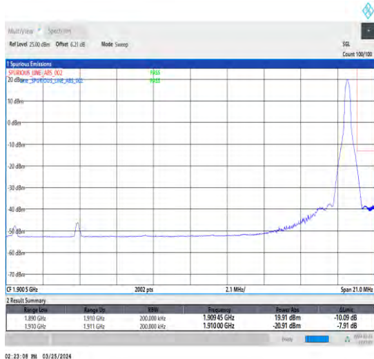
1-N2-15-20-H-5-CP-QPSK-Edge_1RB_Right-1@105-Ant1-1-seegraph-PASS-see graph
