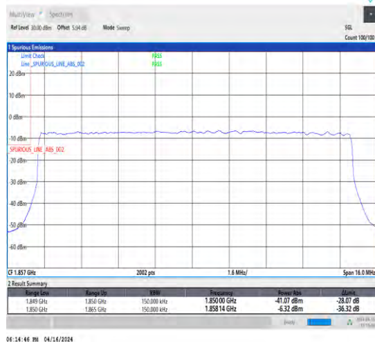
1-N2-15-15-L-3-DFT-PI2BPSK-Outer_Full-75@0-Ant1-1-seegraph-PASS-see graph
