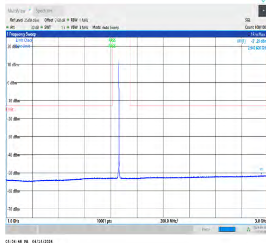
1-N2-15-40-M-1-DFT-QPSK-Edge_1RB_Left-1@0-10 00-3000-Ant1-2949.60--51.29--13-PASS
