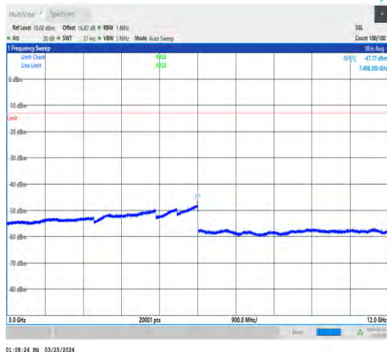
1-N2-15-40-L-1-DFT-PI2BPSK-Inner_1RB_Left-1@ 1-3000-12000-Ant1-7428.45--47.77--13-PASS
