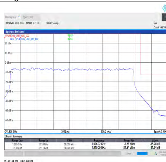
1-N2-15-5-H-3-DFT-PI2BPSK-Outer_Full-25@0-Ant1-1-seegraph-PASS-see graph
