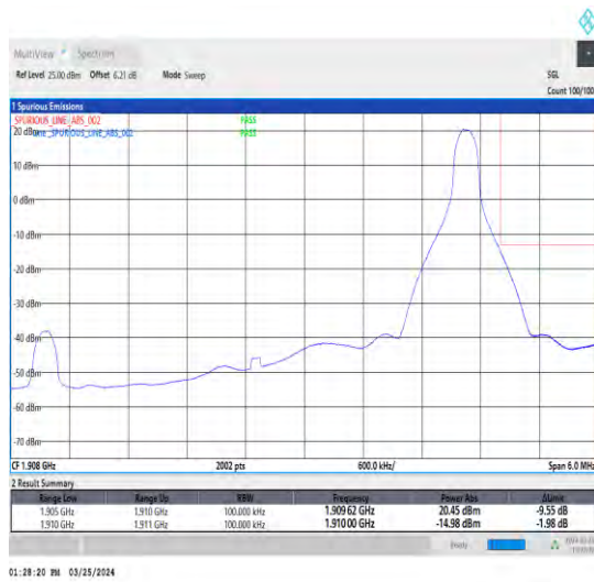
1-N2-15-5-H-2-DFT-PI2BPSK-Edge_1RB_Right-1@24-Ant1-1-seegraph-PASS-see graph
