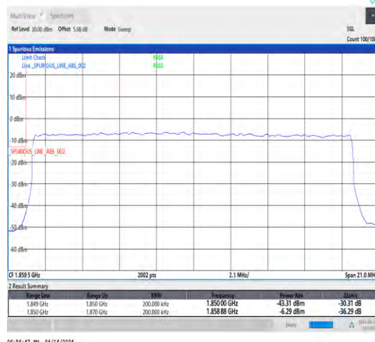
1-N2-15-20-L-3-DFT-PI2BPSK-Outer_Full-100@0-Ant1-1-seegraph-PASS-see graph
