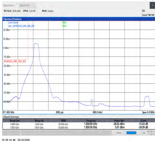
1-N2-15-5-L-1-DFT-PI2BPSK-Edge_1RB_Left-1@0-Ant1-1-seegraph-PASS-see graph
