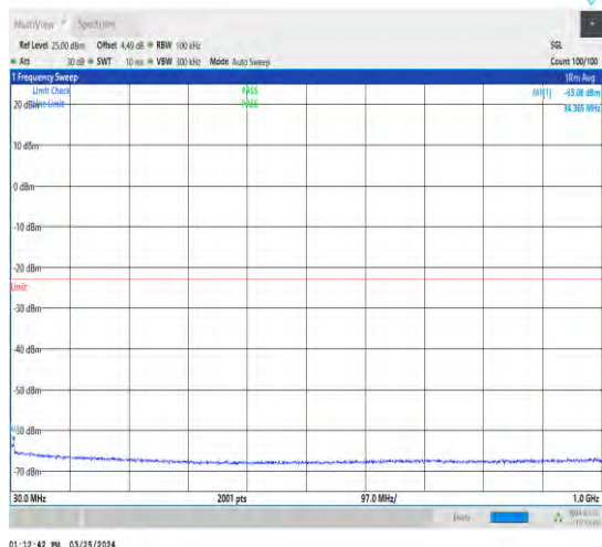
1-N2-15-40-H-1-DFT-PI2BPSK-Inner_1RB_Left-1@ 1-30-1000-Ant1-34.37--63.08--23-PASS
