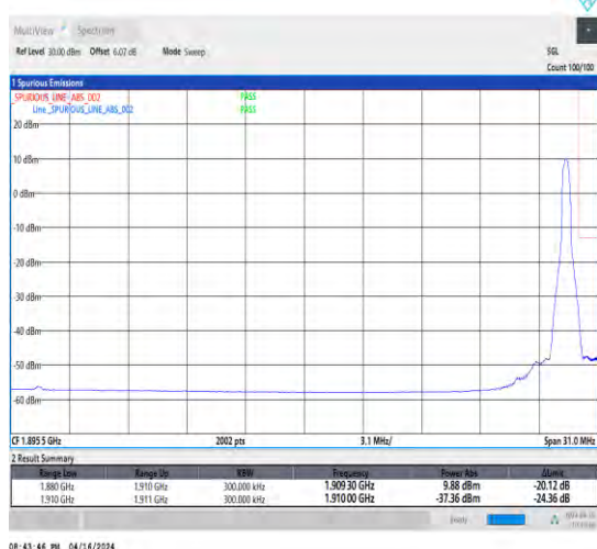
1-N2-15-30-H-5-CP-QPSK-Edge_1RB_Right-1@159-Ant1-1-seegraph-PASS-see graph
