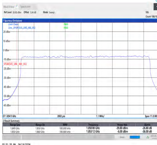
1-N2-15-10-L-3-DFT-PI2BPSK-Outer_Full-50@0-Ant1-1-seegraph-PASS-see graph
