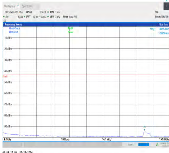
1-N2-15-40-M-1-DFT-PI2BPSK-Inner_1RB_Left-1@ 1-0.009-0.15-Ant1-0.13--93.96--43-PASS
