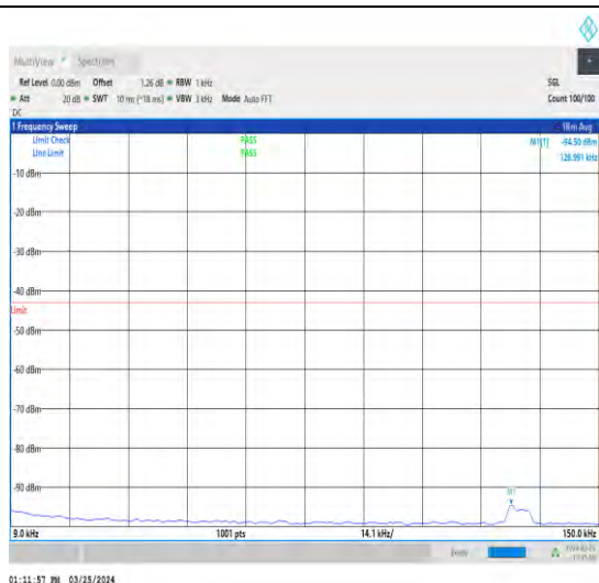
1-N2-15-40-H-1-DFT-PI2BPSK-Inner_1RB_Left-1@ 1-0.009-0.15-Ant1-0.13--94.50--43-PASS
