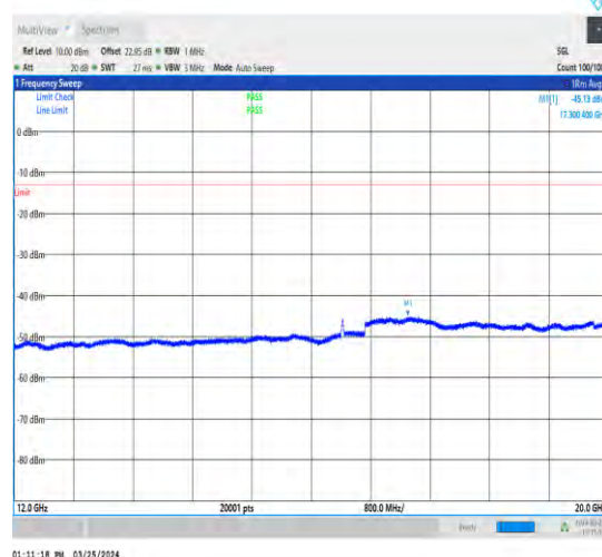
1-N2-15-40-M-1-DFT-PI2BPSK-Inner_1RB_Left-1@ 1-12000-20000-Ant1-17460.40--45.13--13-PASS
