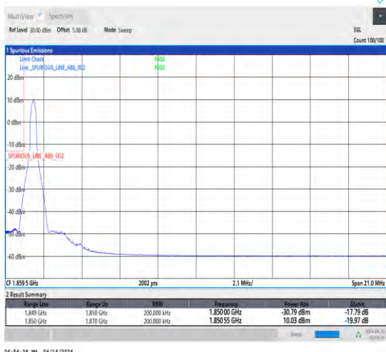
1-N2-15-20-L-1-DFT-PI2BPSK-Edge_1RB_Left-1@0-Ant1-1-seegraph-PASS-see graph
