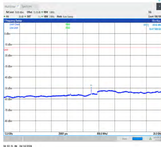
1-N2-15-40-L-1-DFT-QPSK-Edge_1RB_Left-1@0-12 000-20000-Ant1-16417.60--50.92--13-PASS
