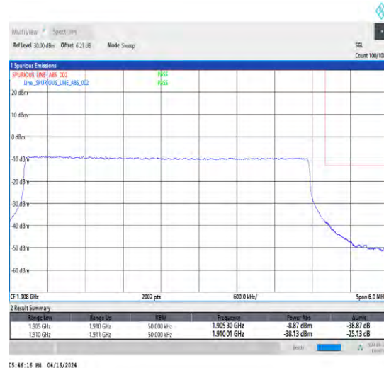
1-N2-15-5-H-6-CP-QPSK-Outer_Full-25@0-Ant1-1-seegraph-PASS-see graph
