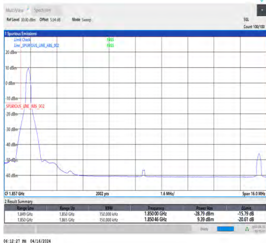
1-N2-15-15-L-1-DFT-PI2BPSK-Edge_1RB_Left-1@0-Ant1-1-seegraph-PASS-see graph
