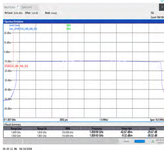
1-N2-15-15-L-6-CP-QPSK-Outer_Full-79@0-Ant1-1-seegraph-PASS-see graph
