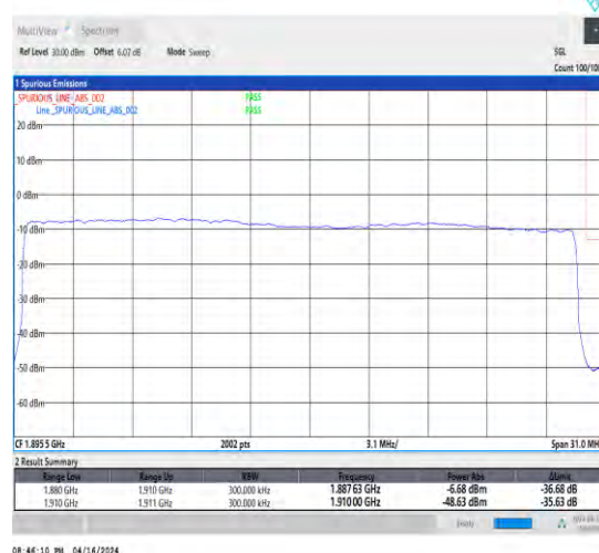
1-N2-15-30-H-6-CP-QPSK-Outer_Full-160@0-Ant1-1-seegraph-PASS-see graph
