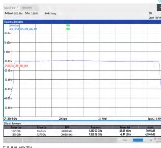
1-N2-15-20-L-6-CP-QPSK-Outer_Full-106@0-Ant1-1-seegraph-PASS-see graph
