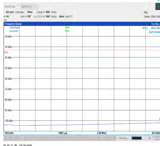
1-N2-15-40-M-1-DFT-QPSK-Edge_1RB_Left-1@0-0. 15-30-Ant1-29.87--102.01--33-PASS
