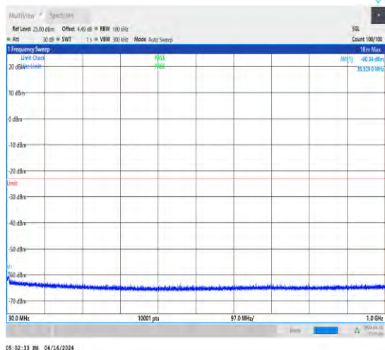
1-N2-15-40-M-1-DFT-QPSK-Edge_1RB_Left-1@0-3 0-1000-Ant1-35.53--60.34--23-PASS
