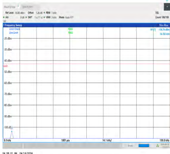
1-N2-15-40-M-1-DFT-QPSK-Edge_1RB_Left-1@0-0 .009-0.15-Ant1-0.02--104.74--43-PASS
