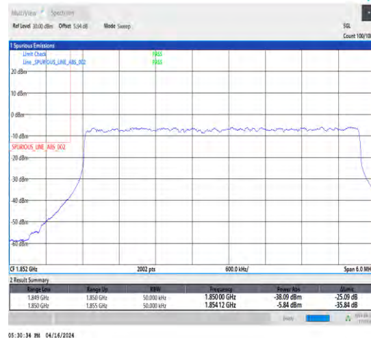
1-N2-15-5-L-3-DFT-PI2BPSK-Outer_Full-25@0-Ant1-1-seegraph-PASS-see graph
