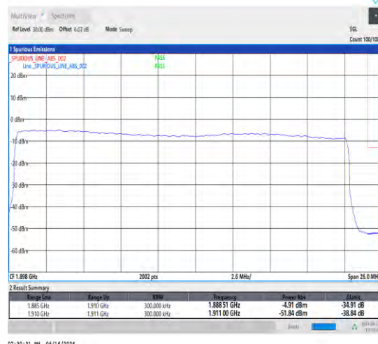
1-N2-15-25-H-3-DFT-PI2BPSK-Outer_Full-128@0-Ant1-1-seegraph-PASS-see graph
