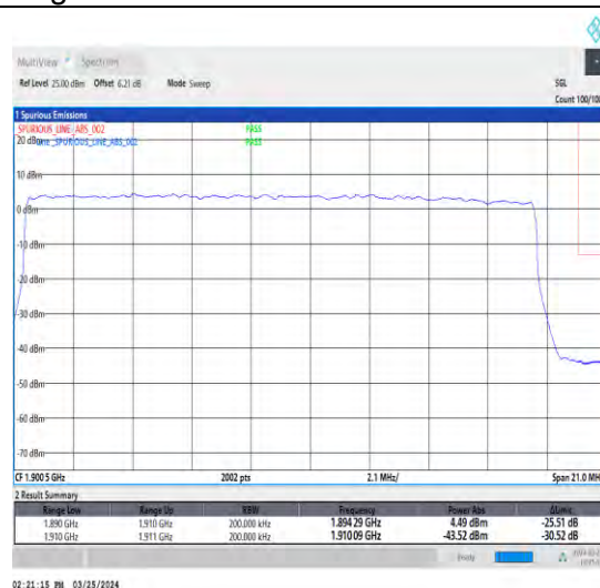
1-N2-15-20-H-3-DFT-PI2BPSK-Outer_Full-100@0-Ant1-1-seegraph-PASS-see graph
