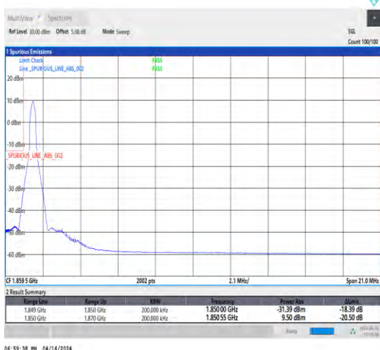
1-N2-15-20-L-4-CP-QPSK-Edge_1RB_Left-1@0-Ant1-1-seegraph-PASS-see graph
