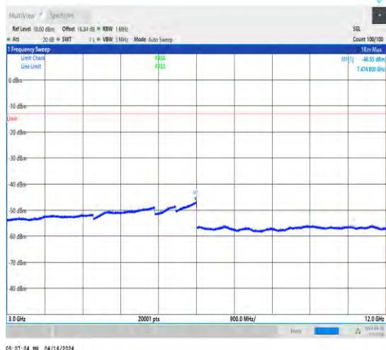
1-N2-15-40-M-1-DFT-QPSK-Edge_1RB_Left-1@0-3 000-12000-Ant1-7474.80--46.55--13-PASS
