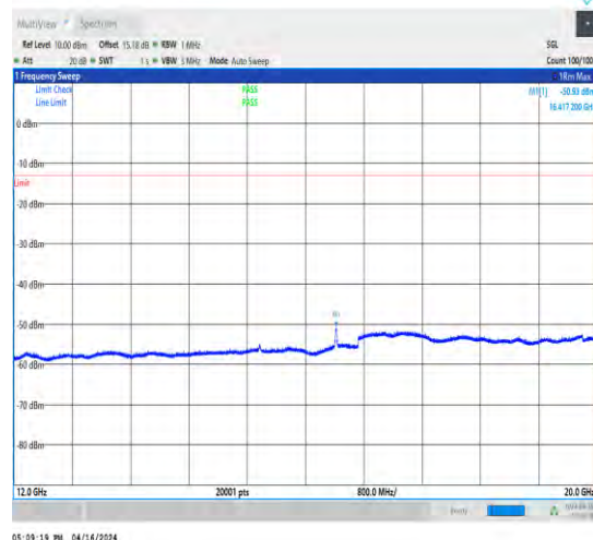
1-N2-15-40-M-1-DFT-QPSK-Edge_1RB_Left-1@0-12 000-20000-Ant1-16417.20--50.93--13-PASS
