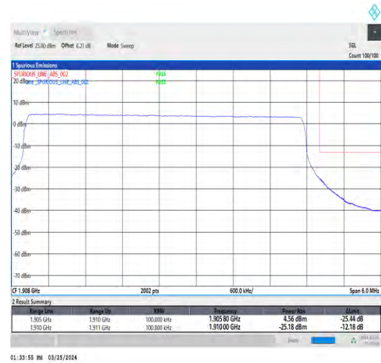
1-N2-15-5-H-6-CP-QPSK-Outer_Full-25@0-Ant1-1-seegraph-PASS-see graph
