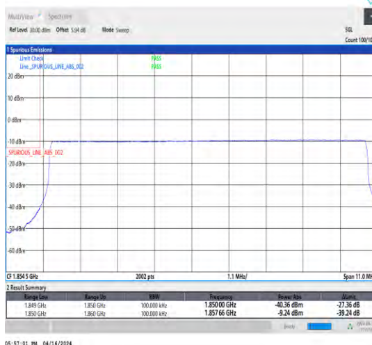
1-N2-15-10-L-6-CP-QPSK-Outer_Full-52@0-Ant1-1-seegraph-PASS-see graph
