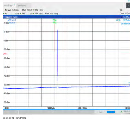
1-N2-15-40-L-1-DFT-QPSK-Edge_1RB_Left-1@0-10 00-3000-Ant1-2975.60--51.35--13-PASS
