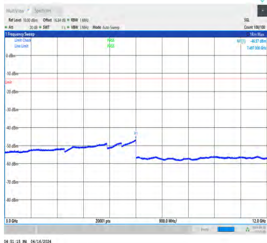
1-N2-15-40-L-1-DFT-QPSK-Edge_1RB_Left-1@0-3 000-12000-Ant1-7497.30--46.57--13-PASS
