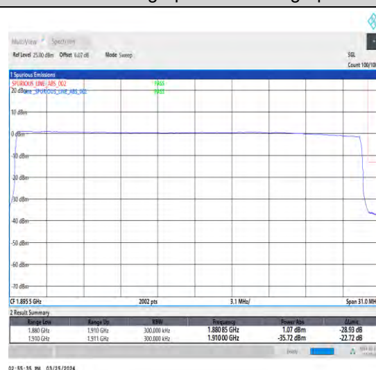
1-N2-15-30-H-6-CP-QPSK-Outer_Full-160@0-Ant1-1-seegraph-PASS-see graph
