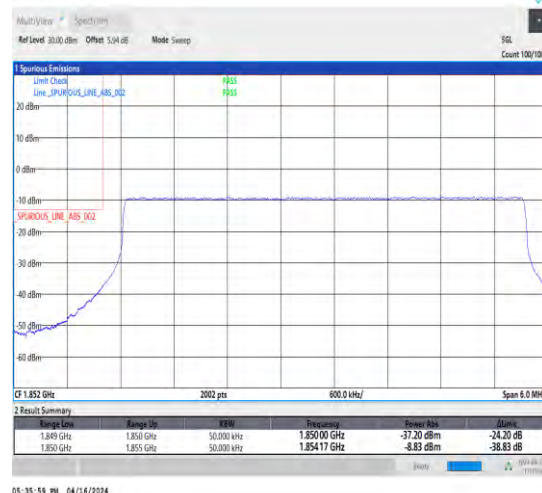
1-N2-15-5-L-6-CP-QPSK-Outer_Full-25@0-Ant1-1-seegraph-PASS-see graph
