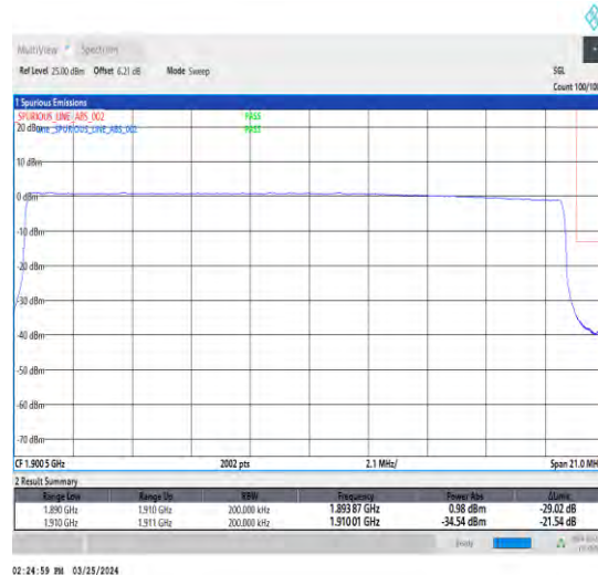
1-N2-15-20-H-6-CP-QPSK-Outer_Full-106@0-Ant1-1-seegraph-PASS-see graph
