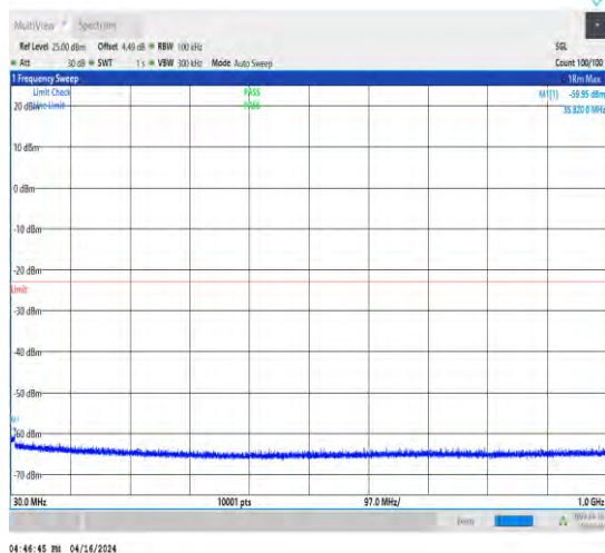
1-N2-15-40-L-1-DFT-QPSK-Edge_1RB_Left-1@0-3 0-1000-Ant1-35.82--59.95--23-PASS
