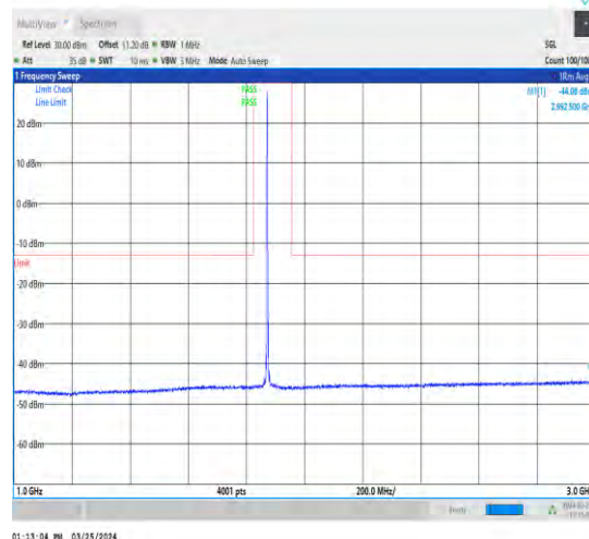
1-N2-15-40-H-1-DFT-PI2BPSK-Inner_1RB_Left-1@ 1-1000-3000-Ant1-2992.50--44.08--13-PASS
