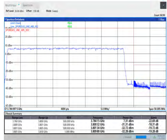
1-N78-3700-3800-PC2-30-40-H-3-DFT-PI2BPSK-Outer_Full-100@0-Ant1-PASS-see graph
