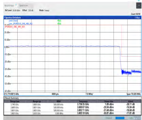
1-N78-3700-3800-PC2-30-60-H-6-CP-QPSK-Outer_Full-162@0-Ant1-PASS-see graph
