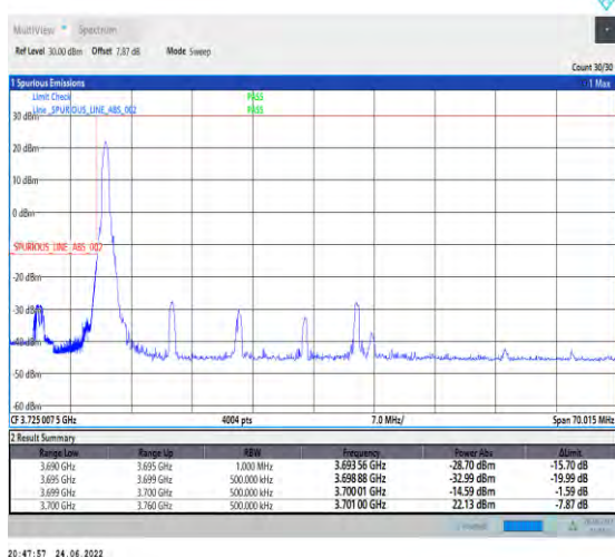
1-N78-3700-3800-PC2-30-60-L-4-CP-QPSK-Edge_1RB_Left-1@0-Ant1-PASS-see graph
