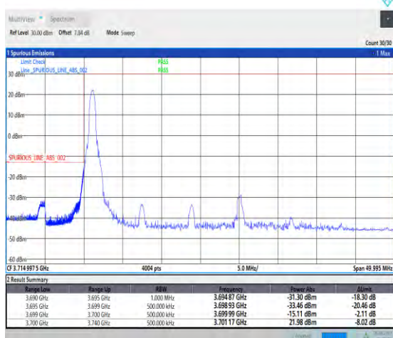
1-N78-3700-3800-PC2-30-40-L-4-CP-QPSK-Edge_1RB_Left-1@0-Ant1-PASS-see graph
