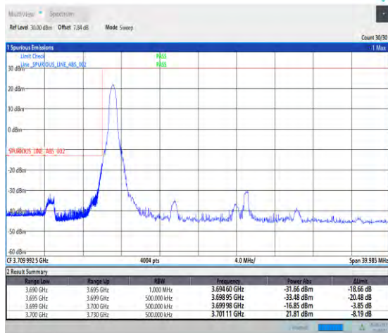
1-N78-3700-3800-PC2-30-30-L-4-CP-QPSK-Edge_1RB_Left-1@0-Ant1-PASS-see graph
