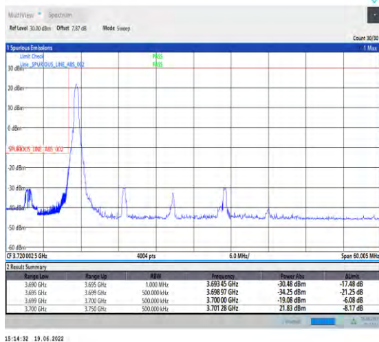
1-N78-3700-3800-PC2-30-50-L-4-CP-QPSK-Edge_1RB_Left-1@0-Ant1-PASS-see graph
