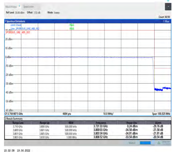
1-N78-3700-3800-PC2-30-90-H-6-CP-QPSK-Outer_Full-245@0-Ant1-PASS-see graph
