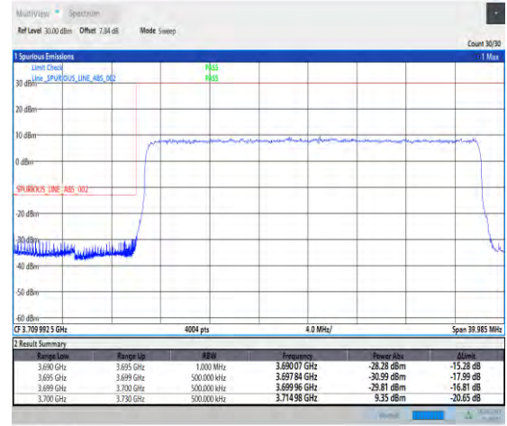
1-N78-3700-3800-PC2-30-30-L-3-DFT-PI2BPSK-Outer_Full-75@0-Ant1-PASS-see graph
