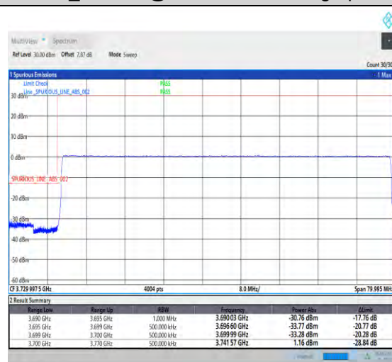
1-N78-3700-3800-PC2-30-70-L-3-DFT-PI2BPSK-Outer_Full-180@0-Ant1-PASS-see graph
