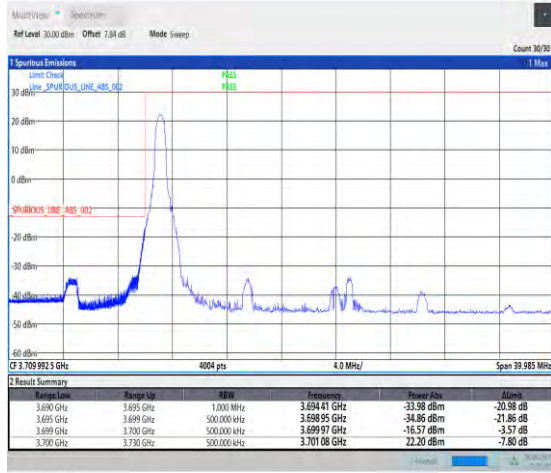
1-N78-3700-3800-PC2-30-30-L-1-DFT-PI2BPSK-Edge_1RB_Left-1@0-Ant1-PASS-see graph
