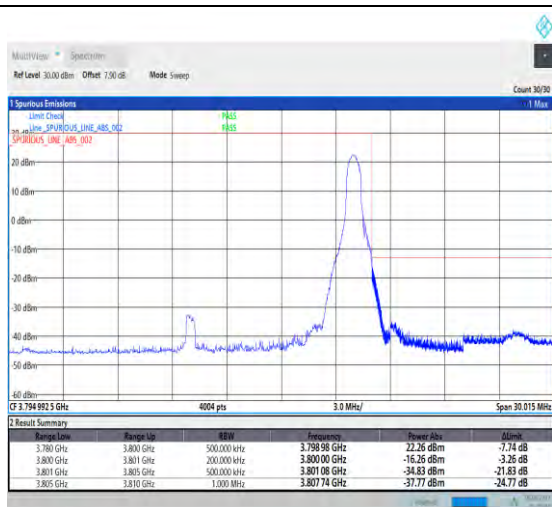
1-N78-3700-3800-PC2-30-20-H-2-DFT-PI2BPSK-Edge_1RB_Right-1@50-Ant1-PASS-see graph
