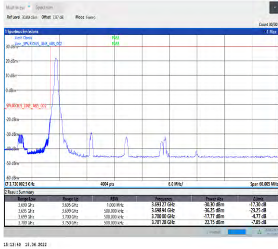
1-N78-3700-3800-PC2-30-50-L-1-DFT-PI2BPSK-Edge_1RB_Left-1@0-Ant1-PASS-see graph
