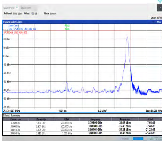
1-N78-3700-3800-PC2-30-40-H-5-CP-QPSK-Edge_1RB_Right-1@105-Ant1-PASS-see graph
