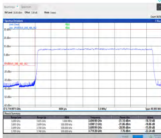
1-N78-3700-3800-PC2-30-40-L-3-DFT-PI2BPSK-Outer_Full-100@0-Ant1-PASS-see graph
