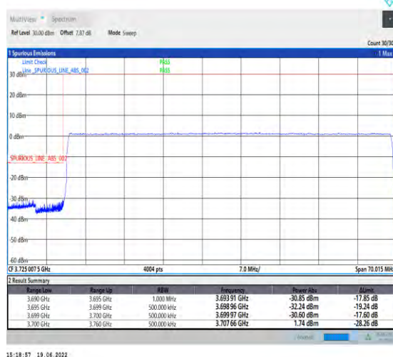
1-N78-3700-3800-PC2-30-60-L-6-CP-QPSK-Outer_Full-162@0-Ant1-PASS-see graph
