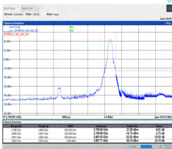
1-N78-3700-3800-PC2-30-20-H-5-CP-QPSK-Edge_1RB_Right-1@50-Ant1-PASS-see graph
