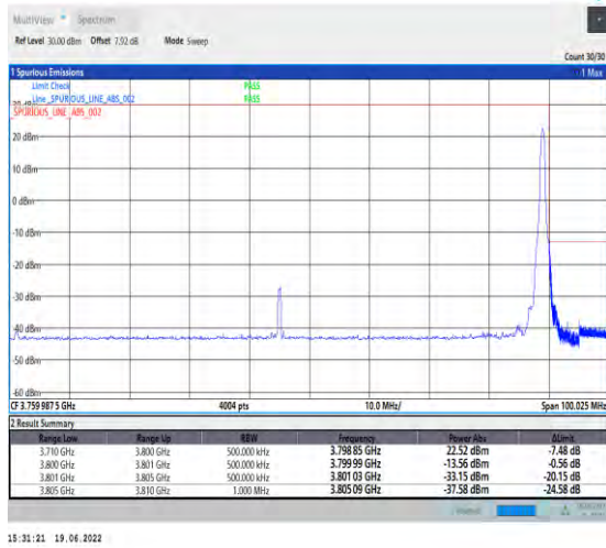
1-N78-3700-3800-PC2-30-90-H-2-DFT-PI2BPSK-Edge_1RB_Right-1@244-Ant1-PASS-see graph
