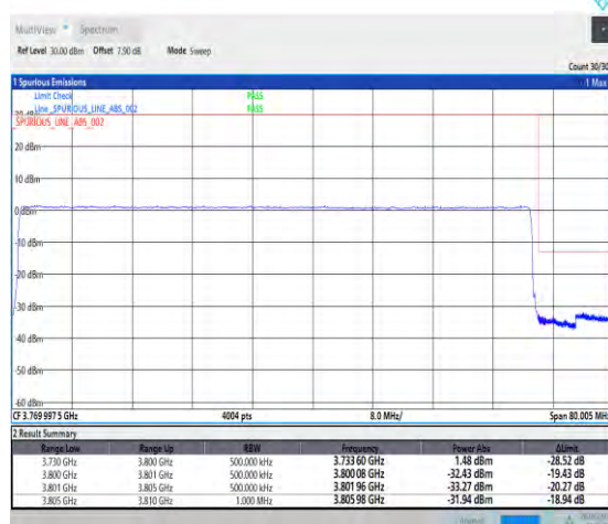
1-N78-3700-3800-PC2-30-70-H-6-CP-QPSK-Outer_Full-189@0-Ant1-PASS-see graph
