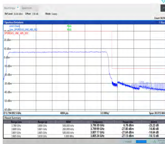
1-N78-3700-3800-PC2-30-20-H-6-CP-QPSK-Outer_Full-51@0-Ant1-PASS-see graph
