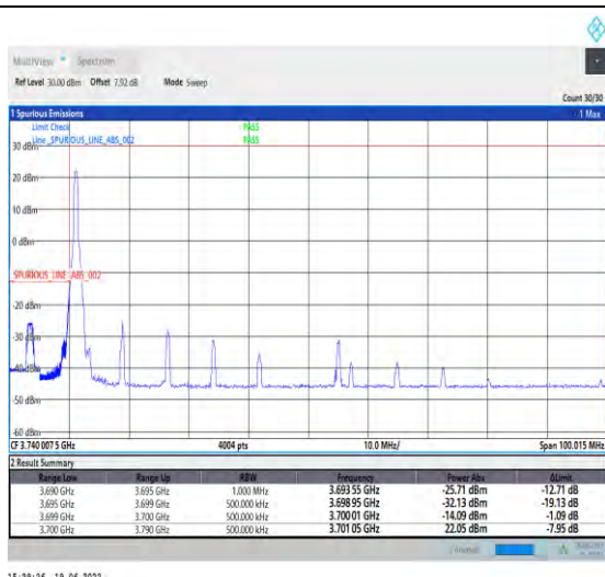
1-N78-3700-3800-PC2-30-90-L-1-DFT-PI2BPSK-Edge_1RB_Left-1@0-Ant1-PASS-see graph
