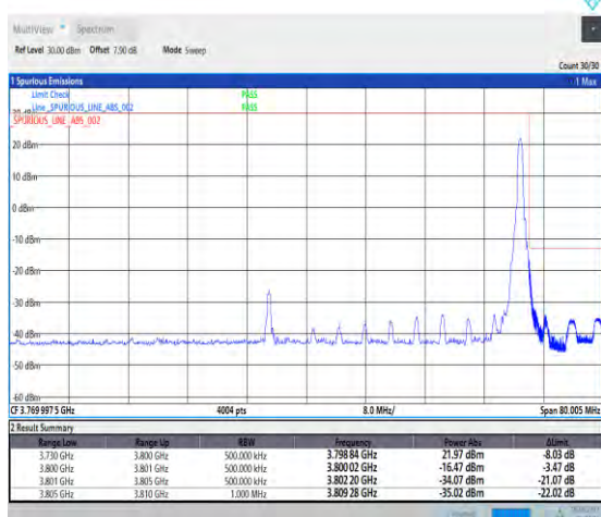
1-N78-3700-3800-PC2-30-70-H-5-CP-QPSK-Edge_1RB_Right-1@188-Ant1-PASS-see graph
