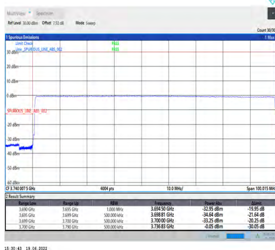
1-N78-3700-3800-PC2-30-90-L-6-CP-QPSK-Outer_Full-245@0-Ant1-PASS-see graph
