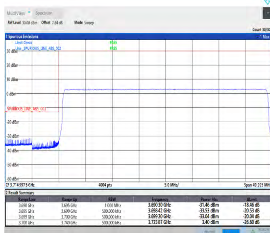
1-N78-3700-3800-PC2-30-40-L-6-CP-QPSK-Outer_Full-106@0-Ant1-PASS-see graph
