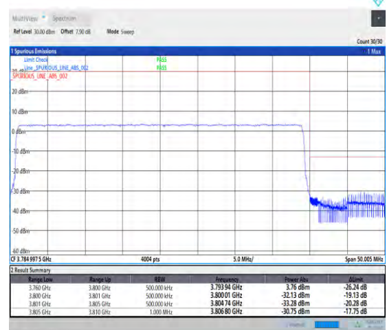
1-N78-3700-3800-PC2-30-40-H-6-CP-QPSK-Outer_Full-106@0-Ant1-PASS-see graph
