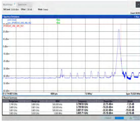
1-N78-3700-3800-PC2-30-60-H-2-DFT-PI2BPSK-Edge_1RB_Right-1@161-Ant1-PASS-see graph
