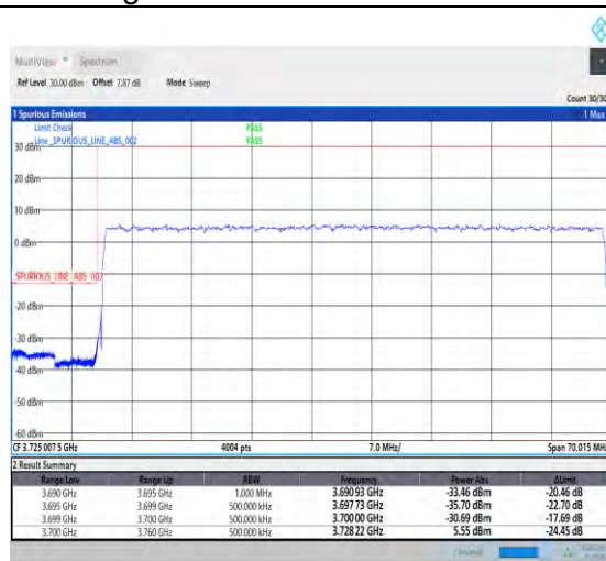
1-N78-3700-3800-PC2-30-60-L-3-DFT-PI2BPSK-Outer_Full-162@0-Ant1-PASS-see graph
