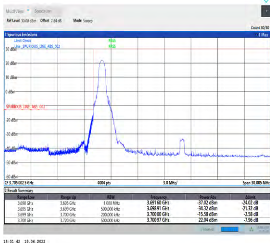
1-N78-3700-3800-PC2-30-20-L-1-DFT-PI2BPSK-Edge_1RB_Left-1@0-Ant1-PASS-see graph
