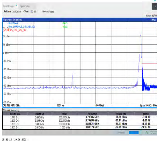
1-N78-3700-3800-PC2-30-90-H-5-CP-QPSK-Edge_1RB_Right-1@244-Ant1-PASS-see graph
