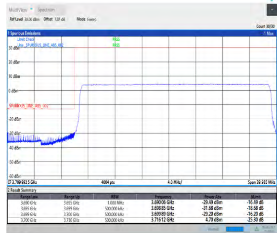
1-N78-3700-3800-PC2-30-30-L-6-CP-QPSK-Outer_Full-78@0-Ant1-PASS-see graph
