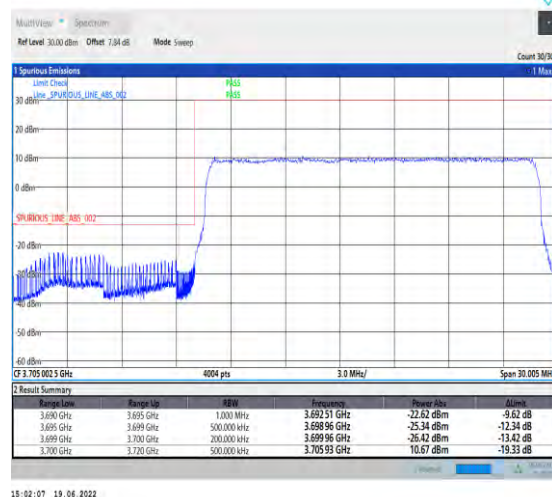
1-N78-3700-3800-PC2-30-20-L-3-DFT-PI2BPSK-Outer_Full-50@0-Ant1-PASS-see graph
