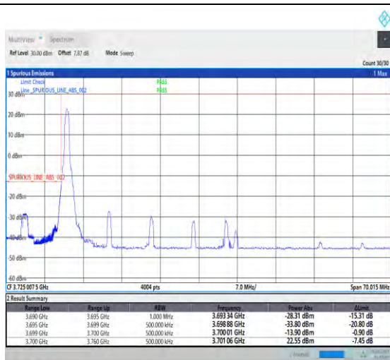
1-N78-3700-3800-PC2-30-60-L-1-DFT-PI2BPSK-Edge_1RB_Left-1@0-Ant1-PASS-see graph
