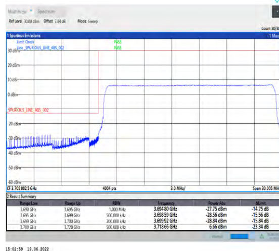
1-N78-3700-3800-PC2-30-20-L-6-CP-QPSK-Outer_Full-51@0-Ant1-PASS-see graph
