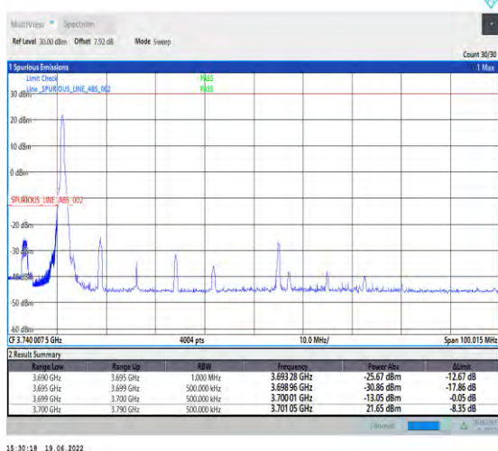
1-N78-3700-3800-PC2-30-90-L-4-CP-QPSK-Edge_1RB_Left-1@0-Ant1-PASS-see graph
