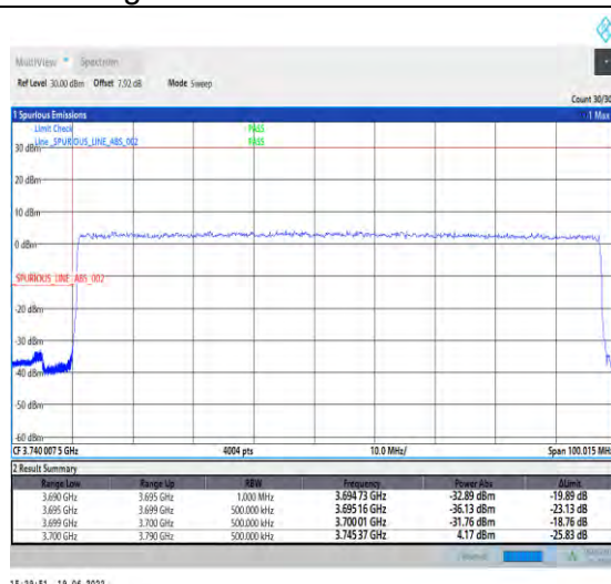
1-N78-3700-3800-PC2-30-90-L-3-DFT-PI2BPSK-Outer_Full-240@0-Ant1-PASS-see graph
