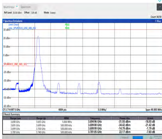
1-N78-3700-3800-PC2-30-40-L-1-DFT-PI2BPSK-Edge_1RB_Left-1@0-Ant1-PASS-see graph
