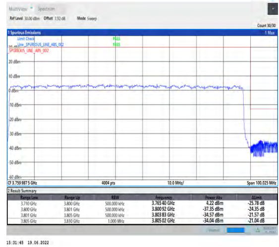
1-N78-3700-3800-PC2-30-90-H-3-DFT-PI2BPSK-Outer_Full-240@0-Ant1-PASS-see graph
