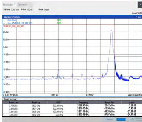
1-N78-3700-3800-PC2-30-40-H-2-DFT-PI2BPSK-Edge_1RB_Right-1@105-Ant1-PASS-see graph
