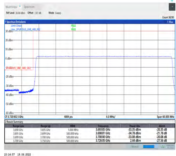
1-N78-3700-3800-PC2-30-50-L-6-CP-QPSK-Outer_Full-133@0-Ant1-PASS-see graph
