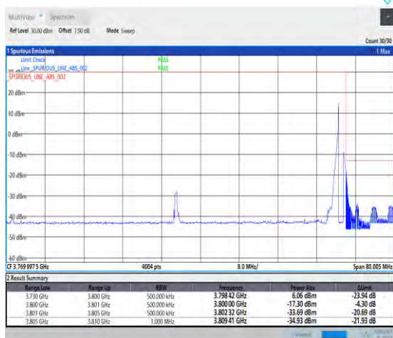
1-N78-3700-3800-PC2-30-70-H-2-DFT-PI2BPSK-Edge_1RB_Right-1@188-Ant1-PASS-see graph
