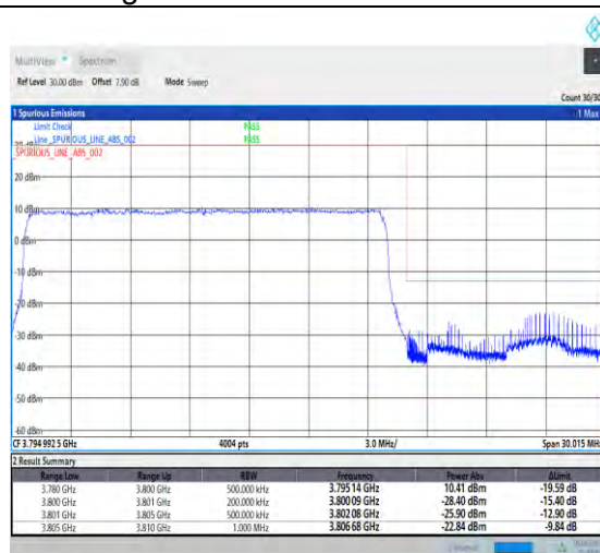
1-N78-3700-3800-PC2-30-20-H-3-DFT-PI2BPSK-Outer_Full-50@0-Ant1-PASS-see graph
