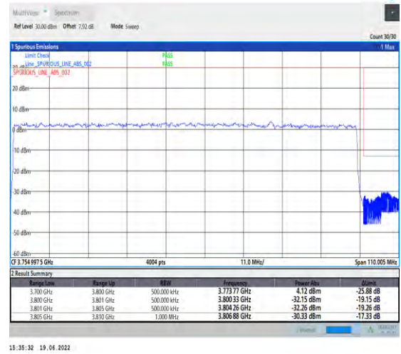
1-N78-3700-3800-PC2-30-100-H-3-DFT-PI2BPSK-Outer_Full-270@0-Ant1-PASS-see graph
