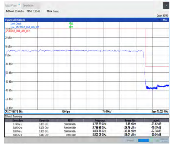
1-N78-3700-3800-PC2-30-60-H-3-DFT-PI2BPSK-Outer_Full-162@0-Ant1-PASS-see graph
