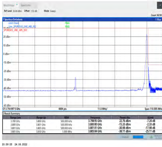
1-N78-3700-3800-PC2-30-100-H-2-DFT-PI2BPSK-Edge_1RB_Right-1@272-Ant1-PASS-see graph
