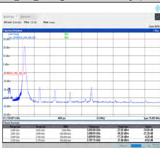
1-N78-3700-3800-PC2-30-70-L-1-DFT-PI2BPSK-Edge_1RB_Left-1@0-Ant1-PASS-see graph
