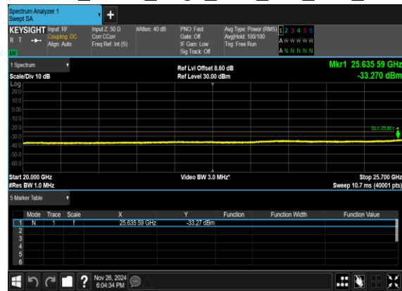
N7(25M)_DFT-s- OFDM_BPSK_Edge_1RB_Left_Low_CH
