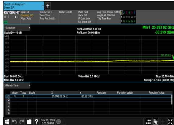
N7(25M)_DFT-s- OFDM_QPSK_Edge_1RB_Left_Low_CH
