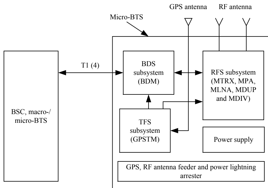
Fig. 1.1-1 Structure of ZXCBS M800T Micro-BTS
