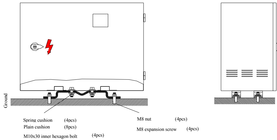
Fig. 13.3-3 Frontal and Lateral Faces of the UPS's Floor-type Installation
