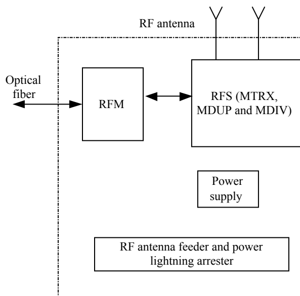
Fig. 1.1-2 Structure of Remote Stations
