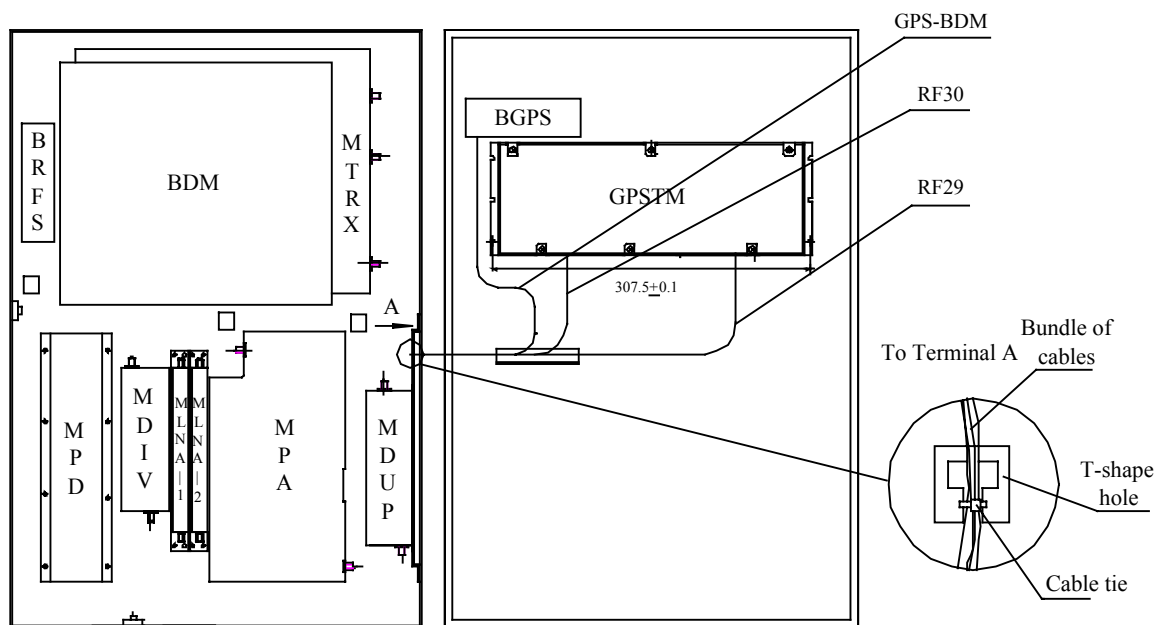
Fig. 10.3-1 Schematic Diagram of Bundling Internal Cables (1)
