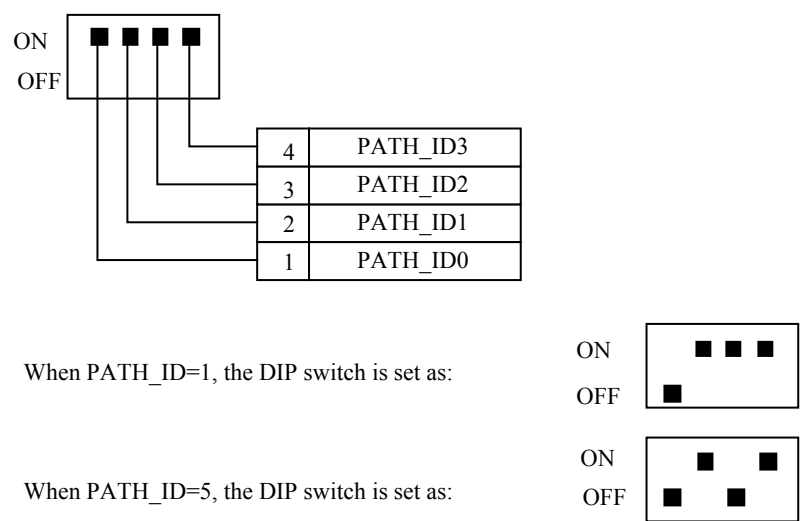
Fig. 12.1-1 Setting of S1
