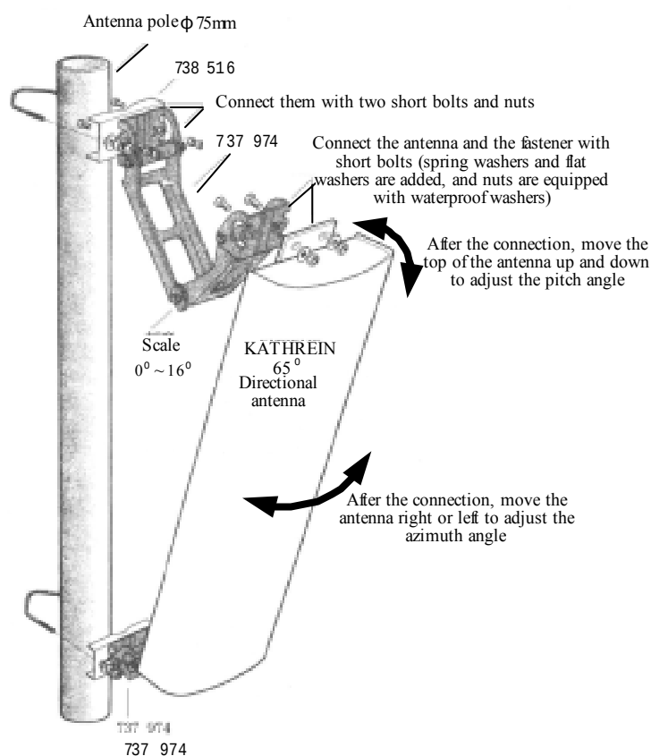
Fig. 8.4-1 Installation of the KATHREIN Antenna
