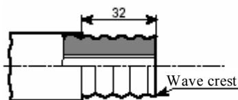
Fig. 8.6-4 Schematic Diagram of Correct Cutting Size
