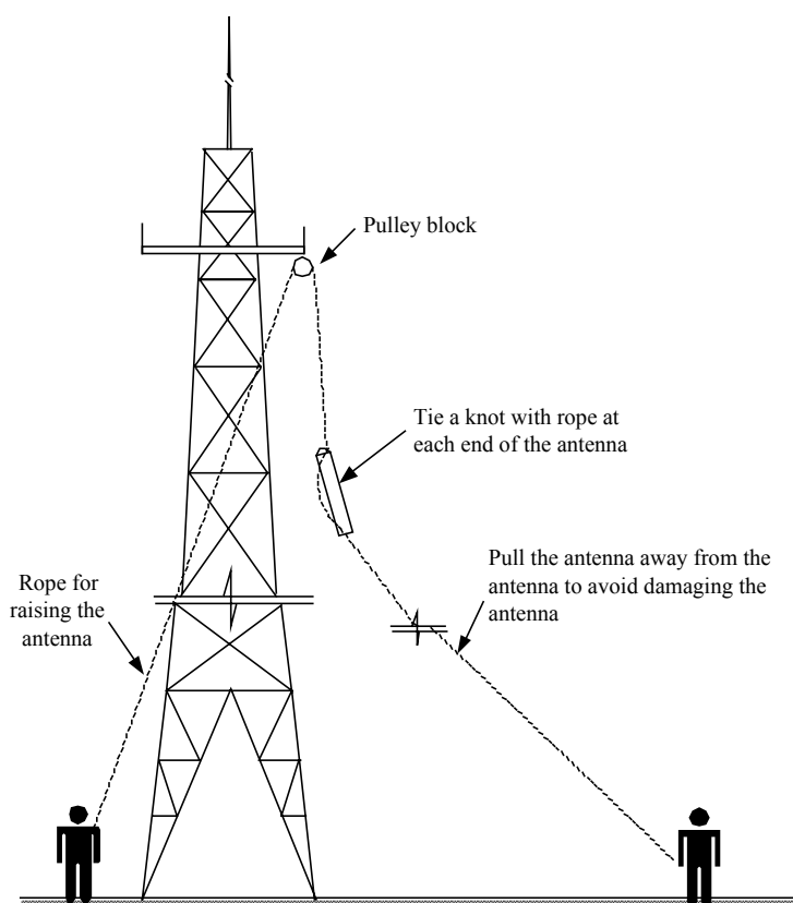
Fig. 8.4-2 Schematic Diagram of Raising the Antenna to the Tower Top
