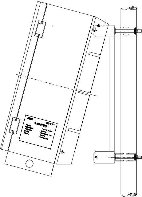
Fig. 4.2-2 Schematic Diagram of Fastening the Cabinet onto the Pole (step 2)
