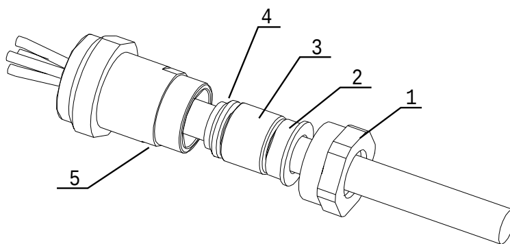
Fig. 5.3-2 Assembling a Power Cable Connector (step 2)
