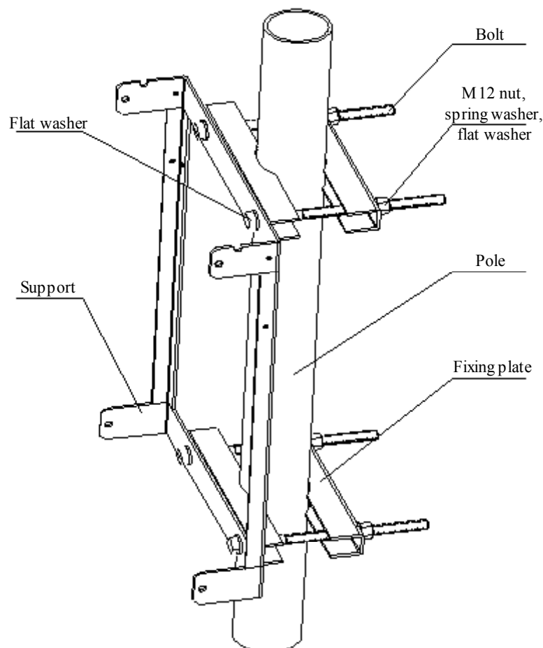
Fig. 4.2-1 Schematic Diagram of Fastening the Cabinet onto the Pole (step 1)
