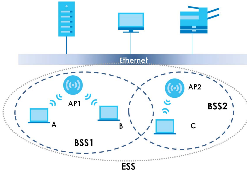
Figure 55 Infrastructure WLAN
