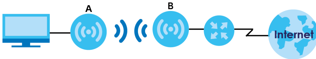
Figure 17 Wireless Client Mode
