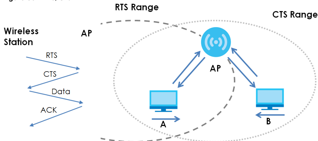
Figure 56 RTS/CTS
