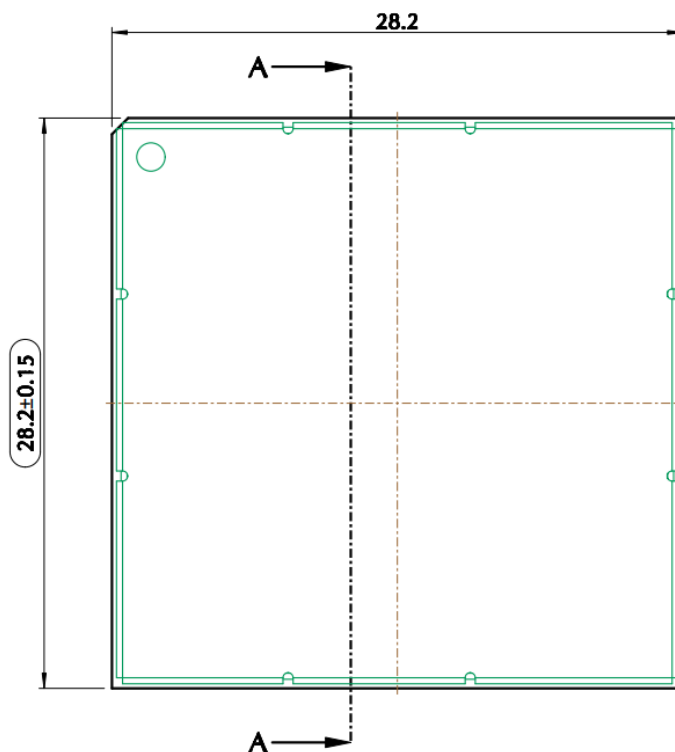
Figure 27: LE910Cx-APX Mechanical Dimensions (Top view) with frame and cover shield design
