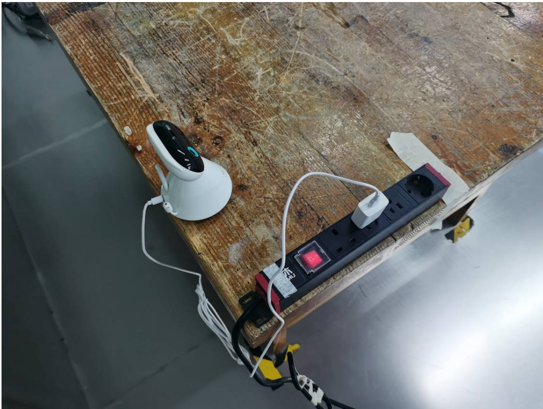
Conducted Emissions Side View (UT-681A-5200ZCY)
