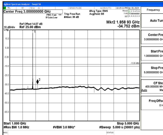
Band4-1.4MHz-16QAM-19957-1-0-Low-1000-5000--34.75-PASS
