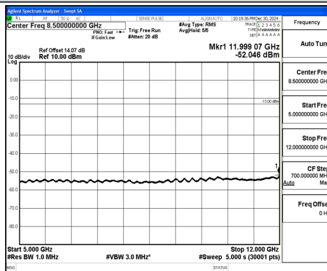
Band4-1.4MHz-16QAM-20175-1-0-Low-5000-12000--52.05-PASS
