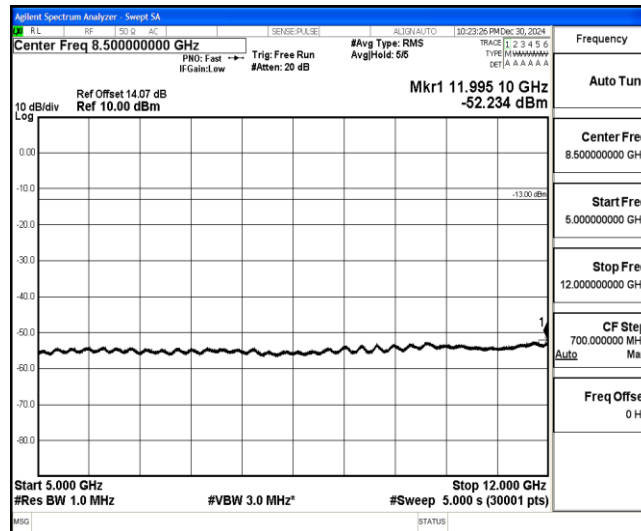
Band4-1.4MHz-16QAM-20393-1-0-High-5000-12000--52.23-PASS
