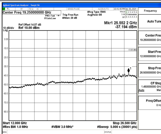
Band4-3MHz-16QAM-20175-1-0-Low-12000-26500--37.19-PASS
