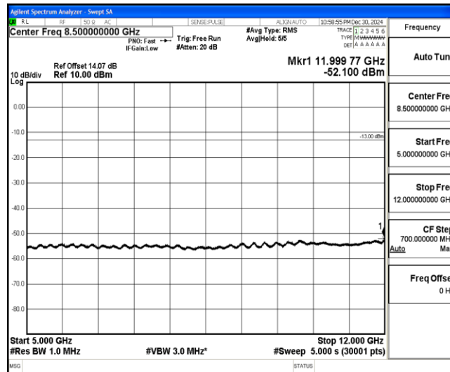
Band4-5MHz-QPSK-19975-1-0-Low-5000-12000--52.1-PASS
