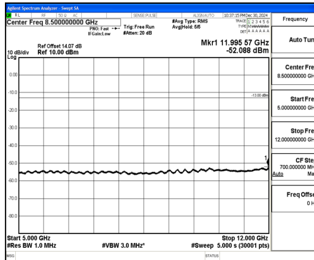
Band4-3MHz-16QAM-19965-1-0-Low-5000-12000--52.09-PASS
