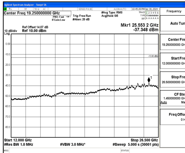
Band4-3MHz-16QAM-20385-1-0-High-12000-26500--37.35-PASS
