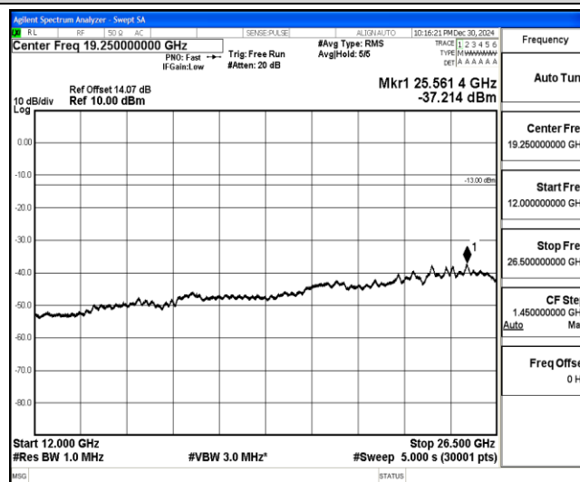
Band4-1.4MHz-16QAM-19957-1-0-Low-12000-26500--37.21-PASS
