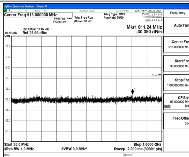
Band4-5MHz-QPSK-19975-1-0-Low-30-1000--30.35-PASS
