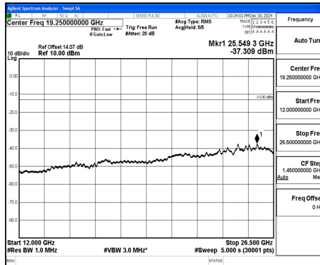
Band4-1.4MHz-16QAM-20393-1-0-High-12000-26500--37.31-PASS
