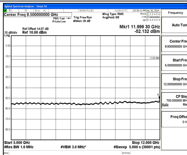
Band4-3MHz-QPSK-20175-1-0-Low-5000-12000--52.13-PASS
