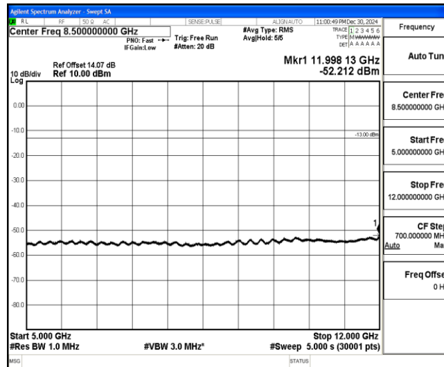
Band4-5MHz-16QAM-19975-1-0-Low-5000-12000--52.21-PASS
