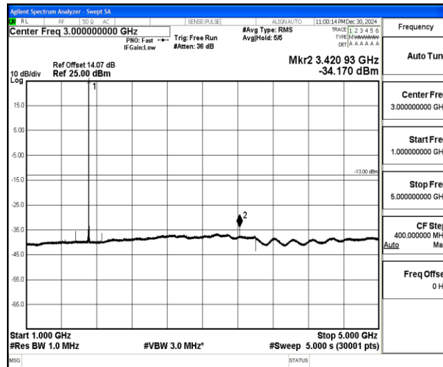
Band4-5MHz-16QAM-19975-1-0-Low-1000-5000--34.17-PASS
