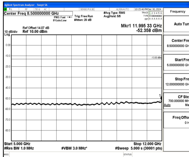
Band4-1.4MHz-16QAM-19957-1-0-Low-5000-12000--52.36-PASS
