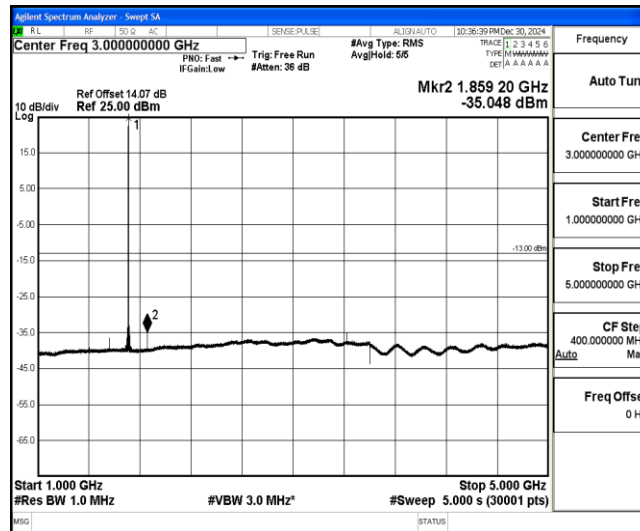
Band4-3MHz-16QAM-19965-1-0-Low-1000-5000--35.05-PASS
