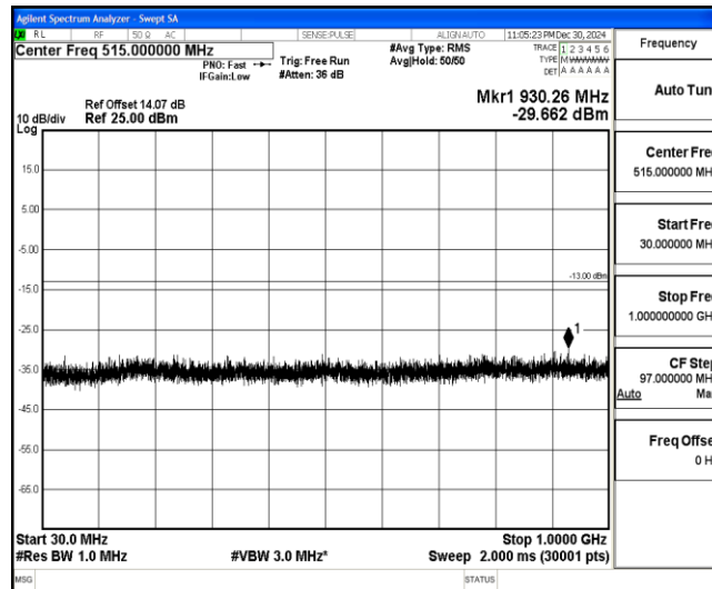
Band4-5MHz-QPSK-20375-1-0-High-30-1000--29.66-PASS
