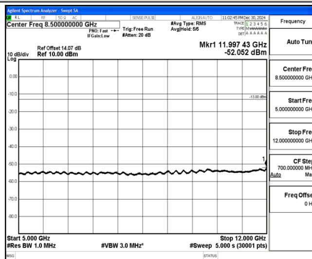
Band4-5MHz-QPSK-20175-1-0-Low-5000-12000--52.05-PASS
