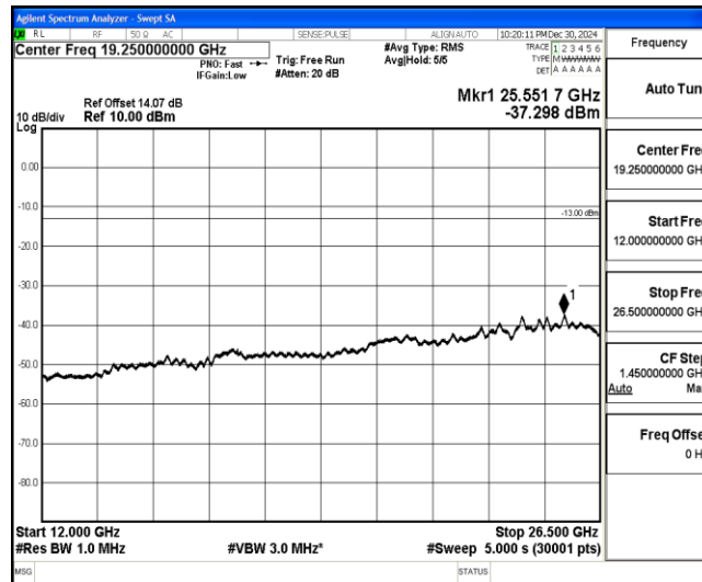
Band4-1.4MHz-16QAM-20175-1-0-Low-12000-26500--37.3-PASS
