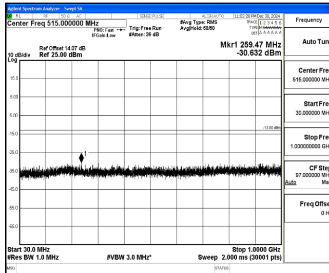
Band4-5MHz-16QAM-20175-1-0-Low-30-1000--30.63-PASS
