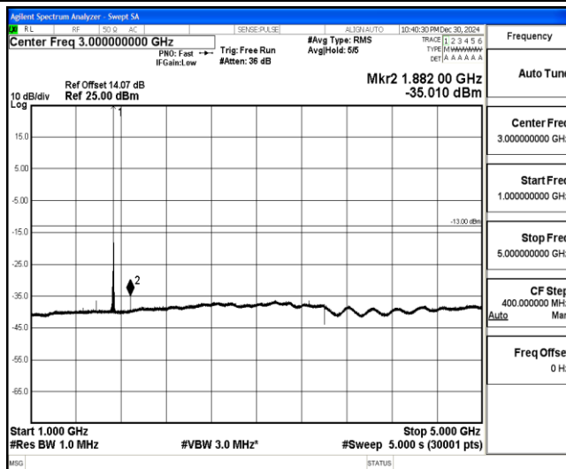
Band4-3MHz-16QAM-20175-1-0-Low-1000-5000--35.01-PASS
