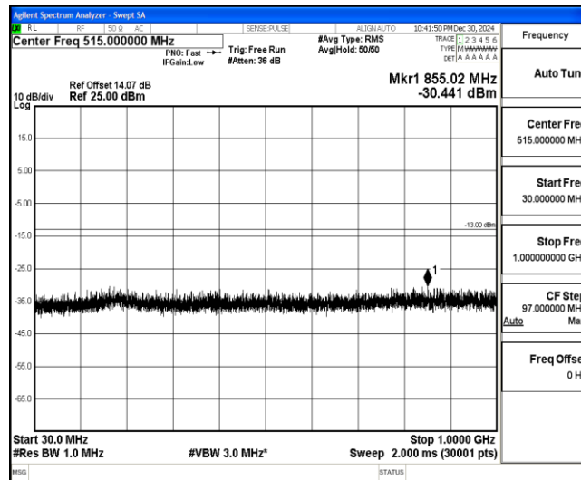
Band4-3MHz-QPSK-20385-1-0-High-30-1000--30.44-PASS
