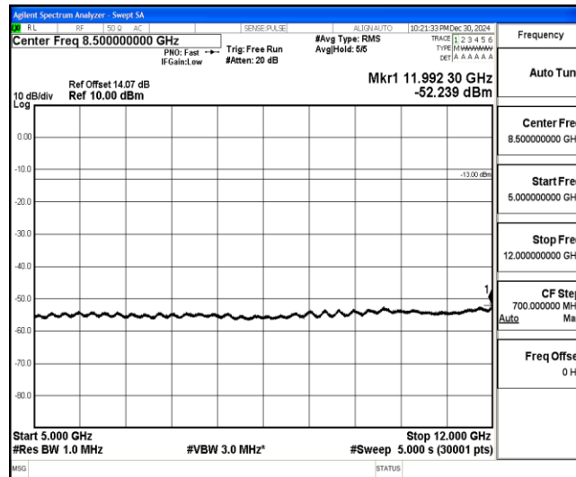
Band4-1.4MHz-QPSK-20393-1-0-High-5000-12000--52.24-PASS
