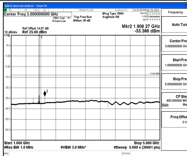
Band4-1.4MHz-QPSK-20393-1-0-High-1000-5000--33.39-PASS
