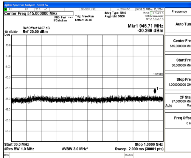
Band4-3MHz-QPSK-20175-1-0-Low-30-1000--30.27-PASS
