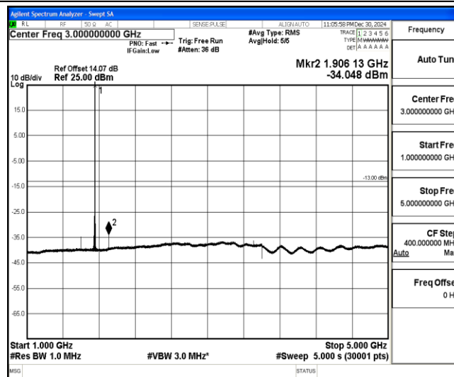
Band4-5MHz-QPSK-20375-1-0-High-1000-5000--34.05-PASS
