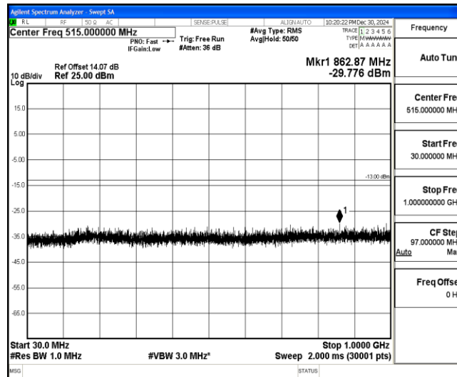
Band4-1.4MHz-QPSK-20393-1-0-High-30-1000--29.78-PASS
