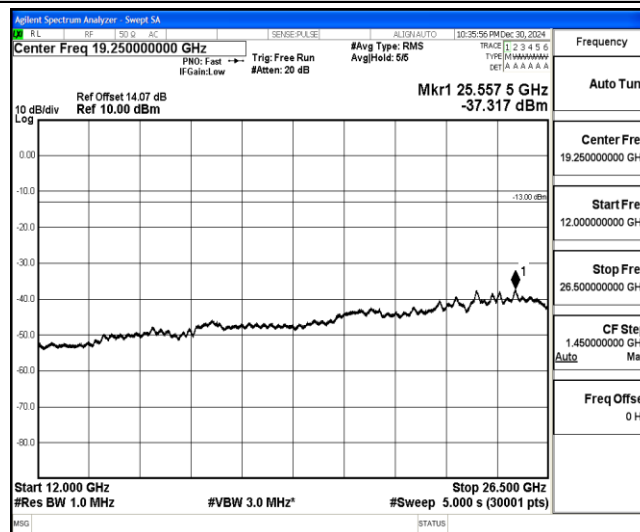
Band4-3MHz-QPSK-19965-1-0-Low-12000-26500--37.32-PASS
