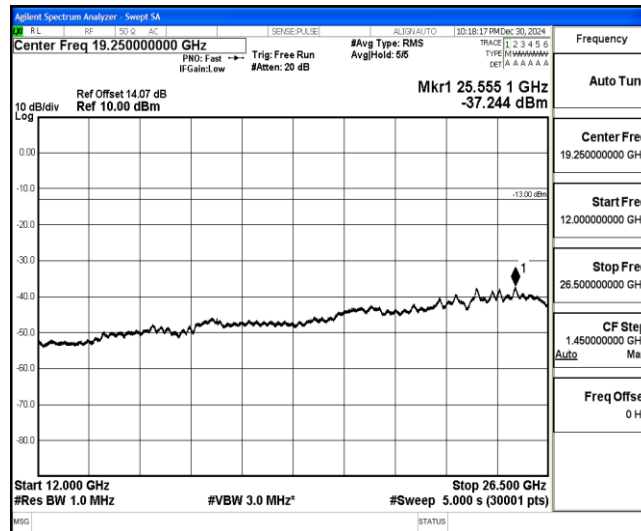
Band4-1.4MHz-QPSK-20175-1-0-Low-12000-26500--37.24-PASS
