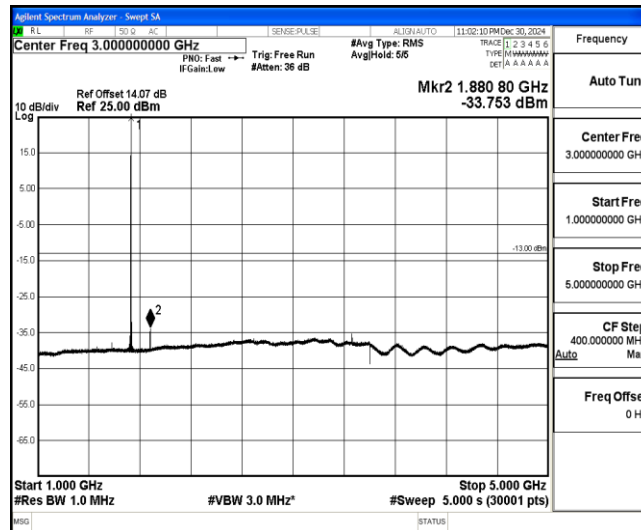
Band4-5MHz-QPSK-20175-1-0-Low-1000-5000--33.75-PASS
