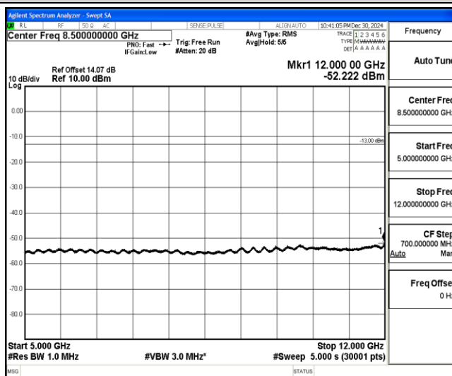
Band4-3MHz-16QAM-20175-1-0-Low-5000-12000--52.22-PASS
