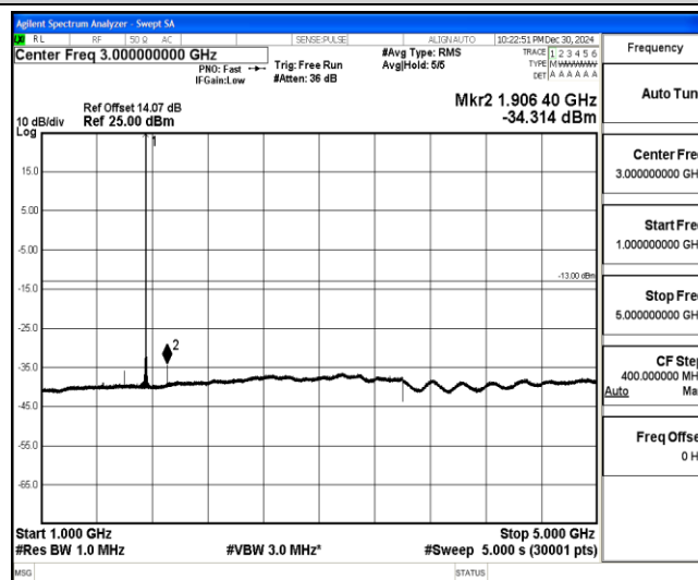
Band4-1.4MHz-16QAM-20393-1-0-High-1000-5000--34.31-PASS
