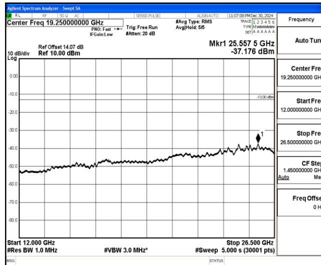
Band4-5MHz-QPSK-20375-1-0-High-12000-26500--37.18-PASS
