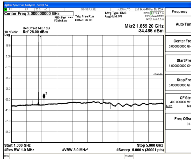
Band4-3MHz-QPSK-19965-1-0-Low-1000-5000--34.47-PASS
