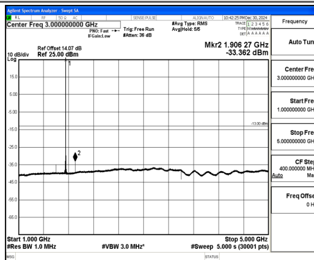
Band4-3MHz-QPSK-20385-1-0-High-1000-5000--33.36-PASS
