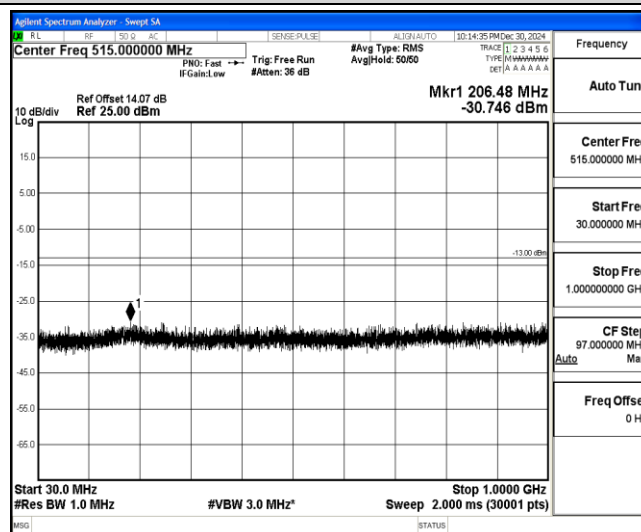
Band4-1.4MHz-16QAM-19957-1-0-Low-30-1000--30.75-PASS
