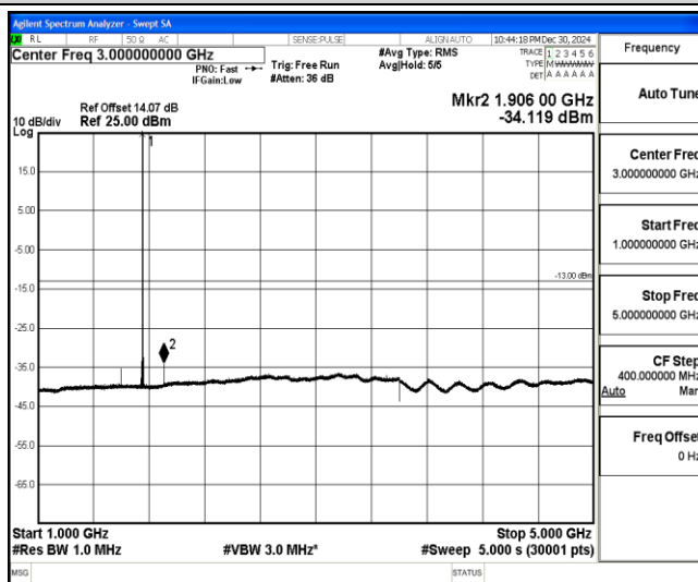
Band4-3MHz-16QAM-20385-1-0-High-1000-5000--34.12-PASS
