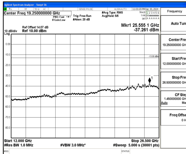
Band4-5MHz-QPSK-20175-1-0-Low-12000-26500--37.26-PASS
