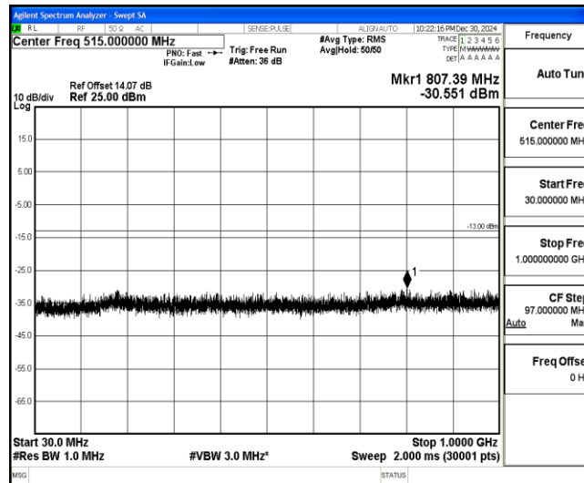
Band4-1.4MHz-16QAM-20393-1-0-High-30-1000--30.55-PASS
