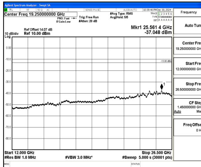
Band4-3MHz-QPSK-20175-1-0-Low-12000-26500--37.05-PASS
