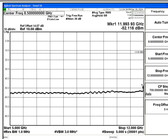
Band4-5MHz-16QAM-20175-1-0-Low-5000-12000--52.12-PASS
