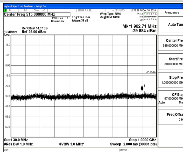
Band4-5MHz-16QAM-19975-1-0-Low-30-1000--29.88-PASS
