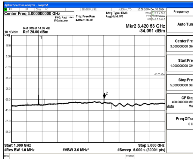
Band4-5MHz-QPSK-19975-1-0-Low-1000-5000--34.09-PASS
