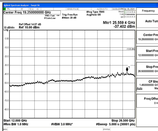
Band4-5MHz-16QAM-19975-1-0-Low-12000-26500--37.4-PASS
