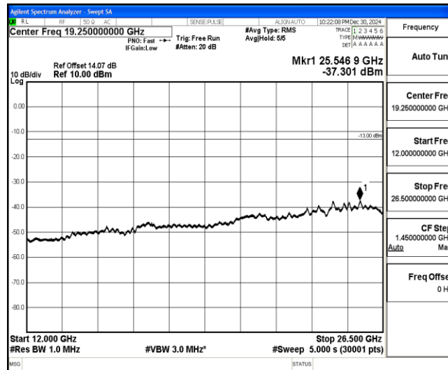
Band4-1.4MHz-QPSK-20393-1-0-High-12000-26500--37.3-PASS
