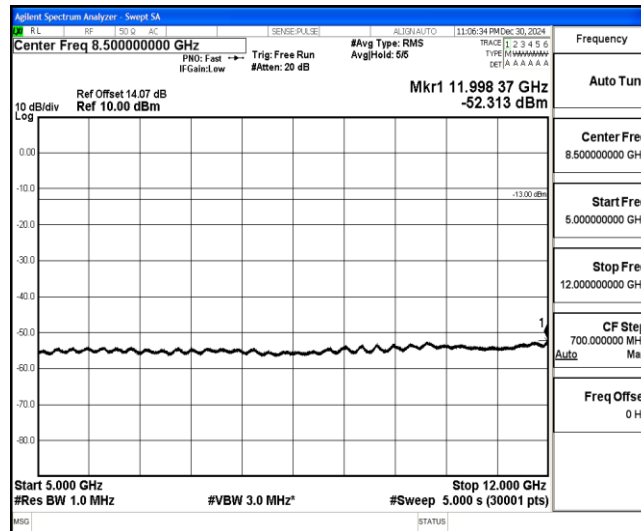
Band4-5MHz-QPSK-20375-1-0-High-5000-12000--52.31-PASS
