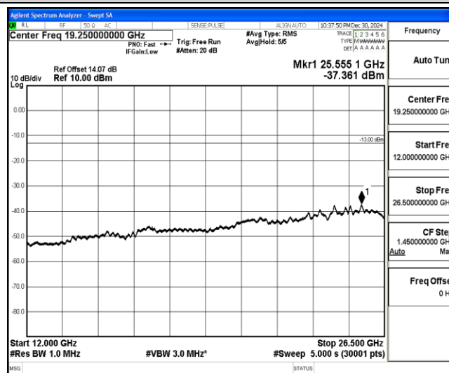
Band4-3MHz-16QAM-19965-1-0-Low-12000-26500--37.36-PASS
