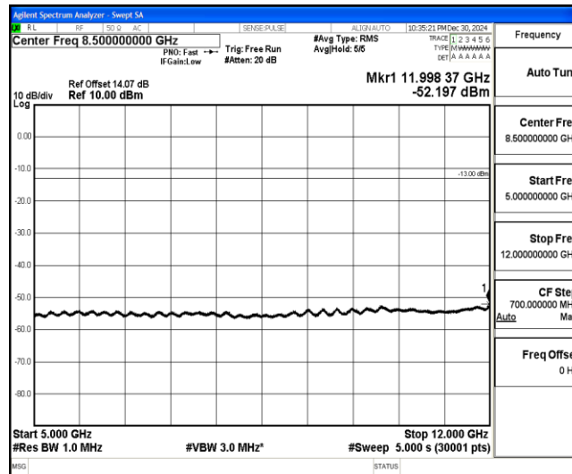
Band4-3MHz-QPSK-19965-1-0-Low-5000-12000--52.2-PASS
