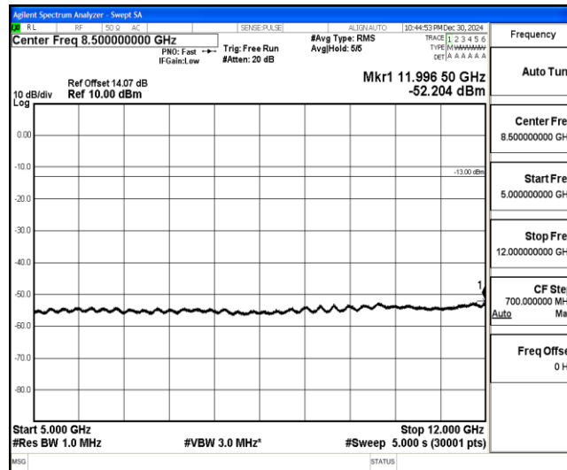
Band4-3MHz-16QAM-20385-1-0-High-5000-12000--52.2-PASS
