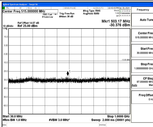
Band4-3MHz-16QAM-20385-1-0-High-30-1000--30.38-PASS
