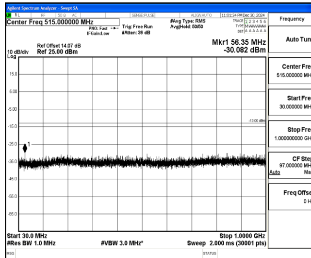
Band4-5MHz-QPSK-20175-1-0-Low-30-1000--30.08-PASS
