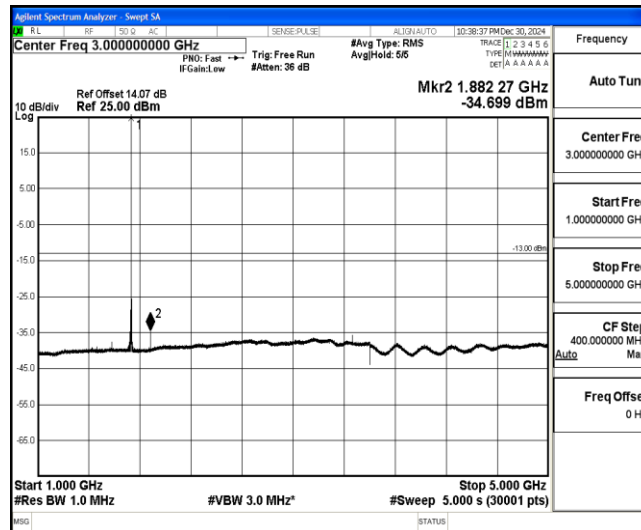
Band4-3MHz-QPSK-20175-1-0-Low-1000-5000--34.7-PASS
