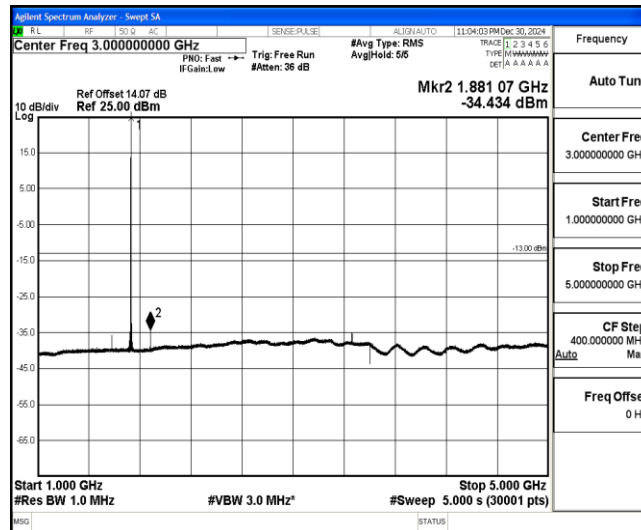
Band4-5MHz-16QAM-20175-1-0-Low-1000-5000--34.43-PASS
