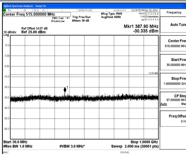
Band4-3MHz-16QAM-20175-1-0-Low-30-1000--30.34-PASS
