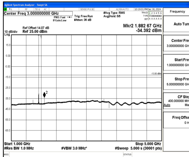
Band4-1.4MHz-16QAM-20175-1-0-Low-1000-5000--34.39-PASS
