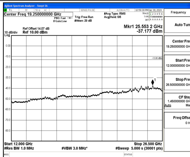
Band4-5MHz-QPSK-19975-1-0-Low-12000-26500--37.18-PASS
