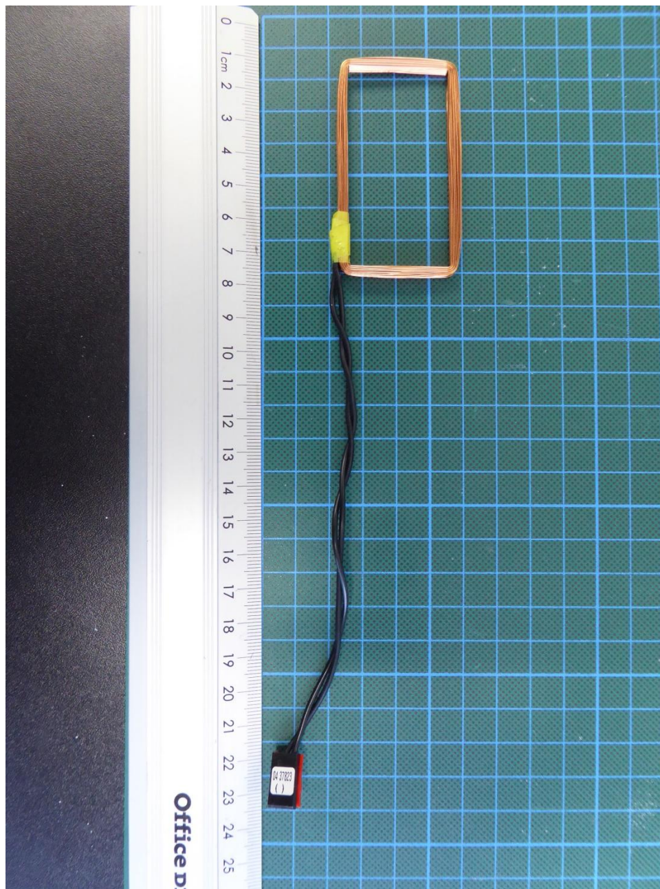
153615_14.JPG: Antenna 4 (0437823 0)
