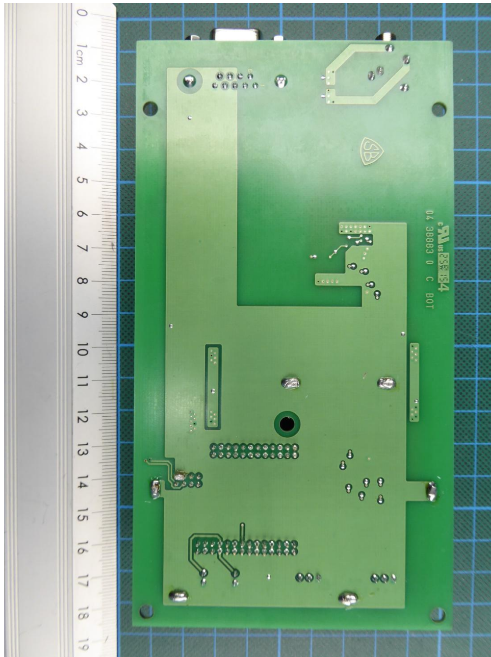
153615_7.JPG: EUT, bottom view
