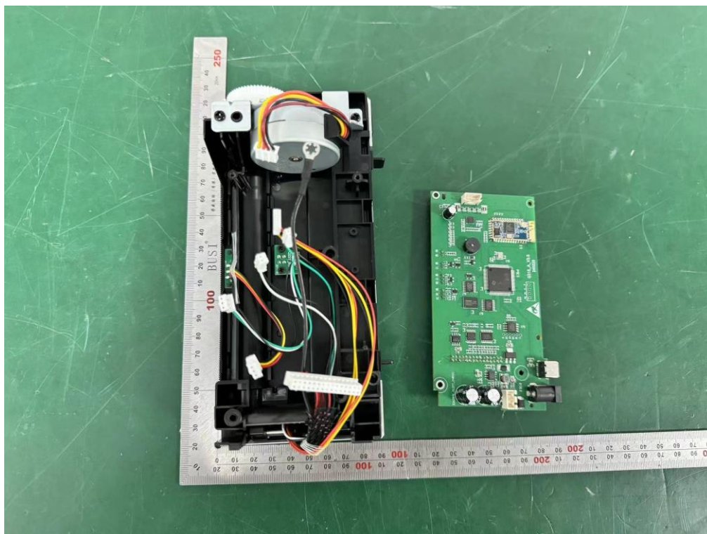
Internal photos M/N: PM-248-WF
