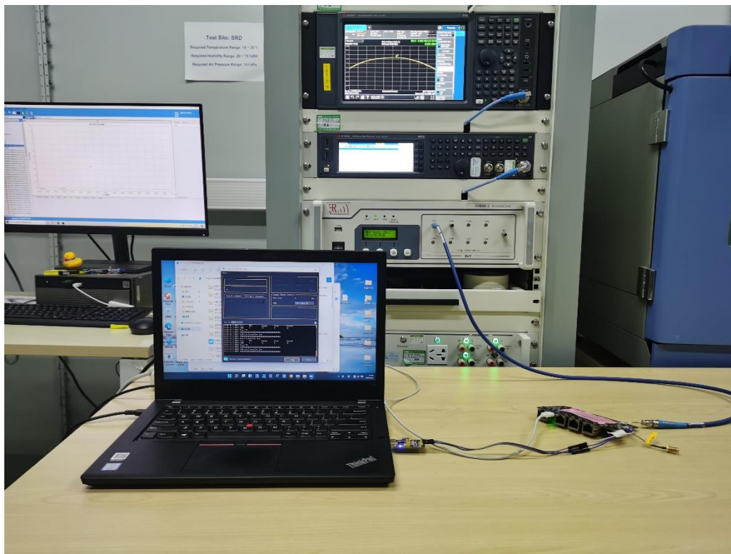
Photograph 3: Set-up photo for RF Conducted Singal test
